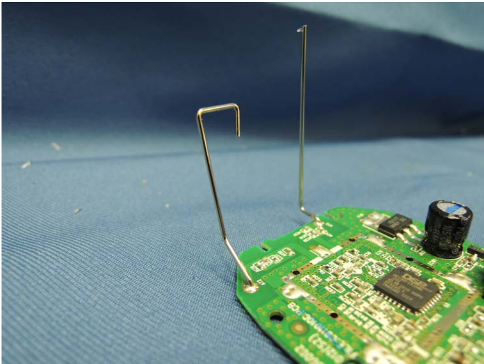
Base Unit Antenna AT2
