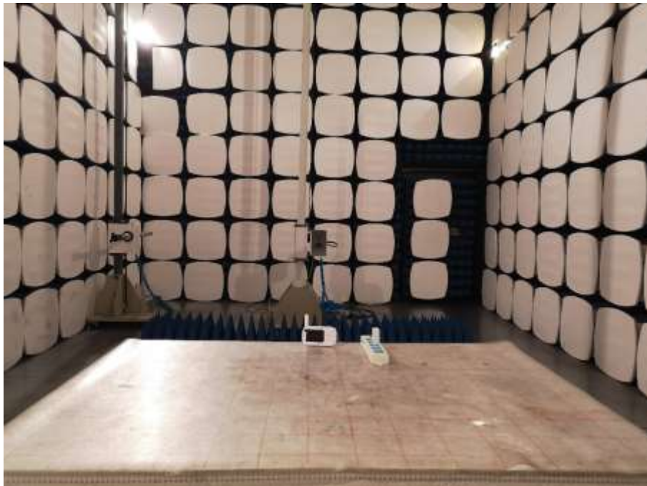
RADIATED EMISSION SET-UP PHOTOS, Above 1GHz
