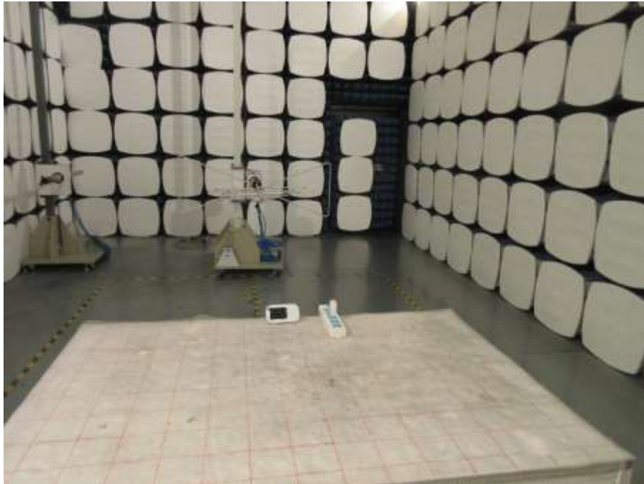
RADIATED EMISSION SET-UP PHOTOS, 30MHz ~ 1GHz
