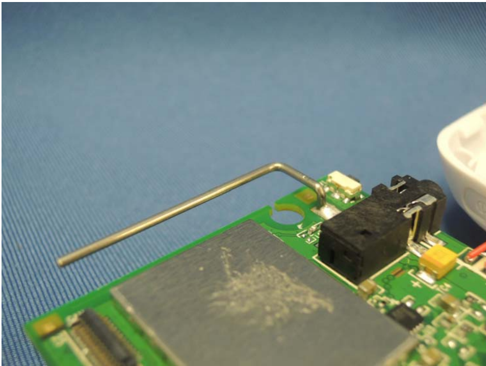
Dect Antenna
