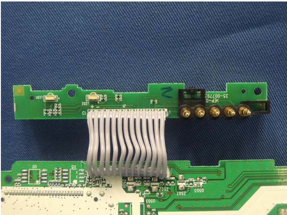
Charger Unit PCB display side (View 2)
