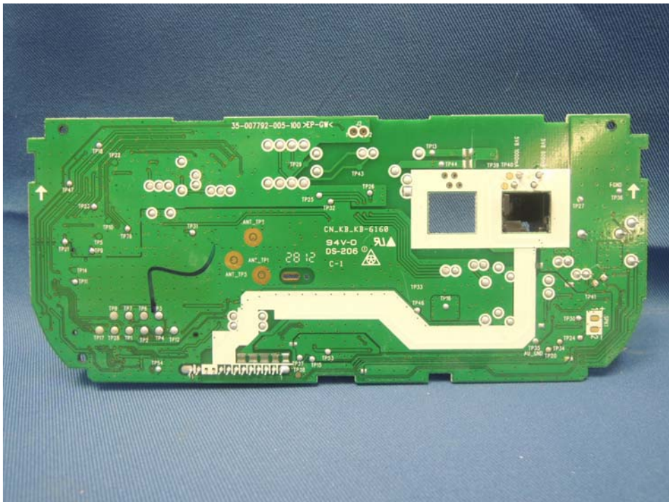
Charger Unit Main PCB comp side (View 3)
