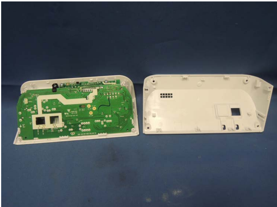
Charger Unit Main PCB comp side (View 1)
