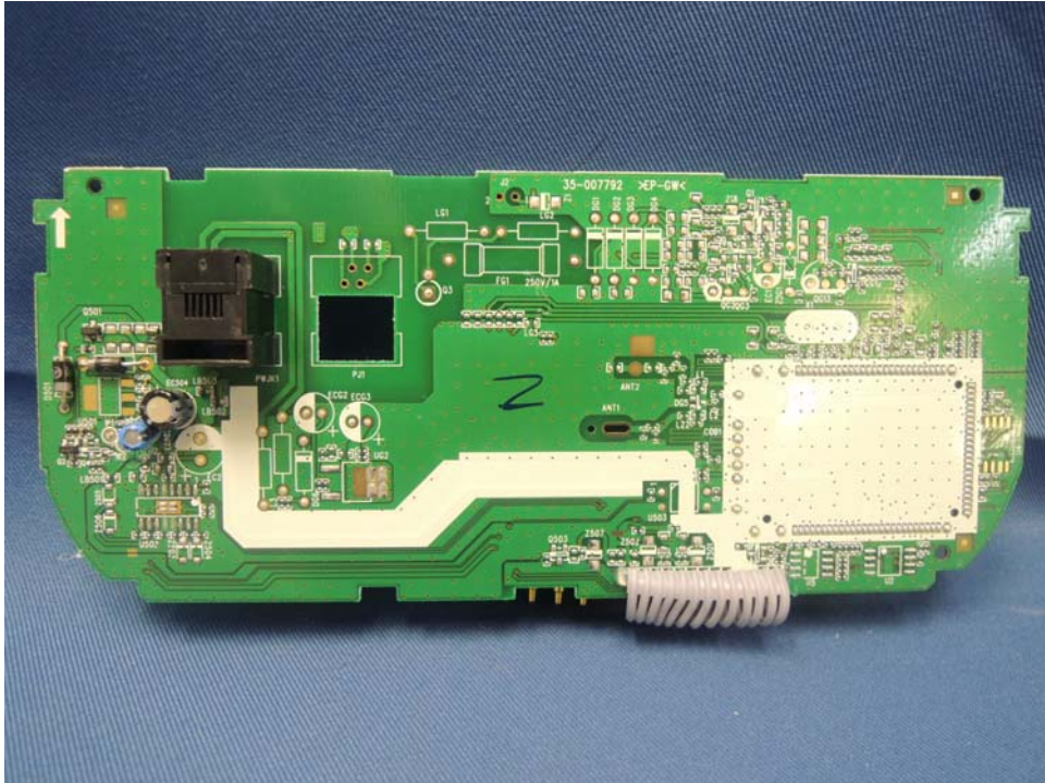
Charger Unit Main PCB comp side (View 2)
