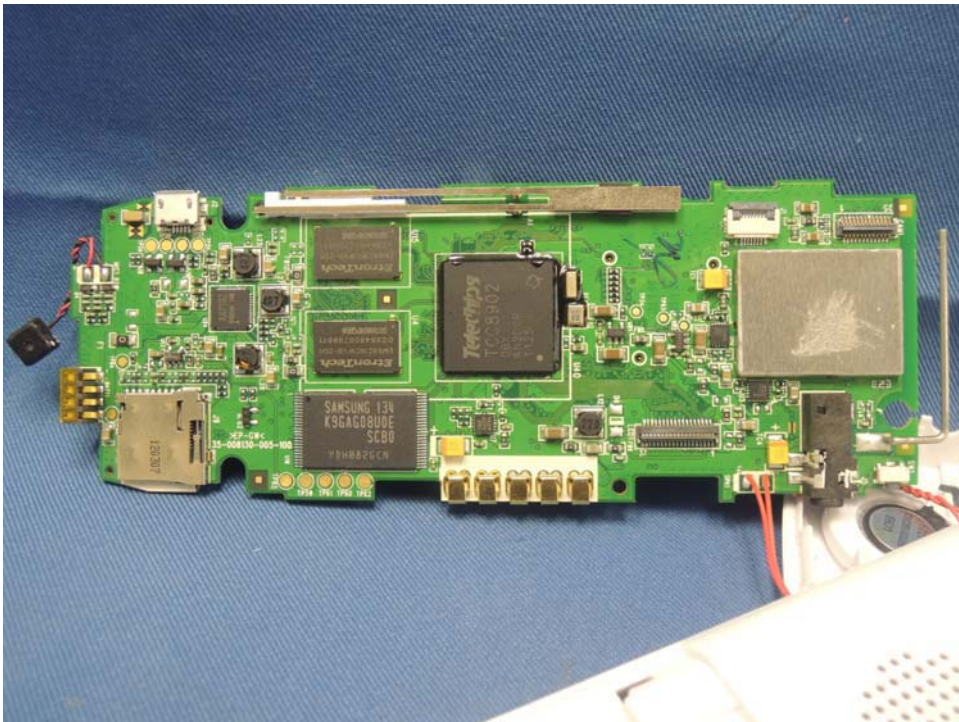
Handset Unit Main PCB comp side
