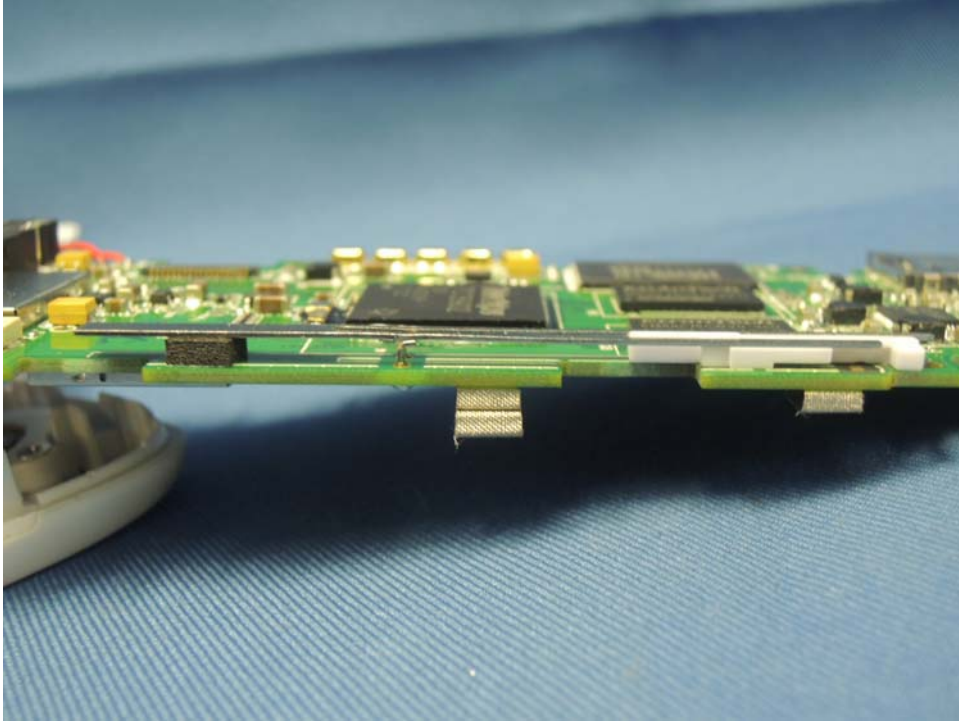
Wifi Antenna
