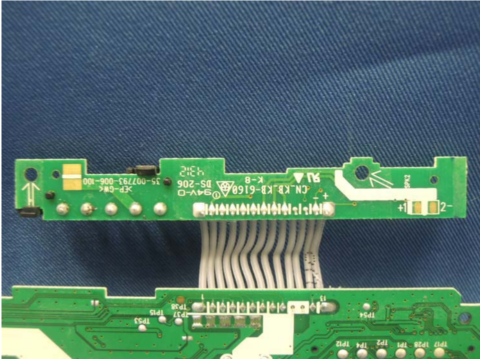
Charger Unit Main PCB display side (View 1)
