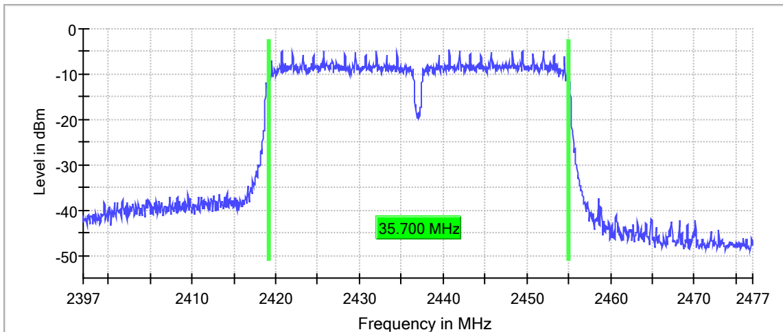
6 dB Bandwidth
