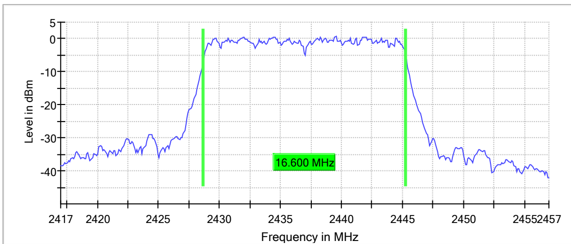
99 % Bandwidth
