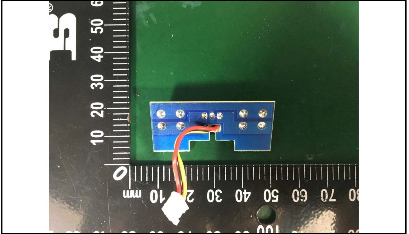
EUT Photo #7 PCB View
