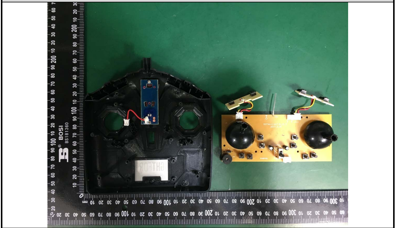
EUT Photo #3 Uncover View
