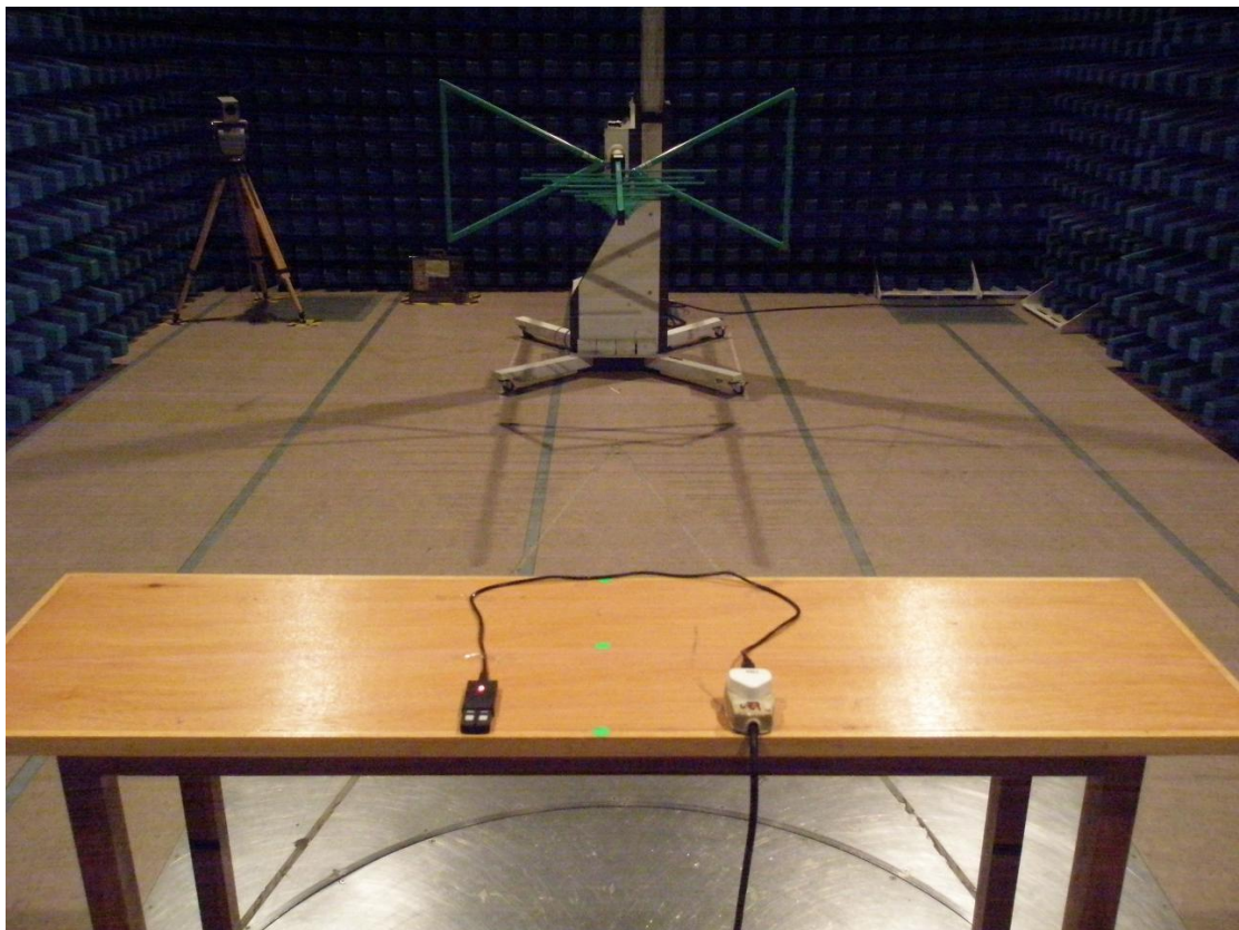
Rear view (Charging)
