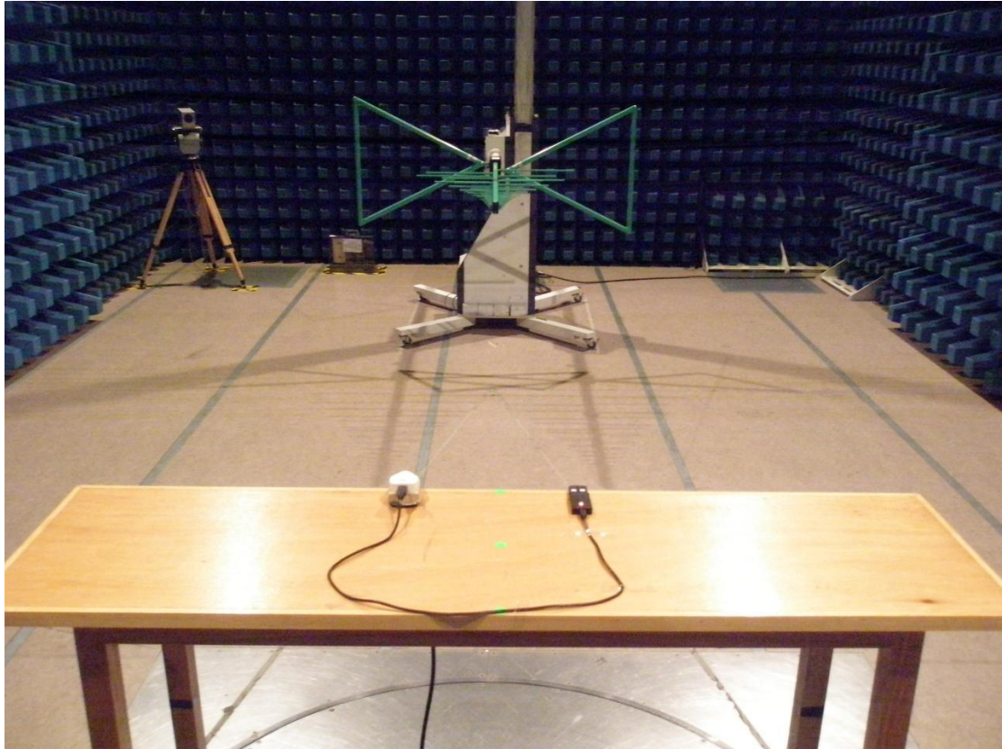
Front view (Charging)
