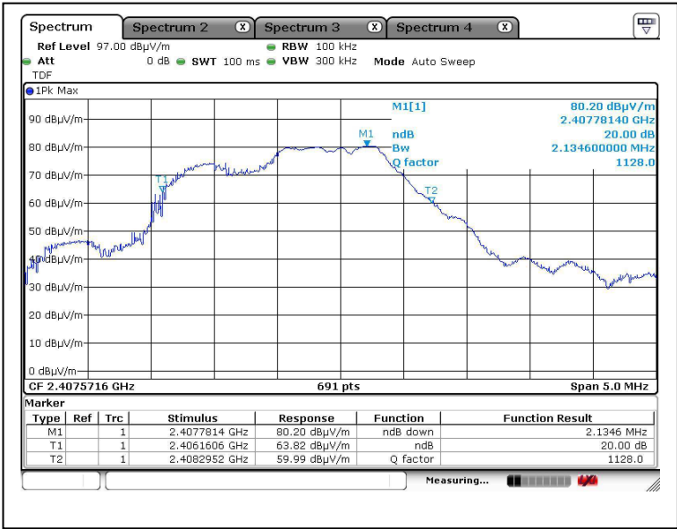
Bandwidth 1 (2407MHz)
