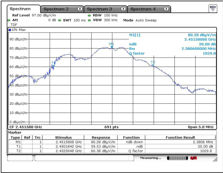
Bandwidth 2 (2452MHz)
