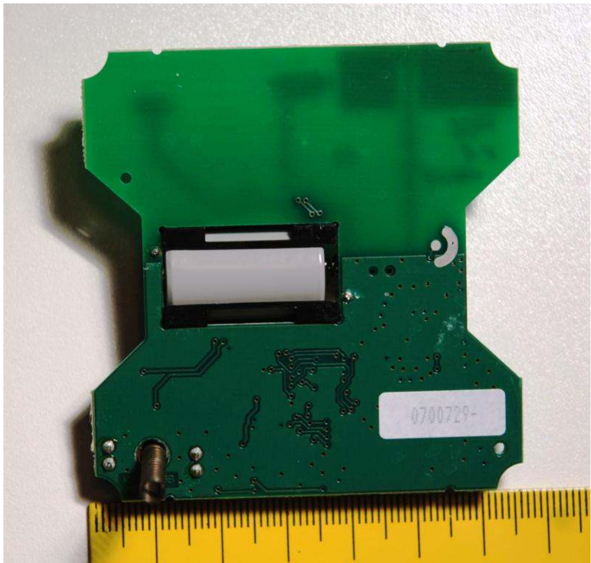
PCB rear view
