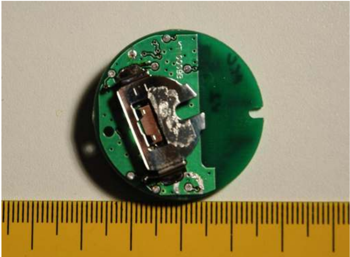
PCB – rear (battery) side
