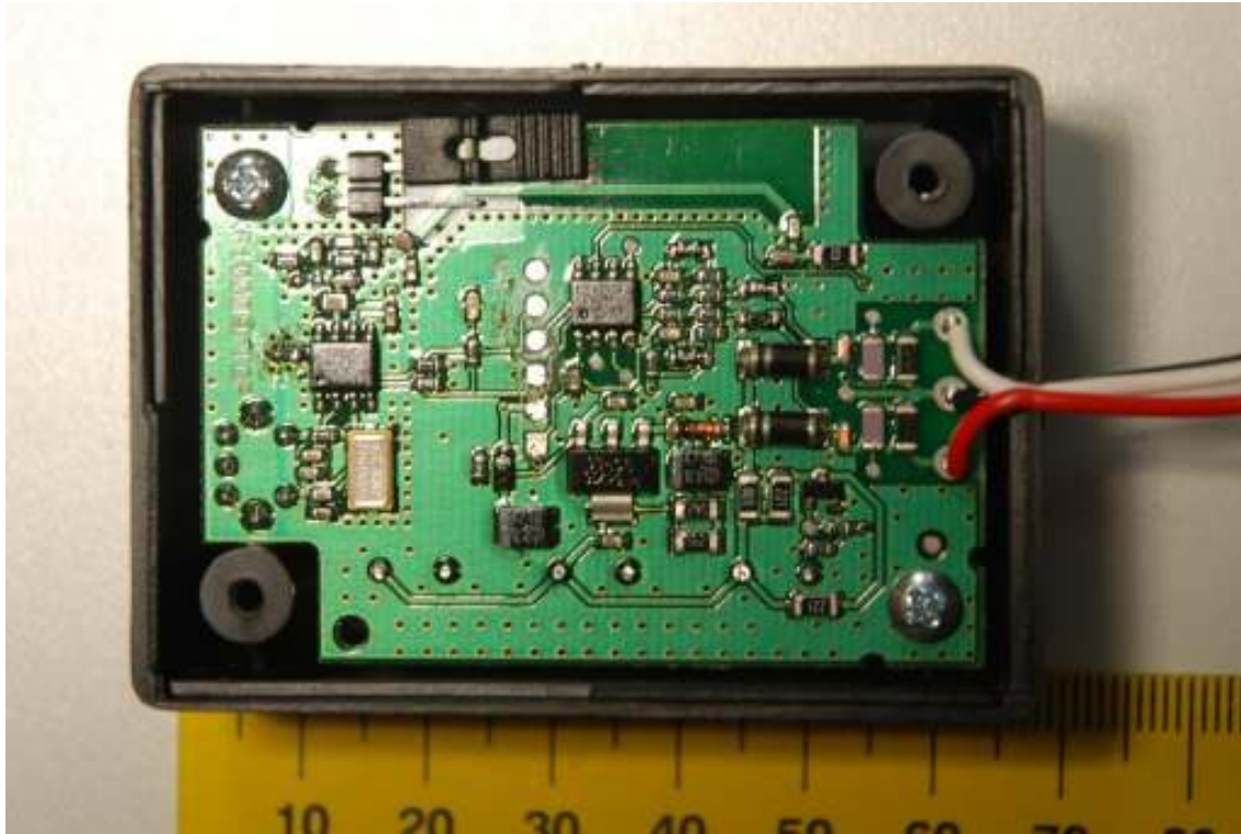
PCB in enclosure
