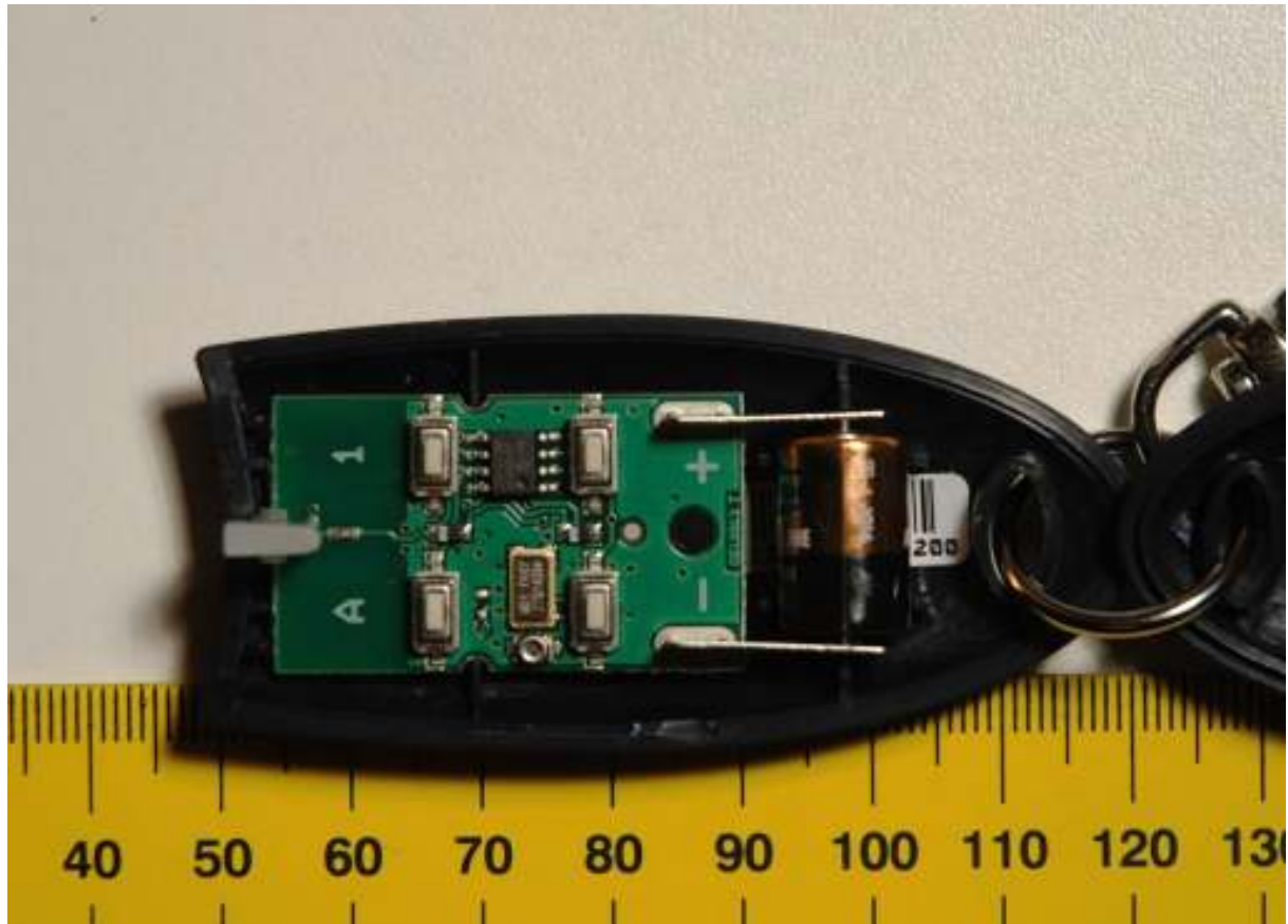
After removing the cover – front side PCB
