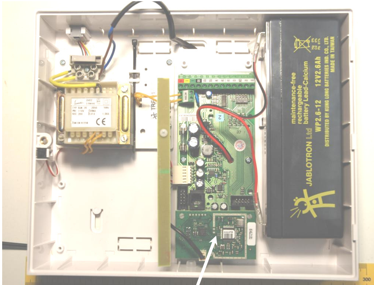
JA-82 R mount in JA-82K-US with antenna
