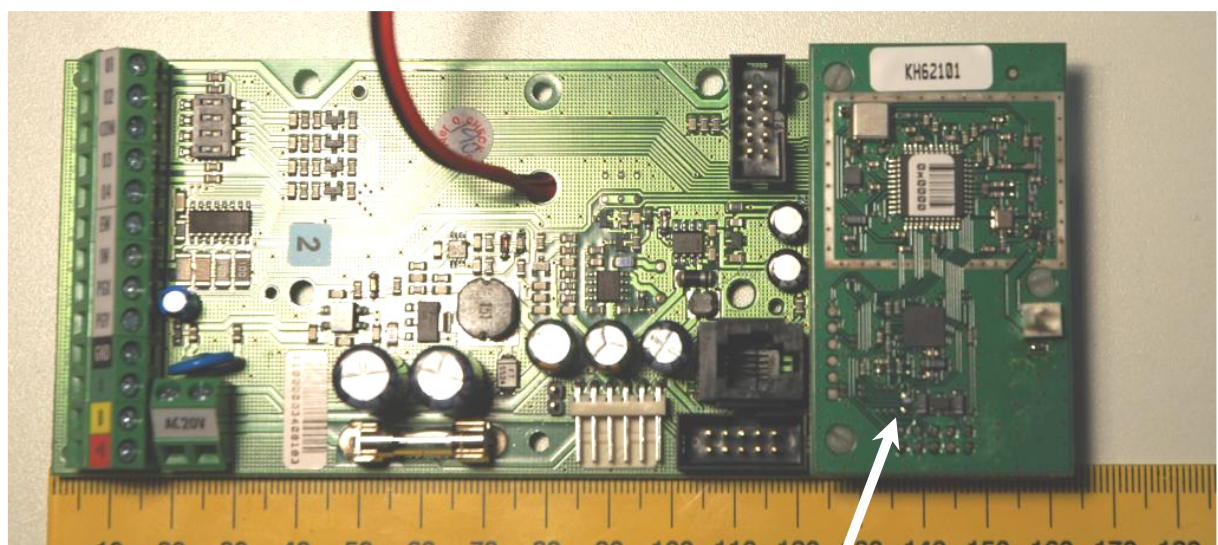
PCB of JA-82R connection to PCB of JA82K-US
