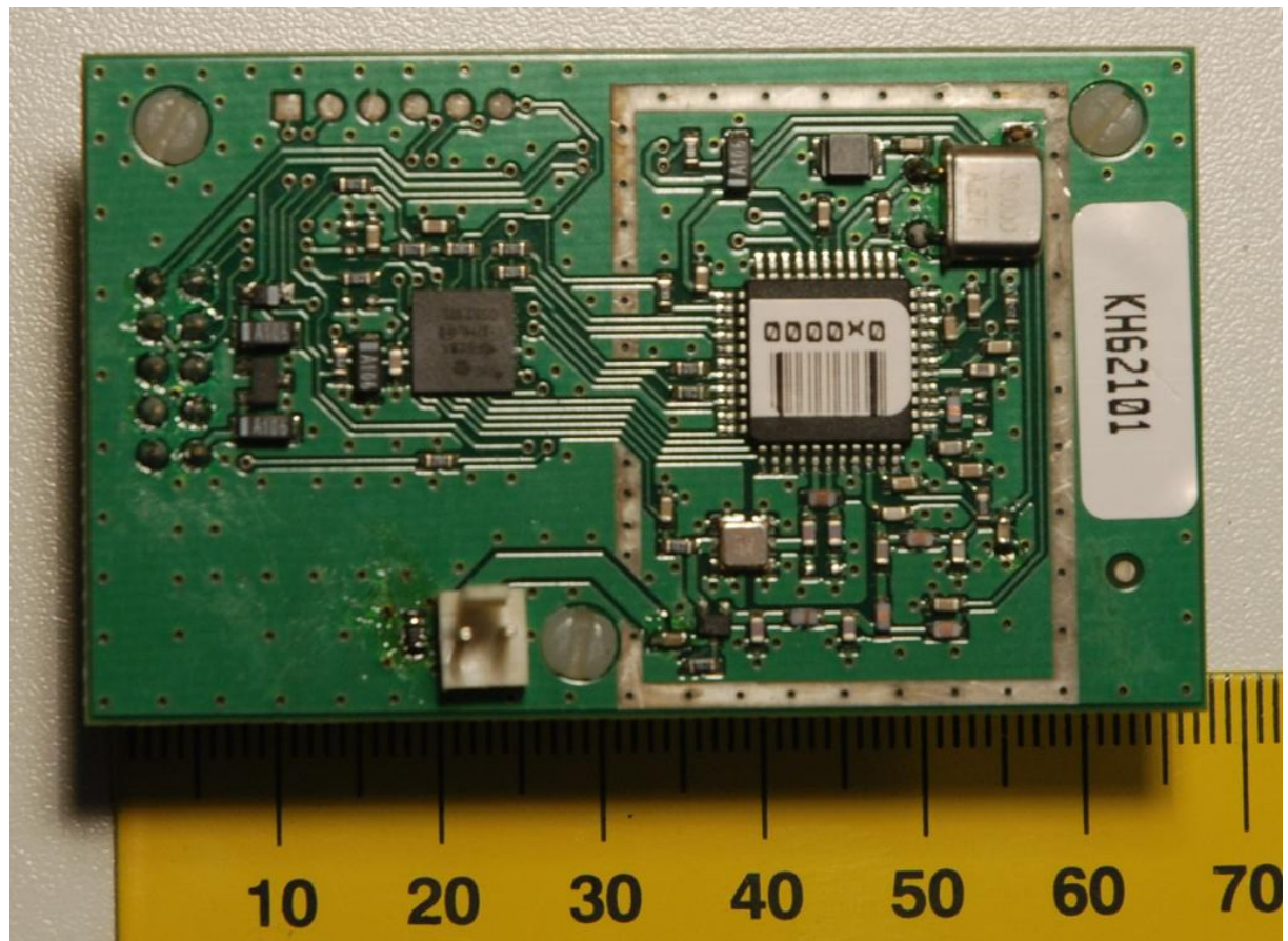
Front view with antenna connector
