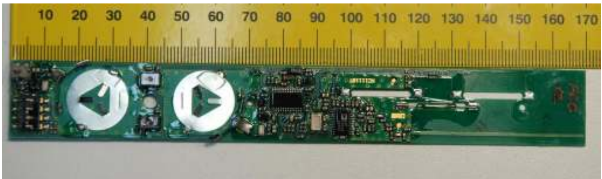
PCB – battery side
