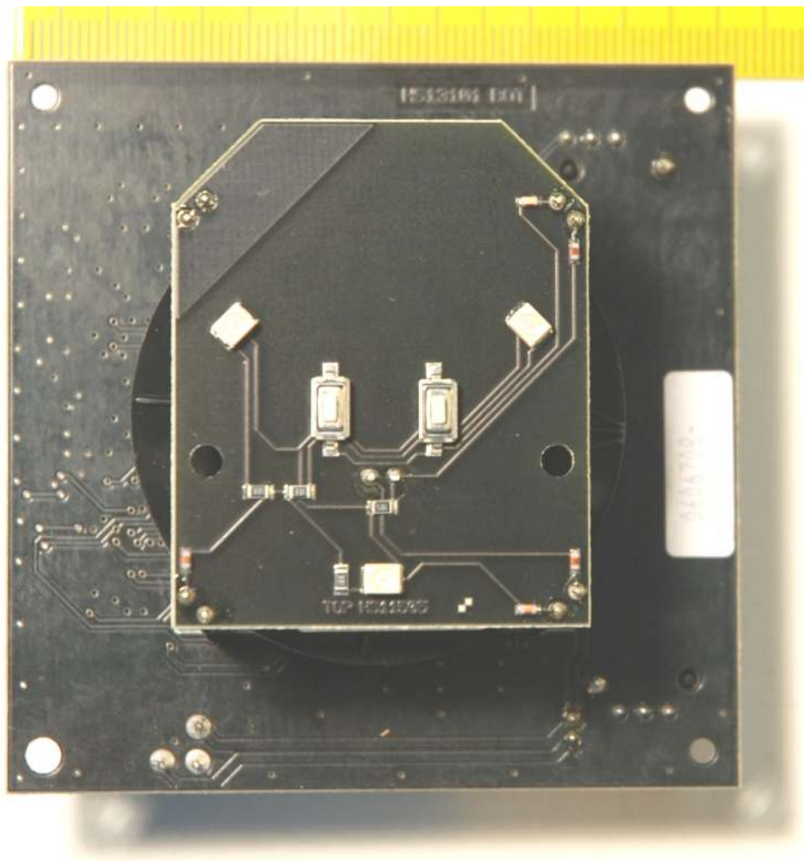
PCB rear view (sensor side)
