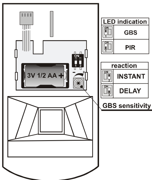
Glass-break detector
