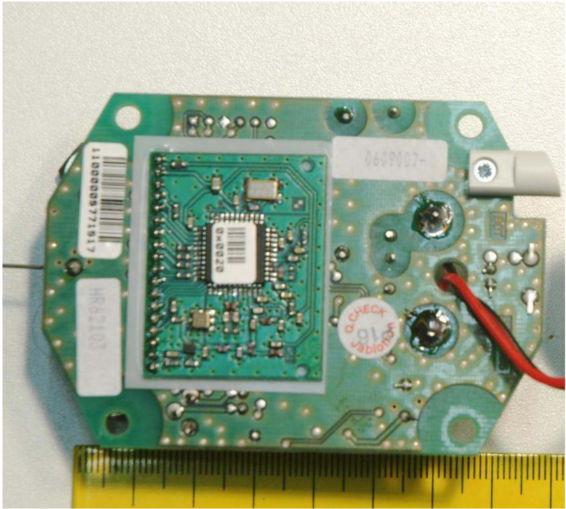
Rear view
