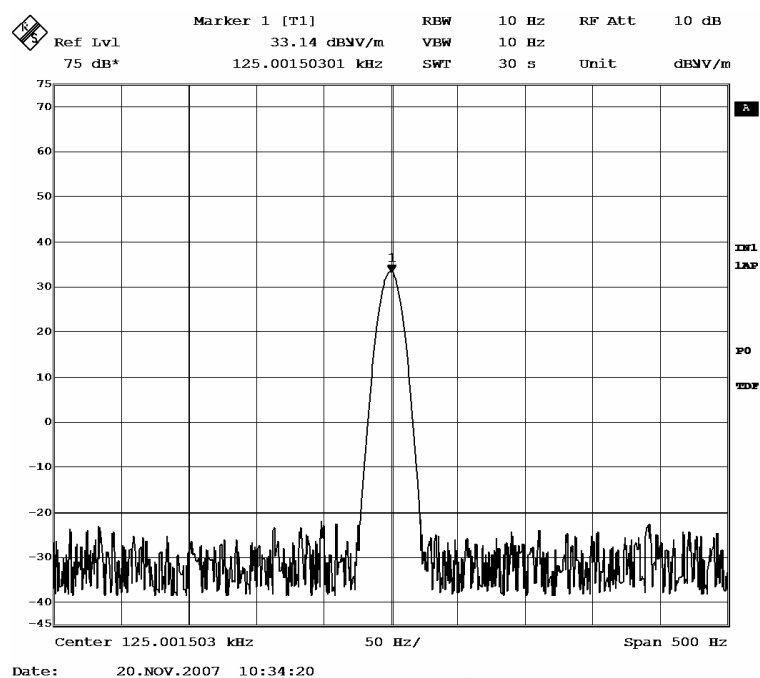
Fig.3 T = -30^{\circ}\text{C}
