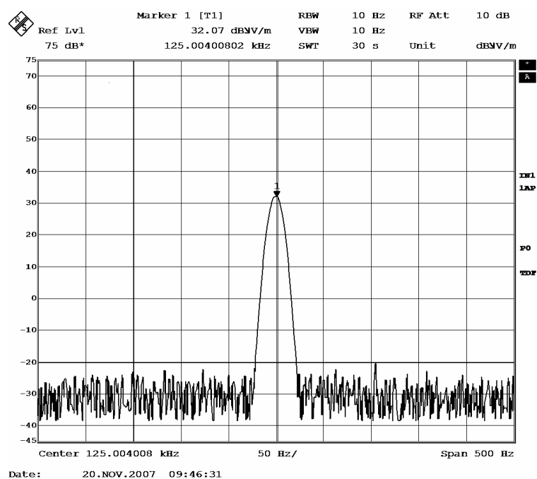
Fig.2 T = 22^{\circ}\text{C}
