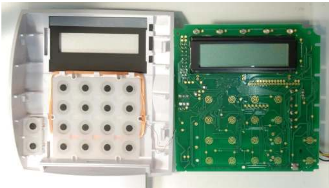
Internal view with antenna – PCB rear side
