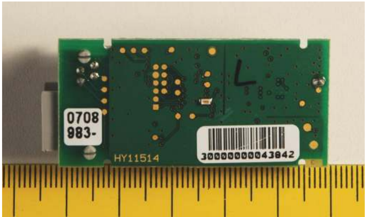
Fig.2 PCB solder view
