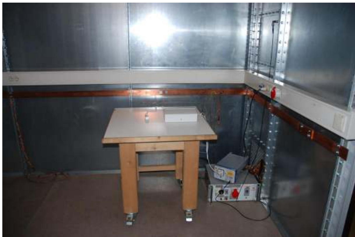
Fig. 3 Conducted emissions setup
