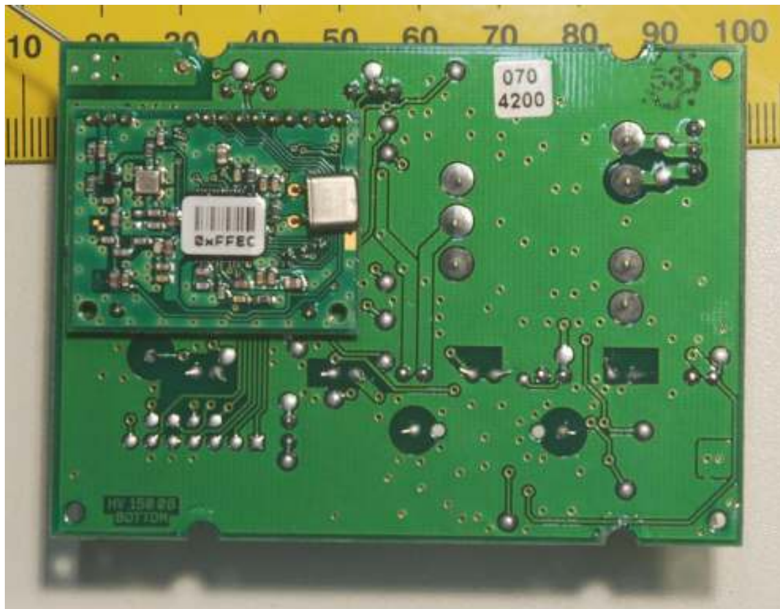
PCB rear view
