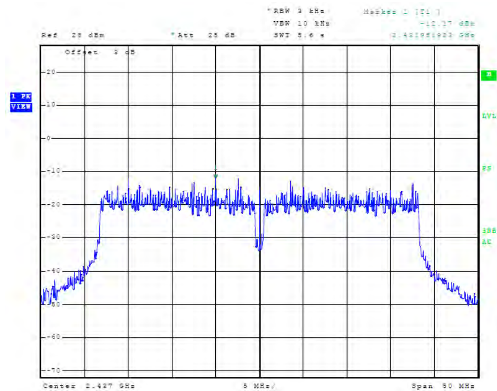
Figure 90 Plot of Antenna Port Conducted Power Spectral Density (chain2, 2437 MHz, 40 MHz Mode)
