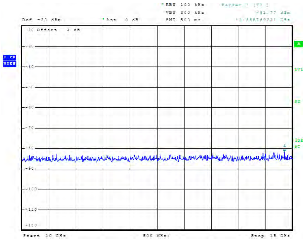
Figure 135 Plot of Receiver Antenna Port Conducted Emissions
