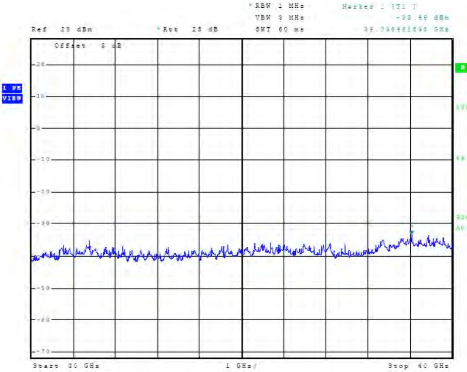
Figure 126 Plot of Antenna Port Conducted Emissions (5 GHz chain2, operation)
