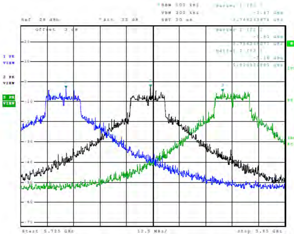
Figure 100 Plot of Antenna Port Conducted (5GHz, chain2, Operational Band, 20MHz Mode)
