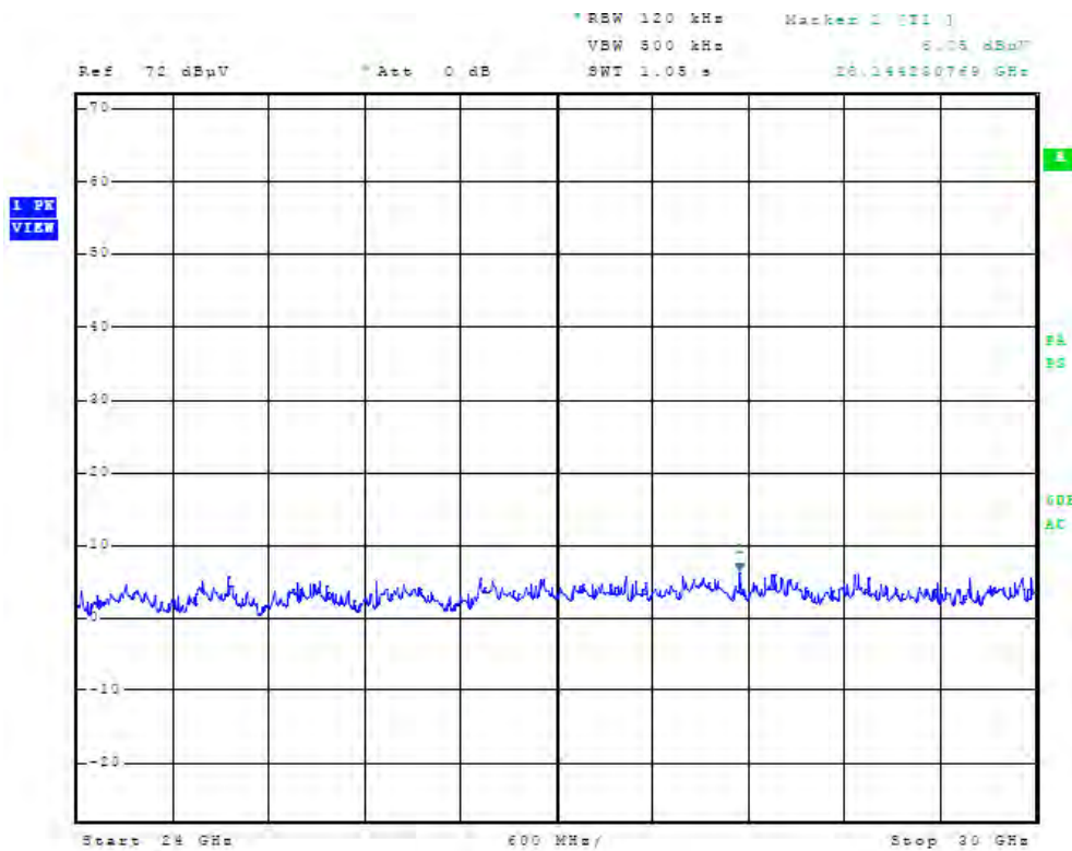
Figure 144 Plot of Receiver Radiated Spurious Emissions taken at 1 meter
