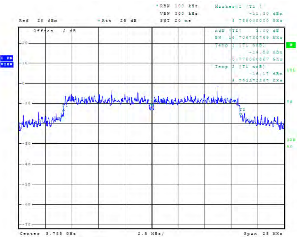
Figure 106 Plot of Antenna Port Conducted 6dB Band width (chain2, 5785 MHz, 20 MHz Mode)
