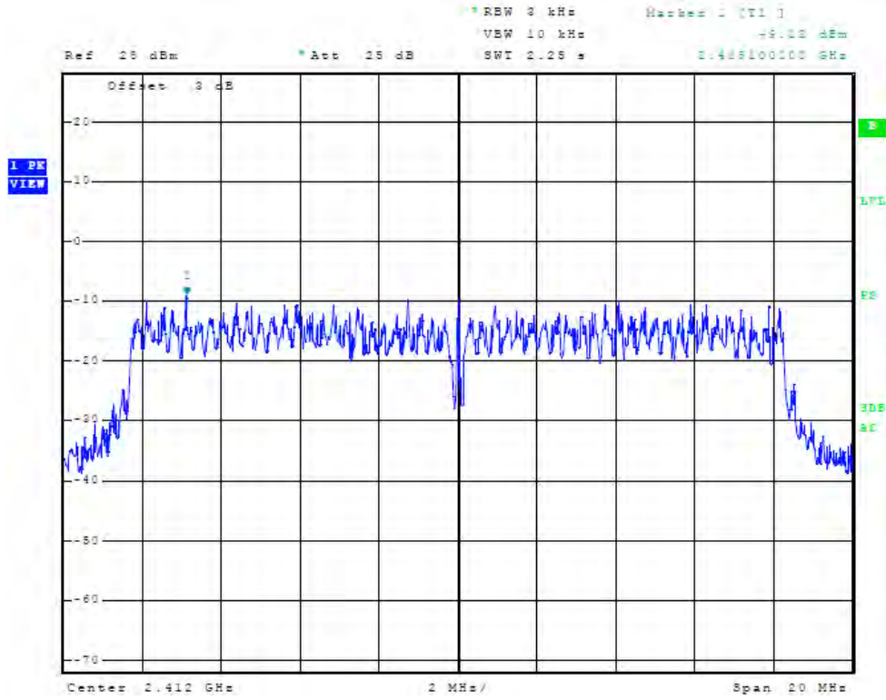
Figure 27 Plot of Antenna Port Conducted Power Spectral Density (chain1, 2412 MHz, 20 MHz Mode)
