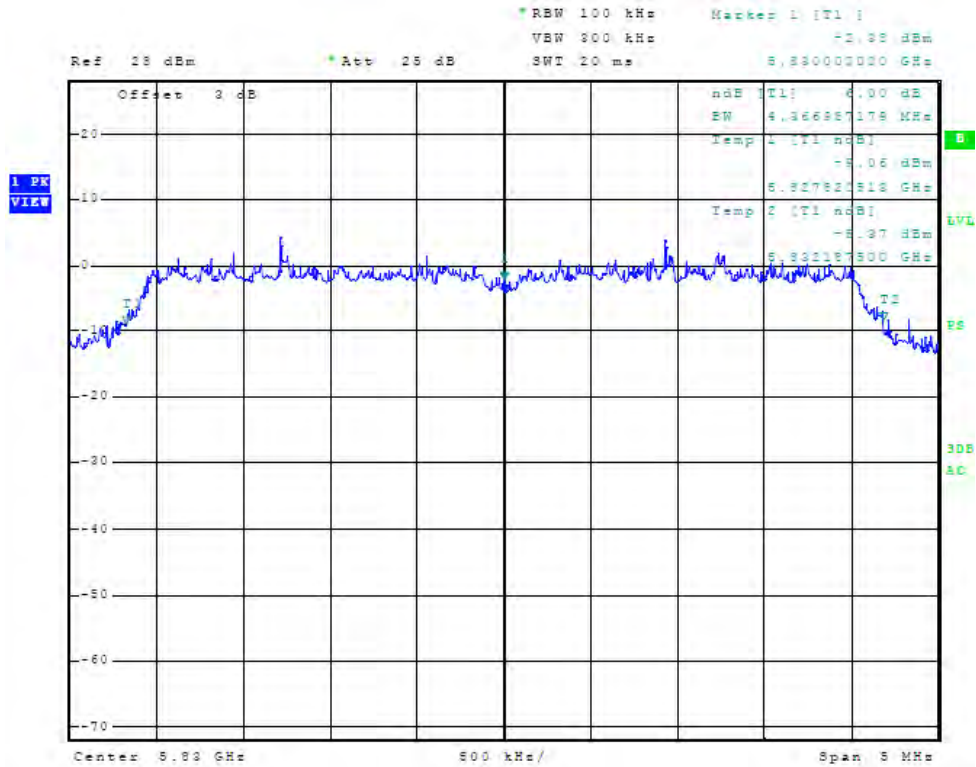
Figure 45 Plot of Antenna Port Conducted 6dB Band width (chain 1, 5830 MHz, 5 MHz Mode)
