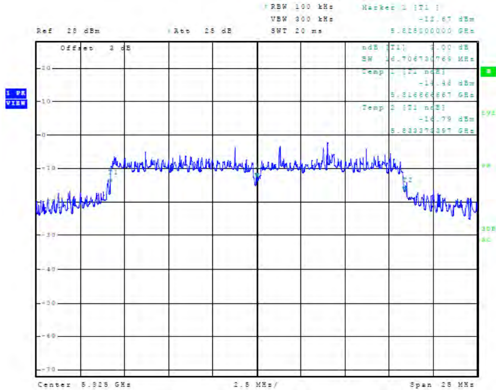
Figure 107 Plot of Antenna Port Conducted 6dB Band width (chain2, 5825 MHz, 20 MHz Mode)
