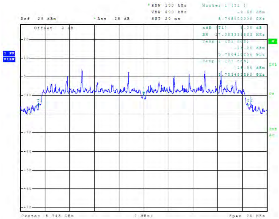
Figure 46 Plot of Antenna Port Conducted 6dB Band width (chain 1, 5745 MHz, 20 MHz Mode)
