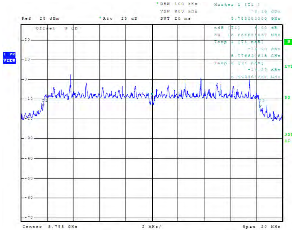
Figure 47 Plot of Antenna Port Conducted 6dB Band width (chain 1, 5785 MHz, 20 MHz Mode)
