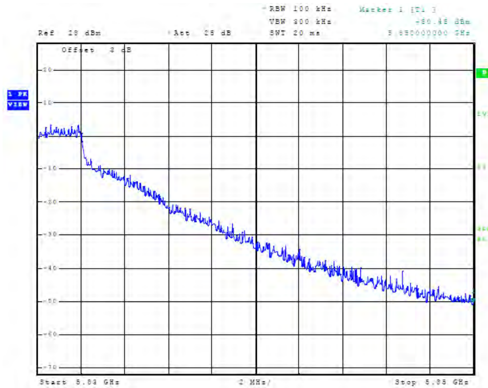
Figure 70 Plot of Antenna Port Conducted High Band Edge Compliance (5 GHz, chain1, operation)
