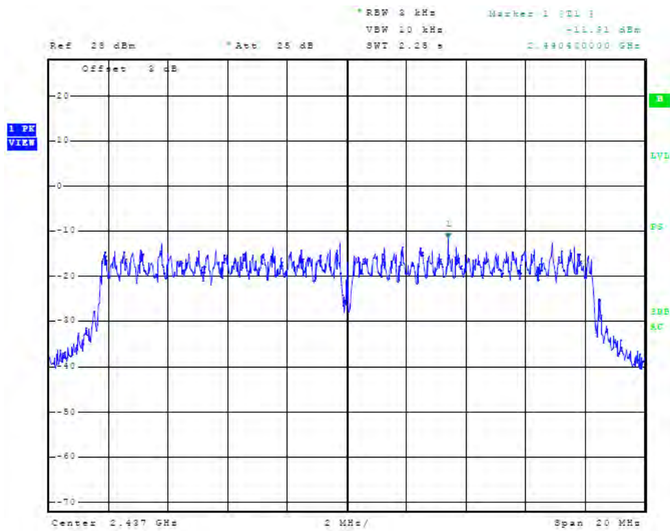
Figure 28 Plot of Antenna Port Conducted Power Spectral Density (chain1, 2437 MHz, 20 MHz Mode)
