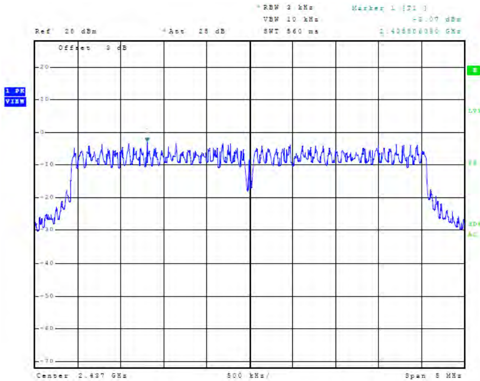
Figure 25 Plot of Antenna Port Conducted Power Spectral Density (chain1, 2437 MHz, 5 MHz Mode)
