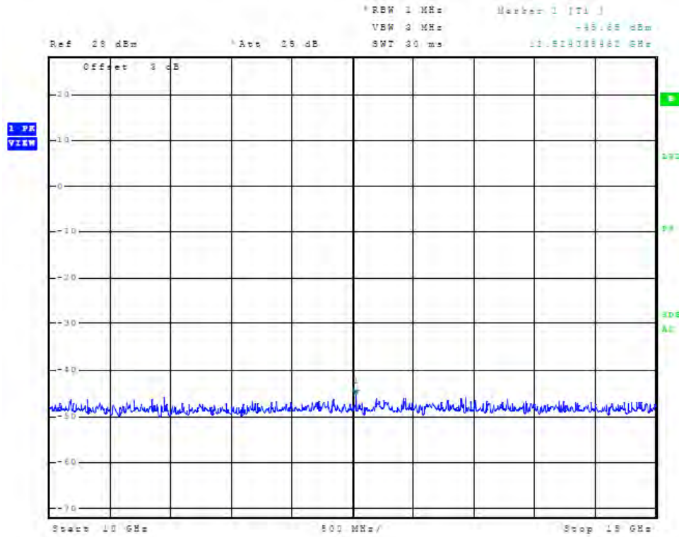
Figure 95 Plot of Antenna Port Conducted Emissions (chain2, 2.4MHz Operation)
