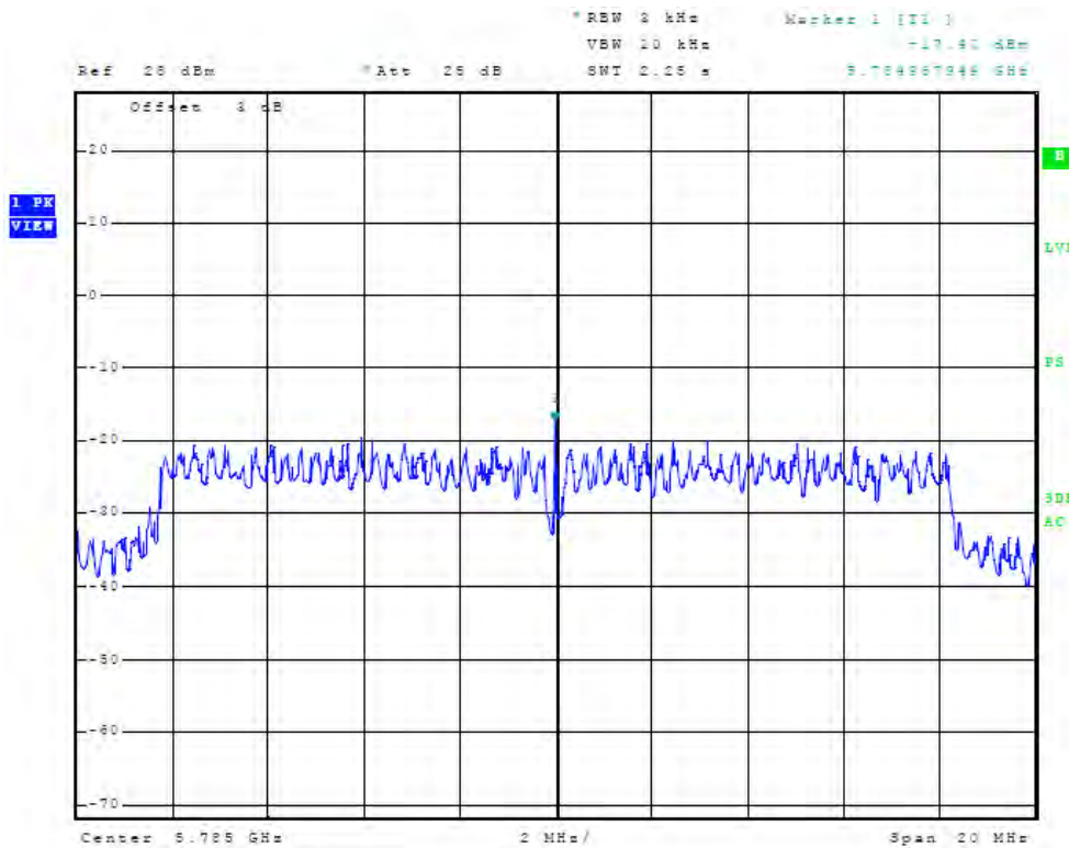
Figure 56 Plot of Antenna Port Conducted Power Spectral Density (chain 1, 5785 GHz, 20MHz Mode)
