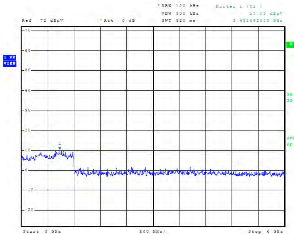
Figure 140 Plot of Receiver Radiated Spurious Emissions taken at 1 meter
