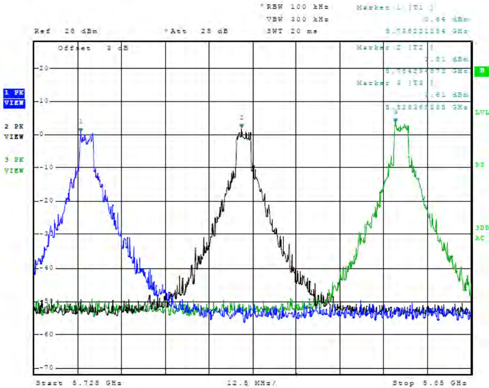
Figure 99 Plot of Antenna Port Conducted (5GHz, chain2, Operational Band, 5MHz Mode)
