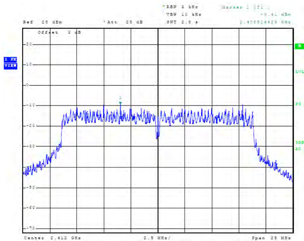
Figure 86 Plot of Antenna Port Conducted Power Spectral Density (chain2, 2412 MHz, 20 MHz Mode)
