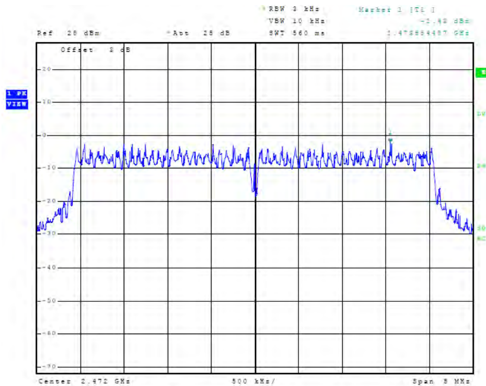
Figure 26 Plot of Antenna Port Conducted Power Spectral Density (chain1, 2472 MHz, 5 MHz Mode)
