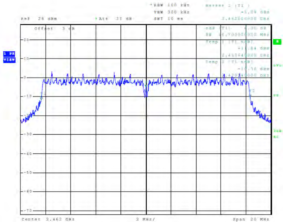
Figure 20 Plot of Antenna Port Conducted 6dB Band width (chain1, 2462 MHz, 20 MHz Mode)
