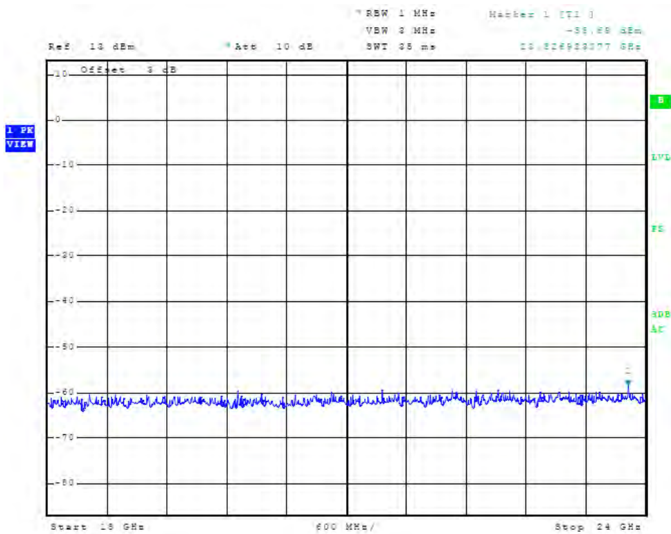
Figure 66 Plot of Antenna Port Conducted Emissions (5 GHz, chain 1, operation)
