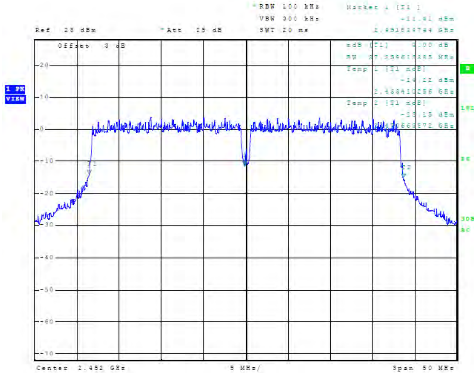
Figure 23 Plot of Antenna Port Conducted 6dB Band width (chain1, 2452 MHz, 40 MHz Mode)
