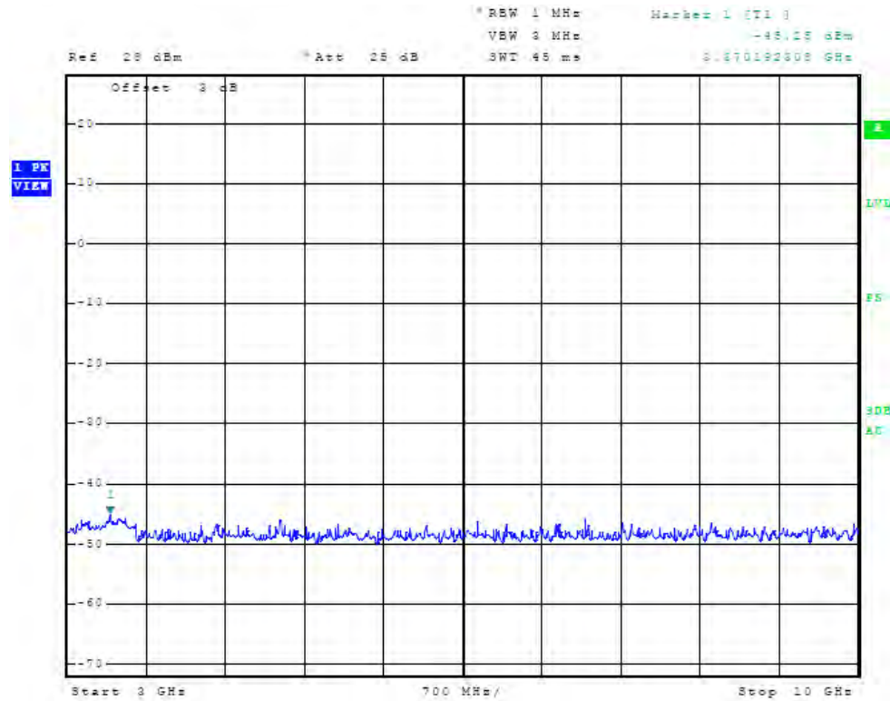
Figure 35 Plot of Antenna Port Conducted Emissions (2 GHz, chain1, Operation)
