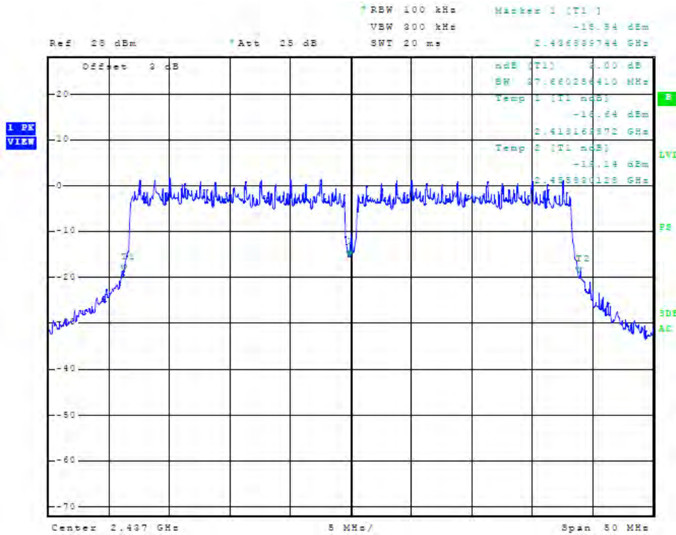
Figure 81 Plot of Antenna Port Conducted 6dB Band width (chain2, 2437 MHz, 40 MHz Mode)
