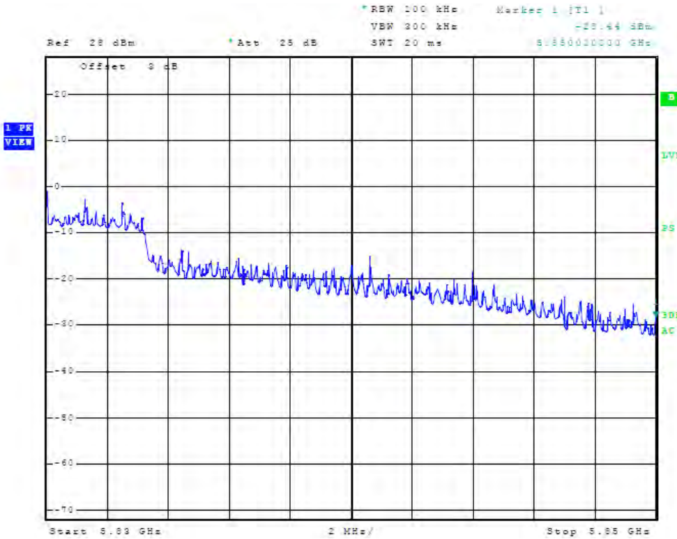
Figure 129 Plot of Antenna Port Conducted High Band Edge Compliance (5 GHz chain2, operation)
