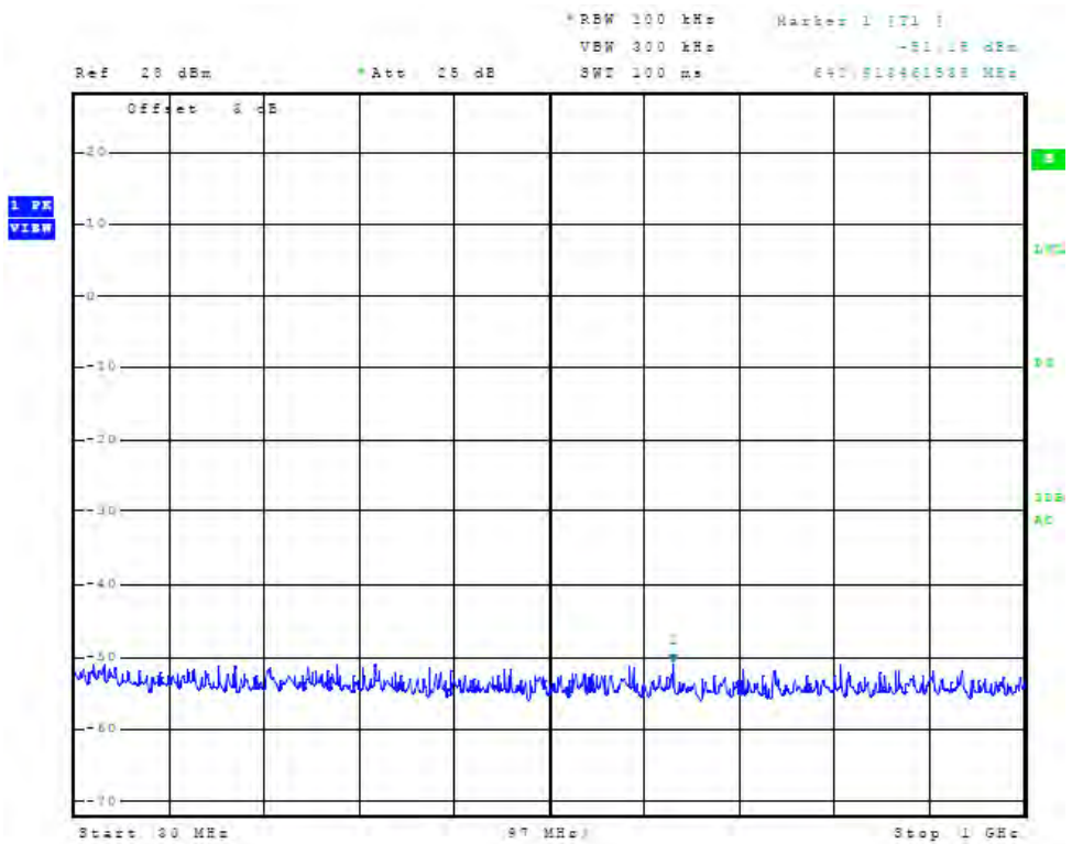
Figure 92 Plot of Antenna Port Conducted Emissions (chain2, 2.4MHz Operation)
