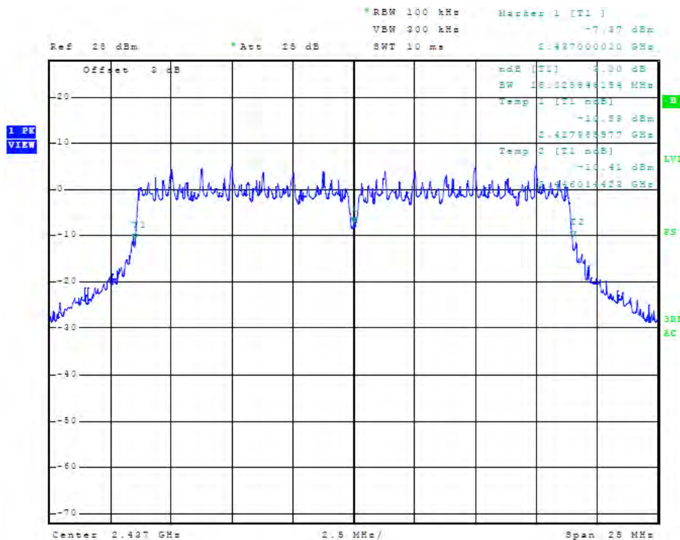
Figure 78 Plot of Antenna Port Conducted 6dB Band width (chain2, 2437 MHz, 20 MHz Mode,)
