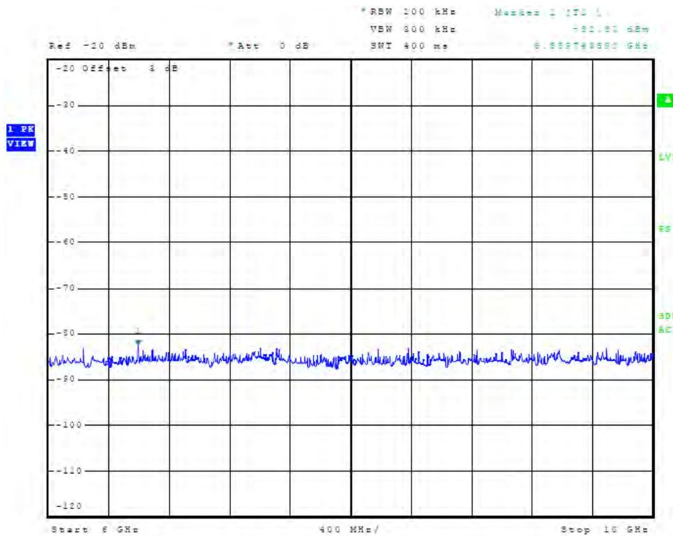
Figure 134 Plot of Receiver Antenna Port Conducted Emissions
