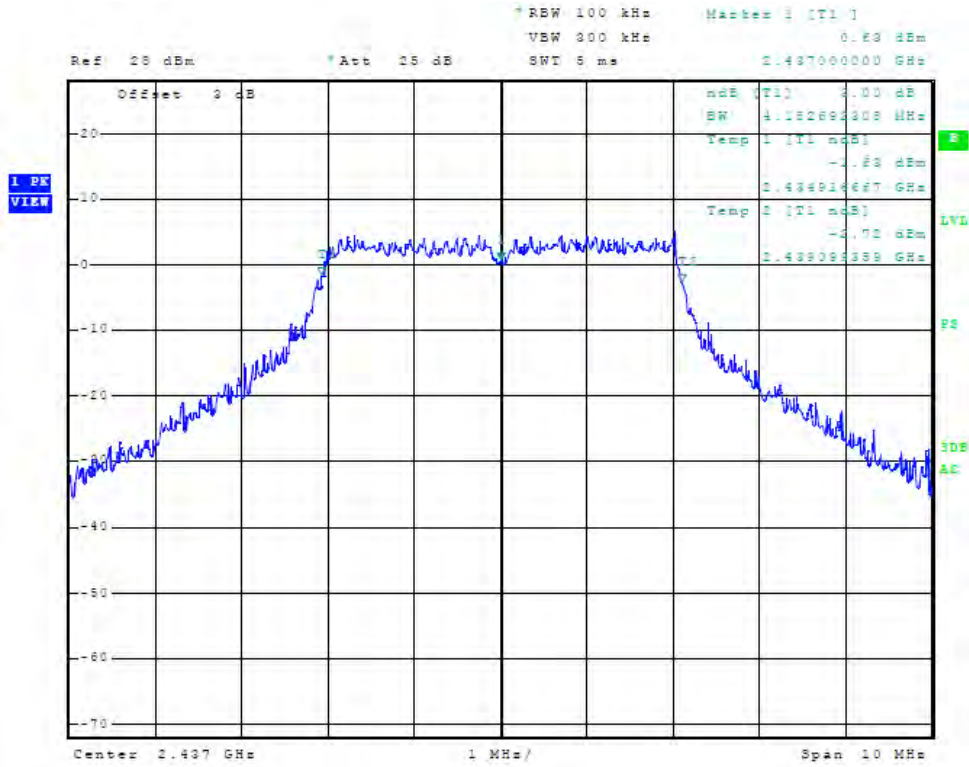
Figure 75 Plot of Antenna Port Conducted 6dB Band width (chain2, 2437 MHz, 5 MHz Mode)
