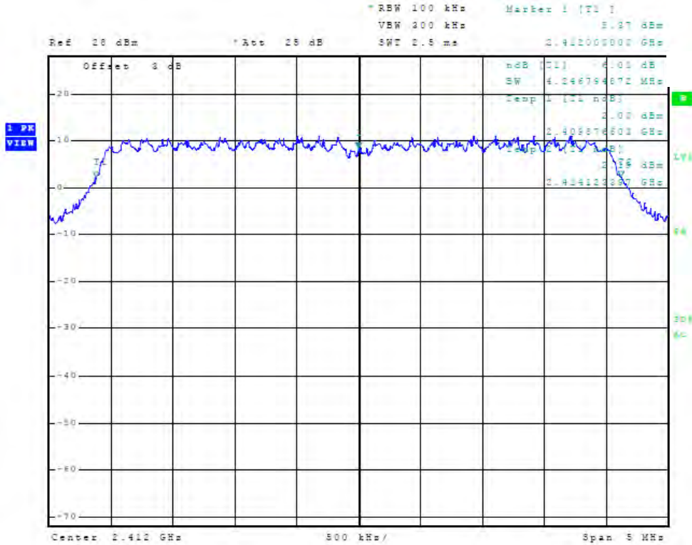
Figure 15 Plot of Antenna Port Conducted 6dB Band width (chain1, 2412 MHz, 5 MHz Mode)
