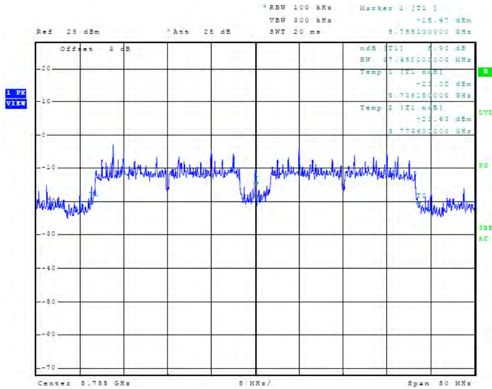
Figure 49 Plot of Antenna Port Conducted 6dB Band width (chain 1, 5755 MHz, 40 MHz Mode)
