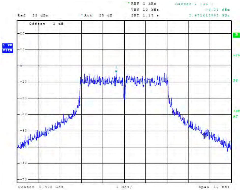
Figure 85 Plot of Antenna Port Conducted Power Spectral Density (chain2, 2472 MHz, 5 MHz Mode)
