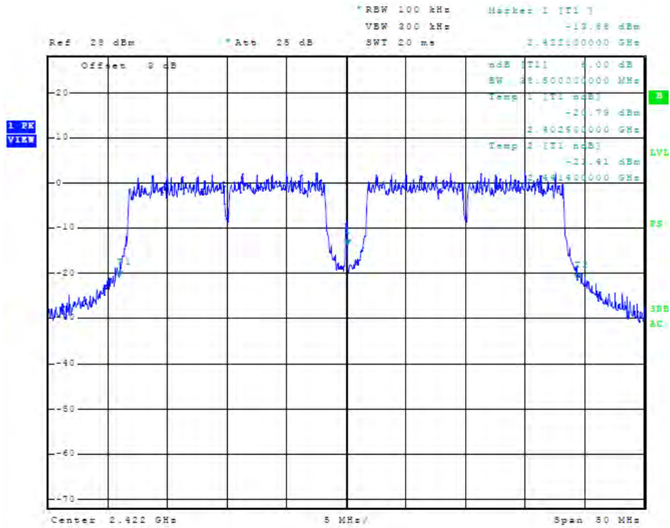
Figure 21 Plot of Antenna Port Conducted 6dB Band width (chain1, 2422 MHz, 40 MHz Mode)
