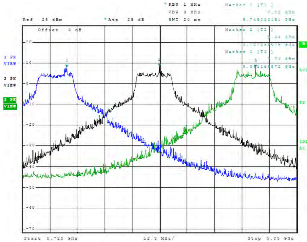
Figure 41 Plot of Antenna Port Conducted (5GHz, chain1, Operational Band, 20MHz Mode)
