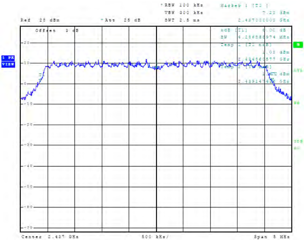
Figure 16 Plot of Antenna Port Conducted 6dB Band width (chain1, 2437 MHz, 5 MHz Mode)
