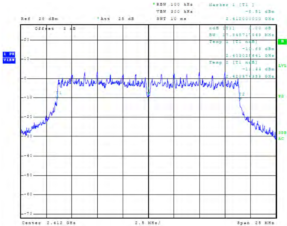
Figure 77 Plot of Antenna Port Conducted 6dB Band width (chain2, 2412 MHz, 20 MHz Mode)
