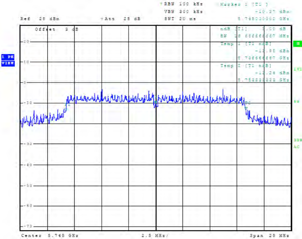
Figure 105 Plot of Antenna Port Conducted 6dB Band width (chain2, 5745 MHz, 20 MHz Mode)
