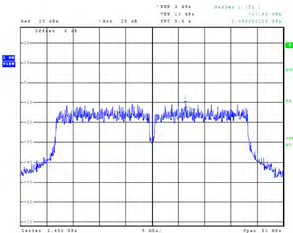
Figure 32 Plot of Antenna Port Conducted Power Spectral Density (chain1, 2452 MHz, 40 MHz Mode)
