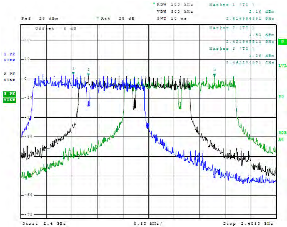
Figure 73 Plot of Antenna Port Conducted (2GHz, chain2, 2 Operational Band, 40MHz Mode)
