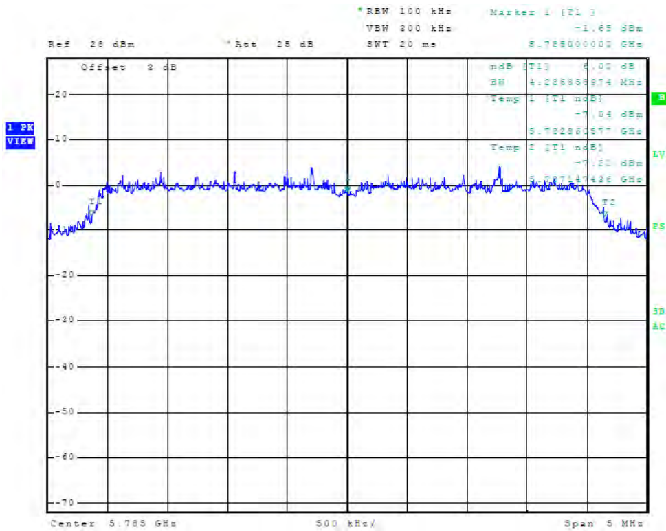
Figure 44 Plot of Antenna Port Conducted 6dB Band width (chain 1, 5785 MHz, 5 MHz Mode)
