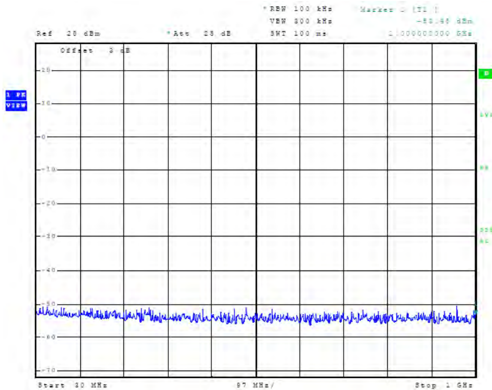
Figure 120 Plot of Antenna Port Conducted Emissions (5 GHz chain2, operation)
