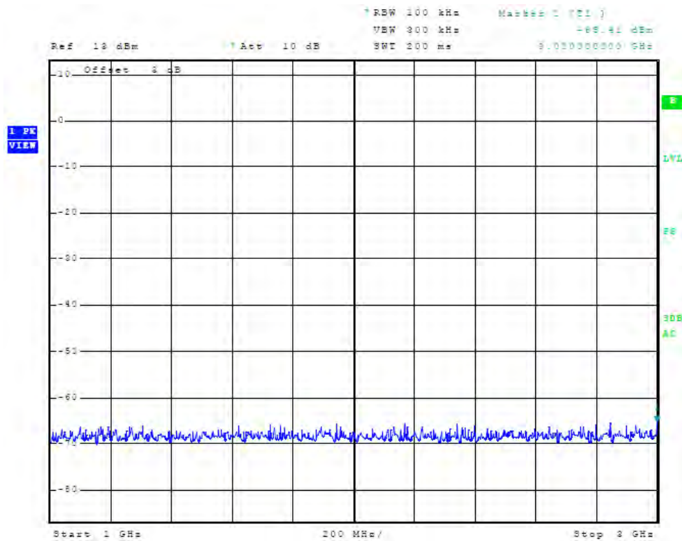
Figure 62 Plot of Antenna Port Conducted Emissions (5 GHz, chain 1, operation)
