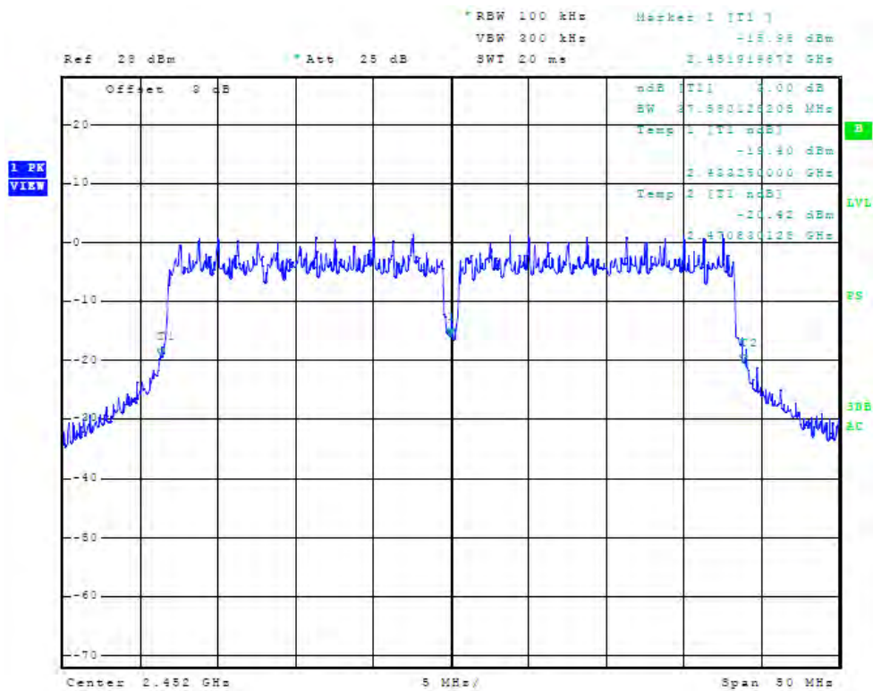
Figure 82 Plot of Antenna Port Conducted 6dB Band width (chain2, 2452 MHz, 40 MHz Mode)
