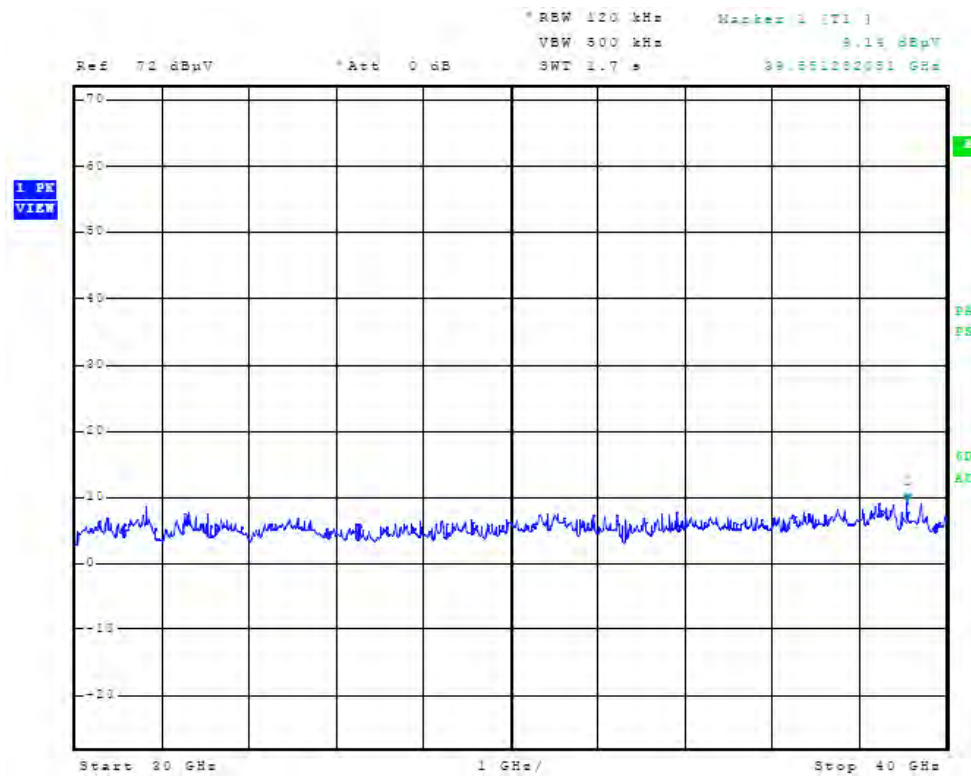
Figure 145 Plot of Receiver Radiated Spurious Emissions taken at 1 meter
