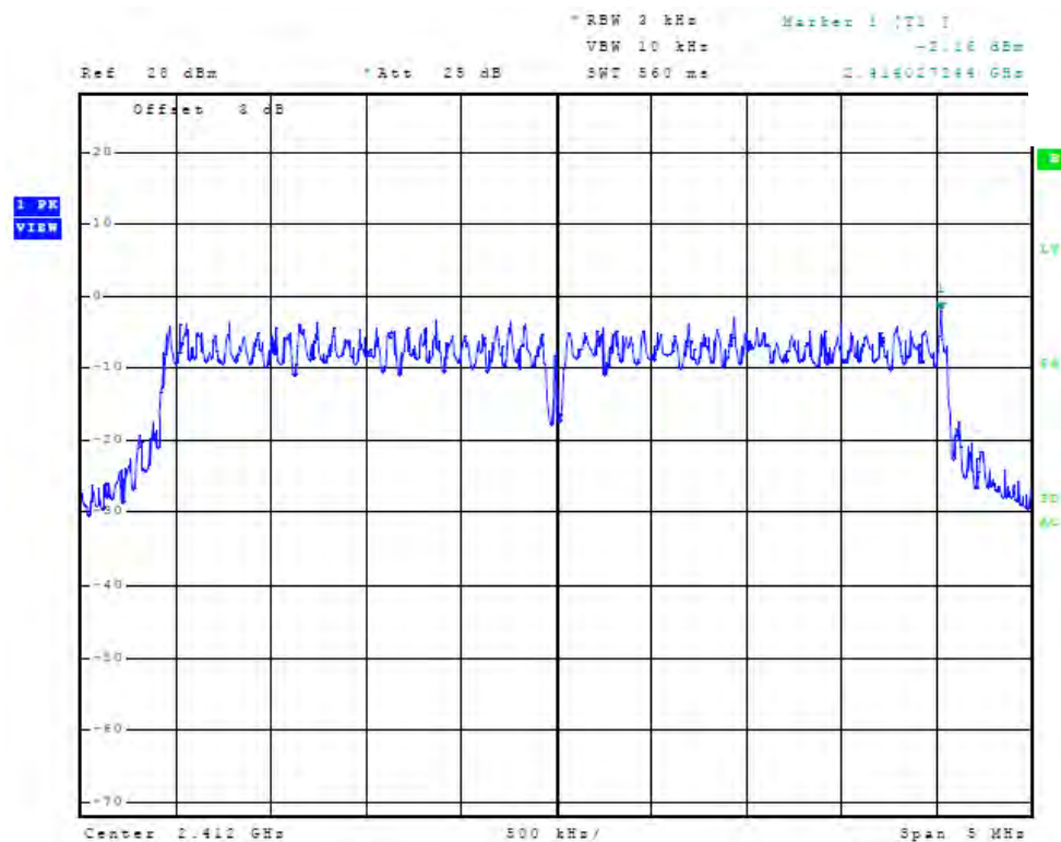
Figure 24 Plot of Antenna Port Conducted Power Spectral Density (chain1, 2412 MHz, 5 MHz Mode)
