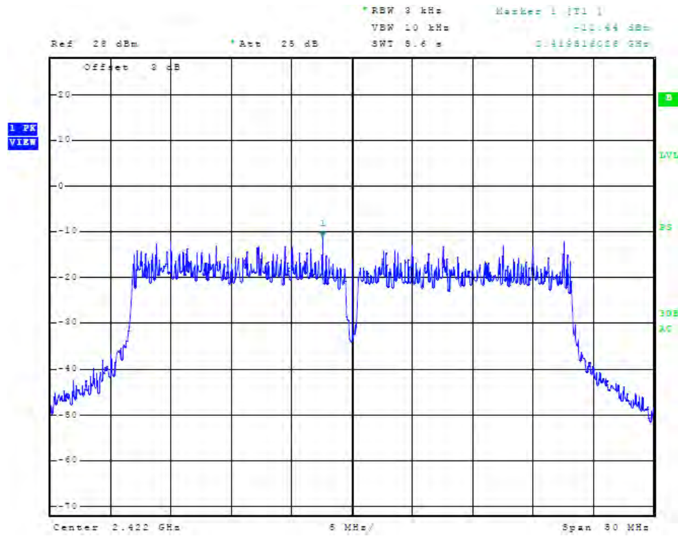
Figure 89 Plot of Antenna Port Conducted Power Spectral Density (chain2, 2422 MHz, 40 MHz Mode)
