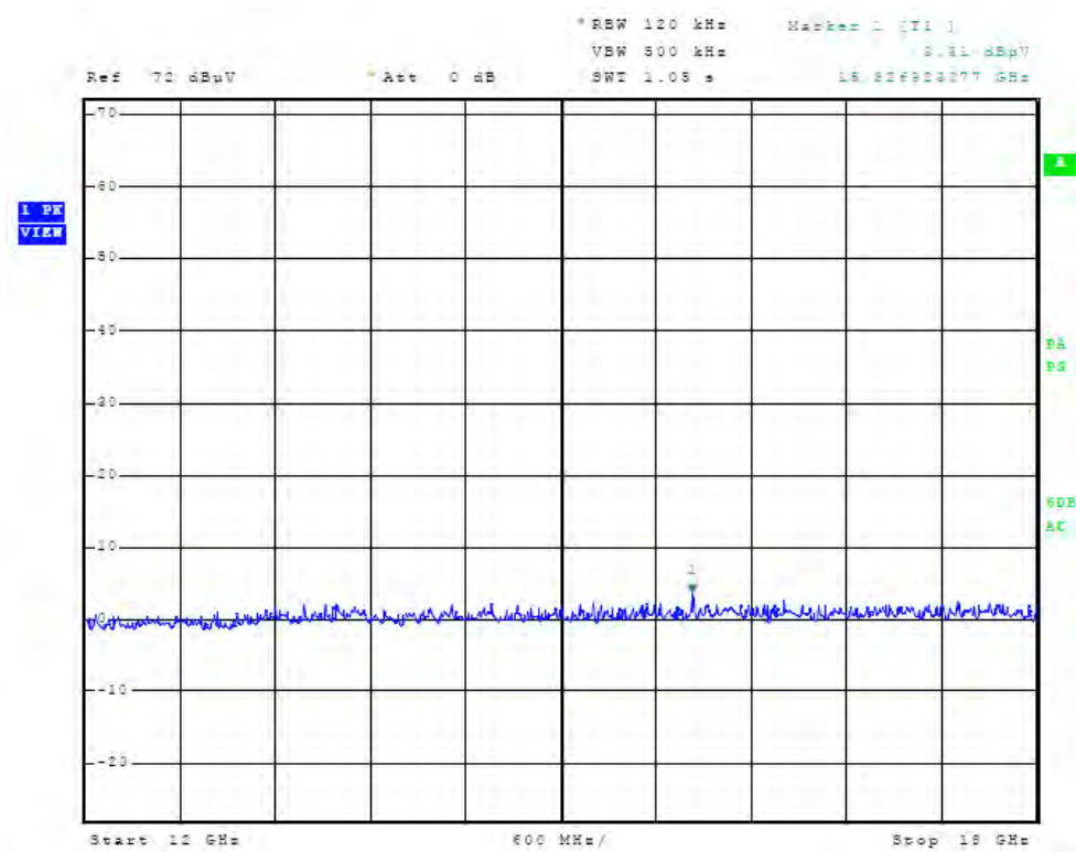
Figure 142 Plot of Receiver Radiated Spurious Emissions taken at 1 meter
