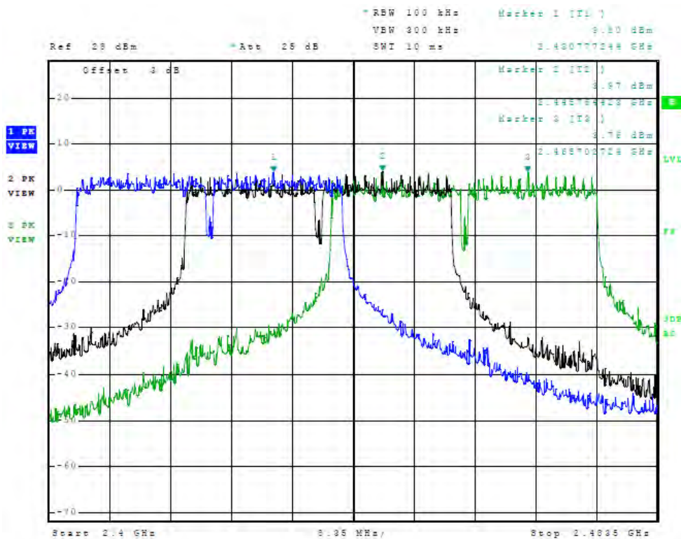
Figure 14 Plot of Antenna Port Conducted (2 GHz, chain1, Operational Band, 40MHz Mode)
