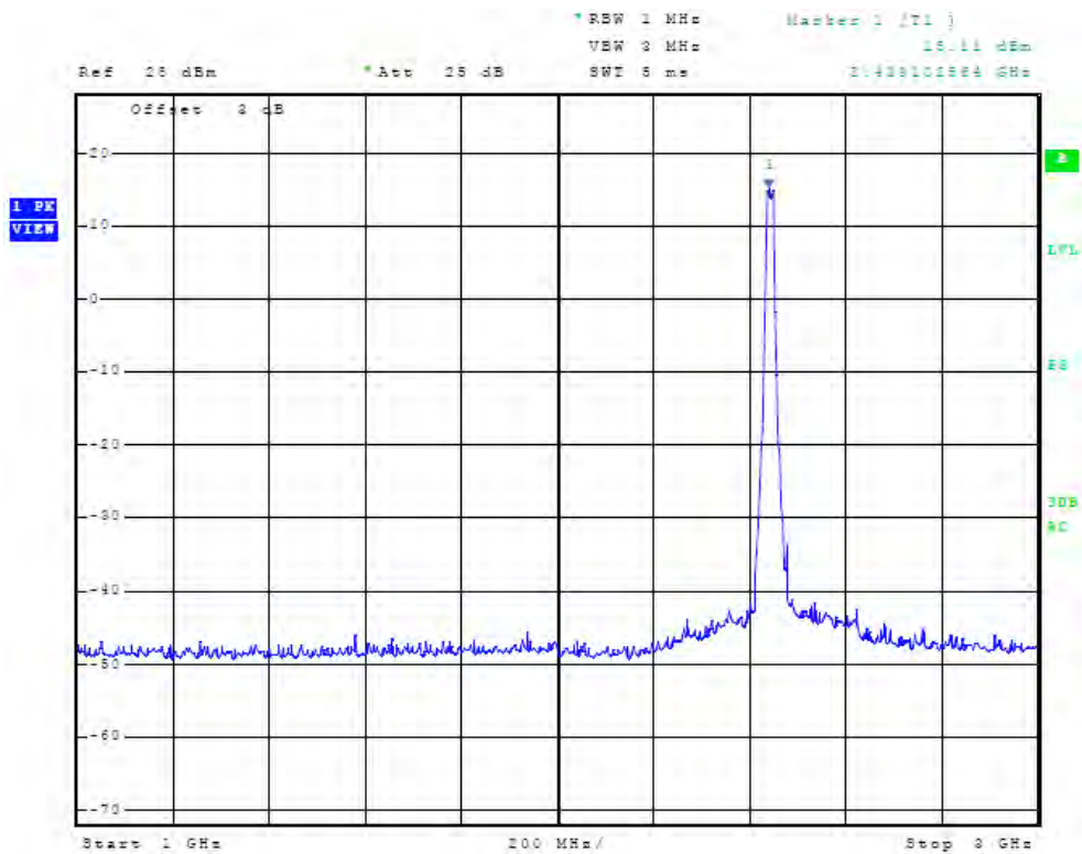
Figure 34 Plot of Antenna Port Conducted Emissions (2 GHz, chain1, Operation)
