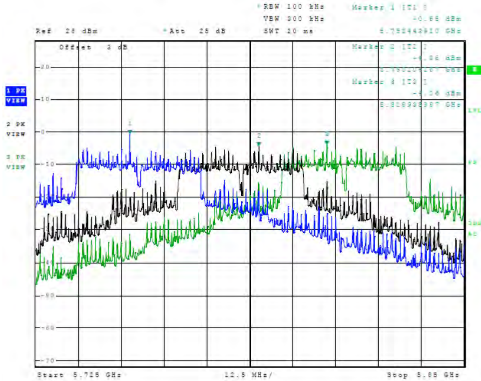
Figure 101 Plot of Antenna Port Conducted (5GHz, chain2, Operational Band, 40MHz Mode)
