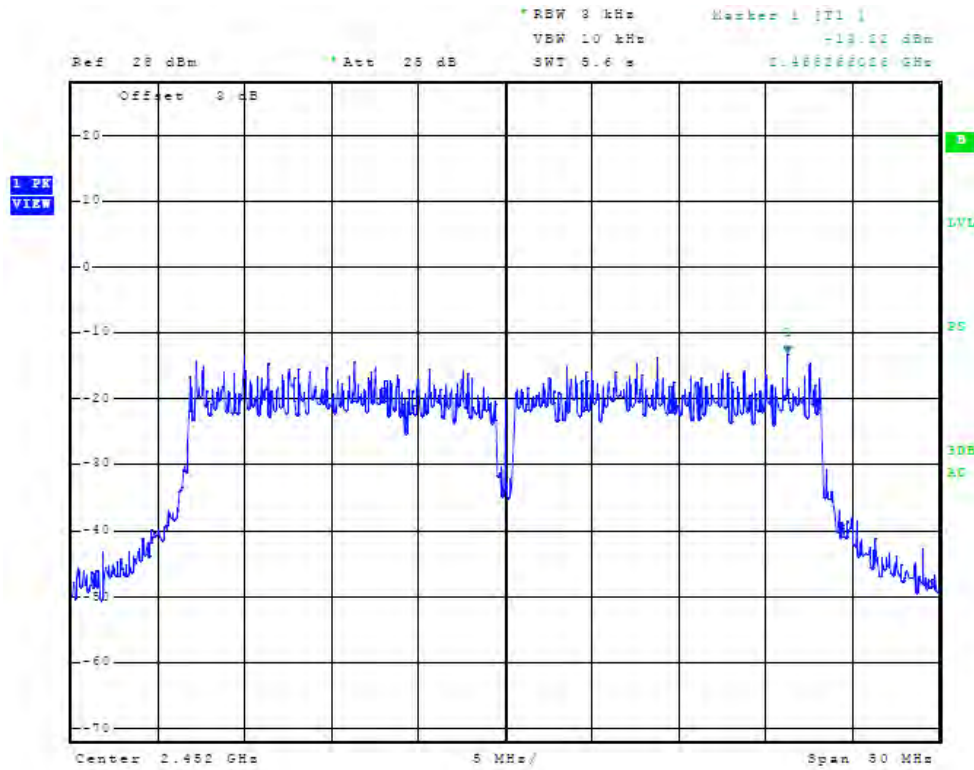
Figure 91 Plot of Antenna Port Conducted Power Spectral Density (chain2, 2452 MHz, 40 MHz Mode)
