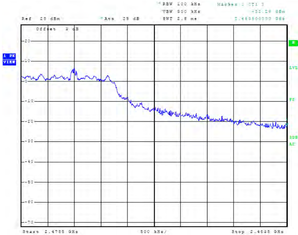
Figure 39 Plot of High Band Edge Compliance at Antenna Port (2 GHz, chain1, Operation)
