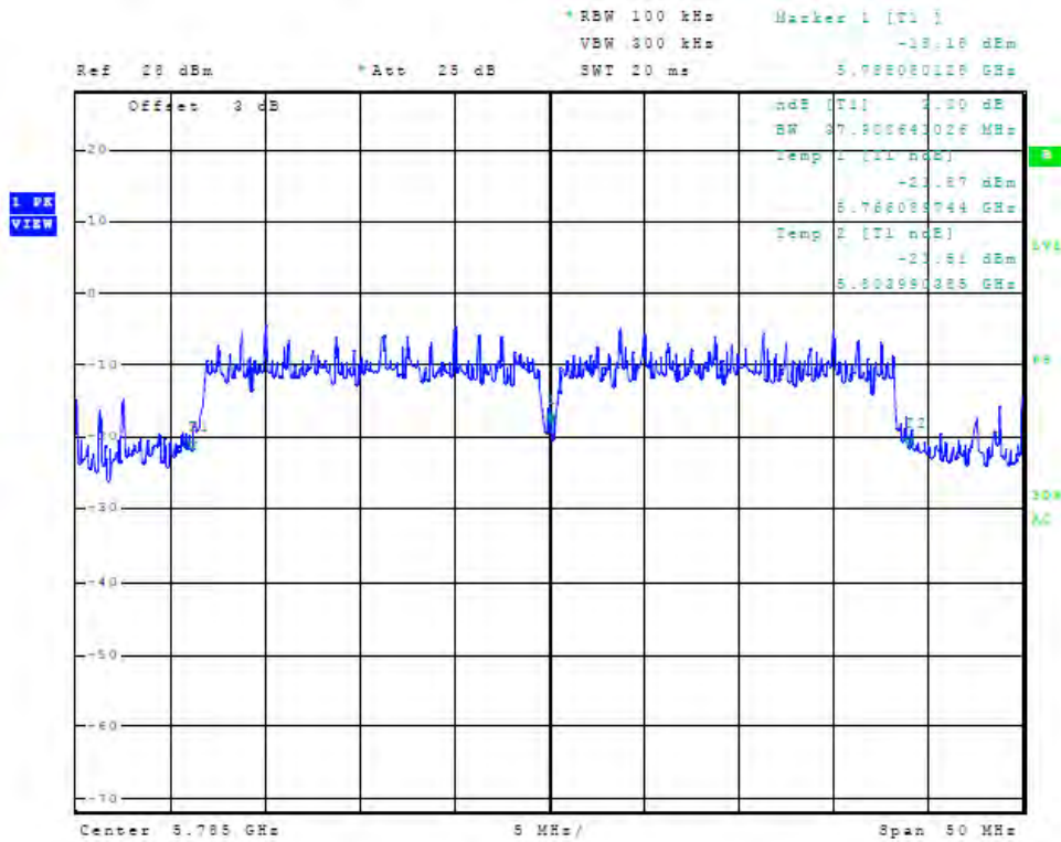
Figure 109 Plot of Antenna Port Conducted 6dB Band width (chain2, 5785 MHz, 40 MHz Mode)
