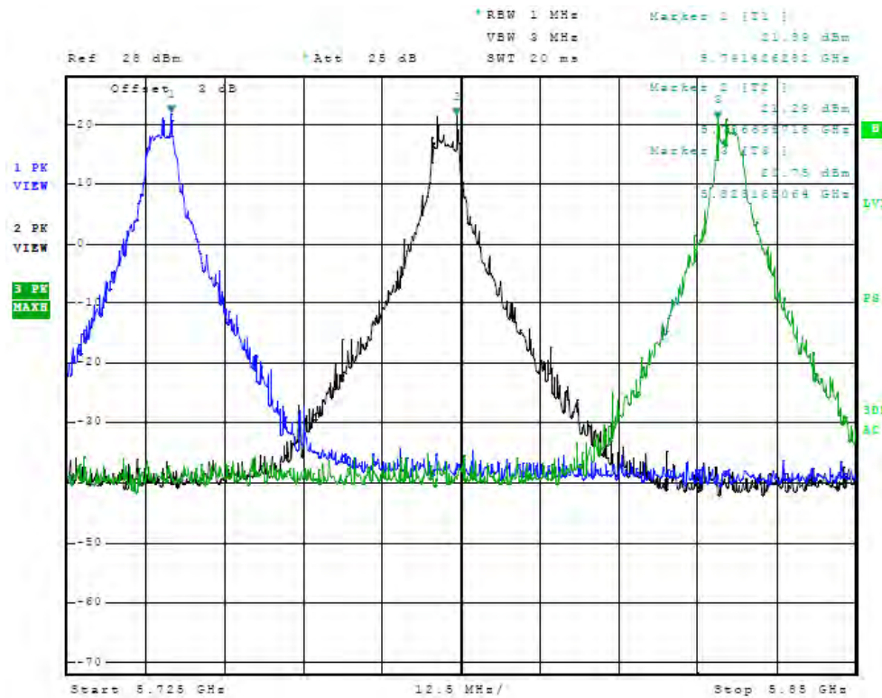
Figure 40 Plot of Antenna Port Conducted (5GHz, chain1, Operational Band, 5MHz Mode)
