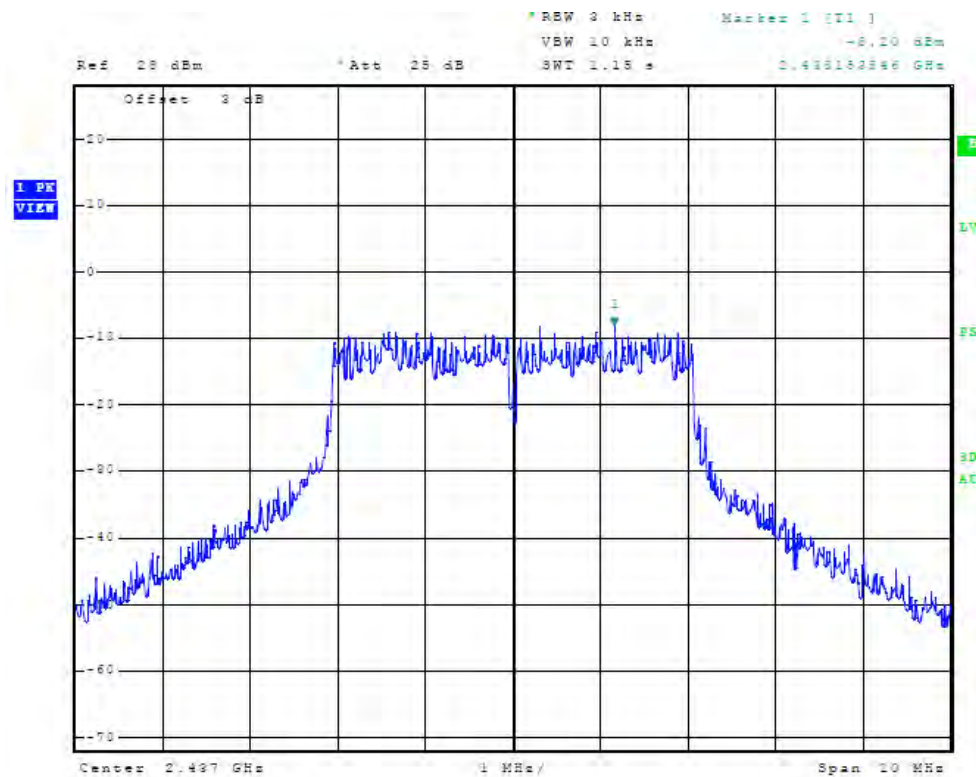
Figure 84 Plot of Antenna Port Conducted Power Spectral Density (chain2, 2437 MHz, 5 MHz Mode)
