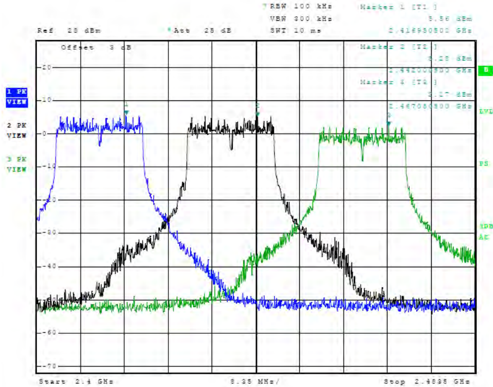
Figure 13 Plot of Antenna Port Conducted (2 GHz, chain1, Operational Band, 20MHz Mode)
