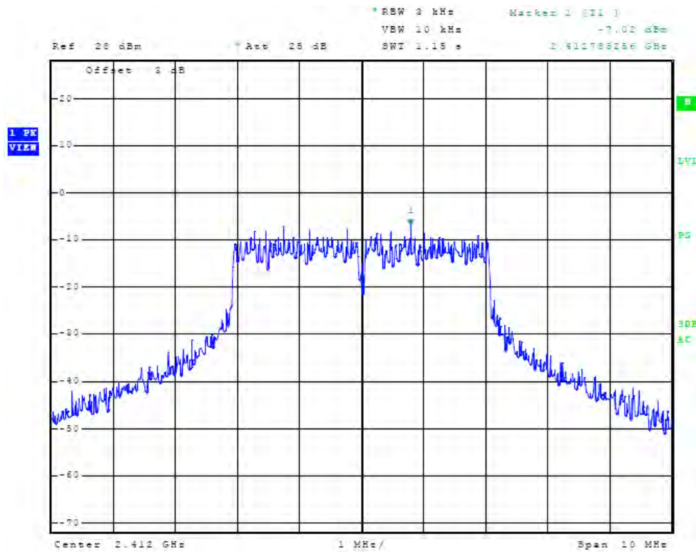
Figure 83 Plot of Antenna Port Conducted Power Spectral Density (chain2, 2412 MHz, 5 MHz Mode)
