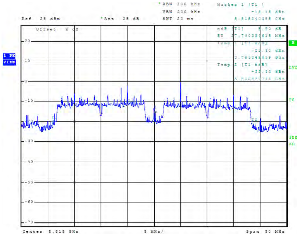
Figure 51 Plot of Antenna Port Conducted 6dB Band width (chain 1, 5815 MHz, 40 MHz Mode)
