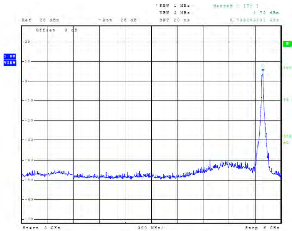
Figure 122 Plot of Antenna Port Conducted Emissions (5 GHz chain2, operation)
