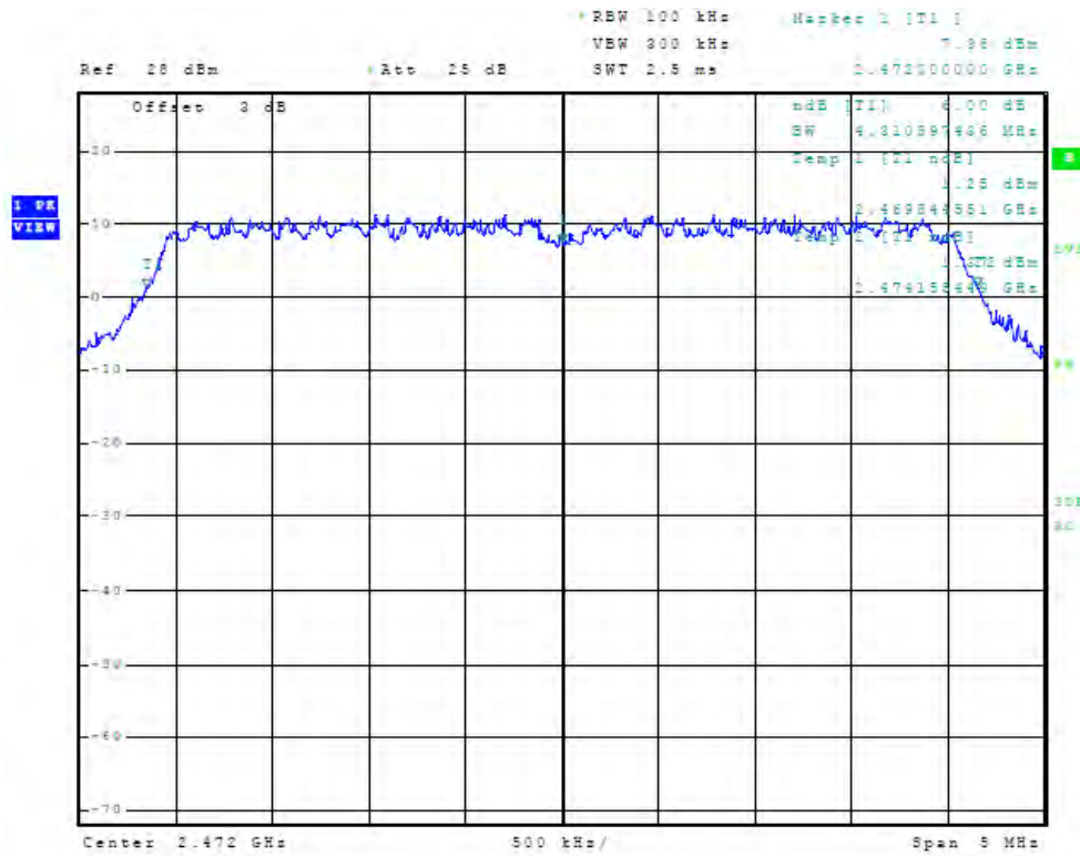
Figure 17 Plot of Antenna Port Conducted 6dB Band width (chain1, 2472 MHz, 5 MHz Mode)
