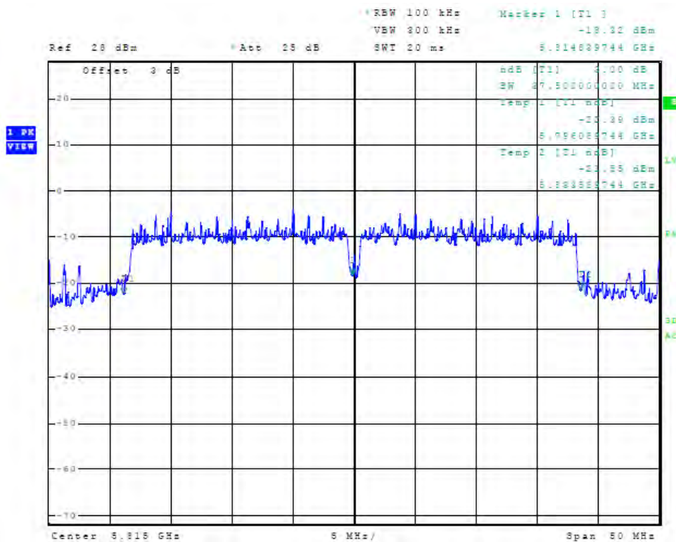
Figure 110 Plot of Antenna Port Conducted 6dB Band width (chain2, 5815 MHz, 40 MHz Mode)
