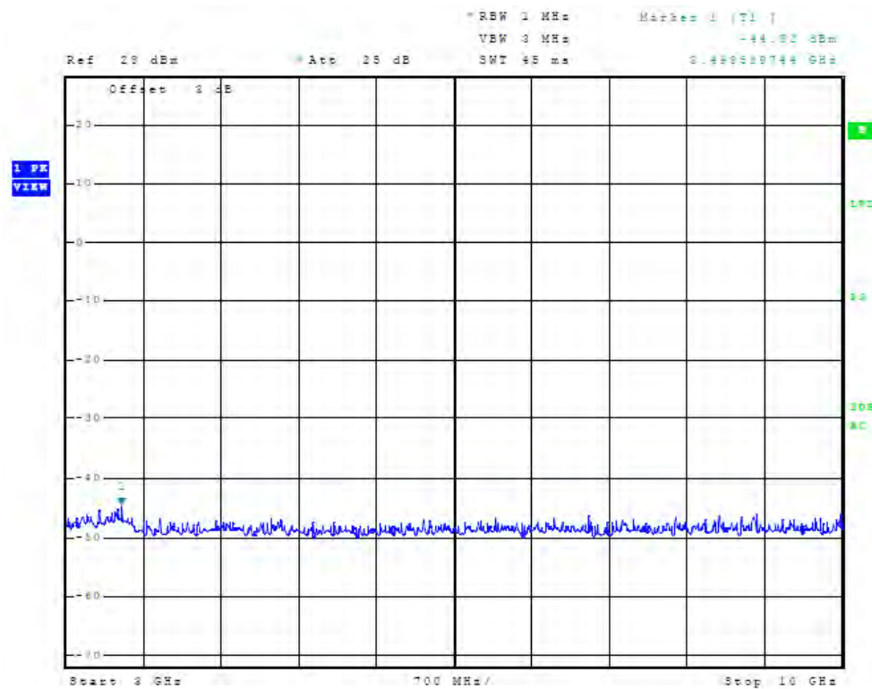
Figure 94 Plot of Antenna Port Conducted Emissions (chain2, 2.4MHz Operation)
