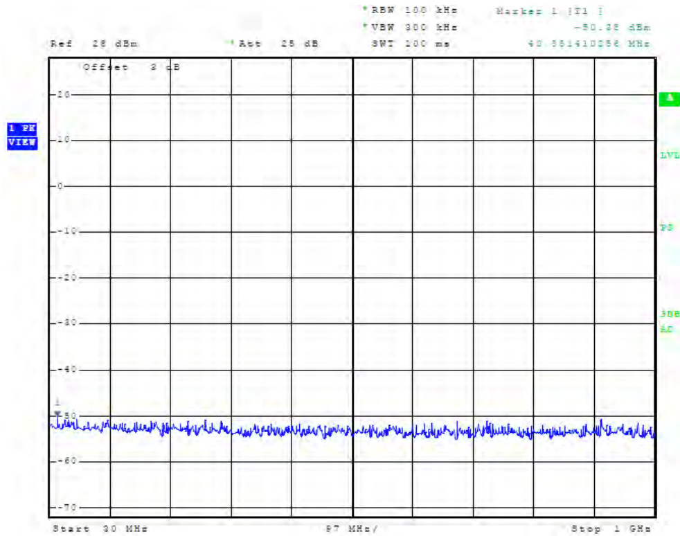
Figure 33 Plot of Antenna Port Conducted Emissions (2 GHz, chain1, Operation)
