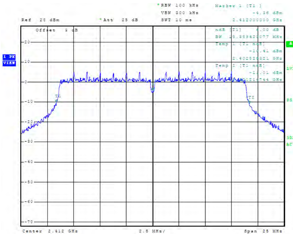
Figure 18 Plot of Antenna Port Conducted 6dB Band width (chain1, 2412 MHz, 20 MHz Mode)
