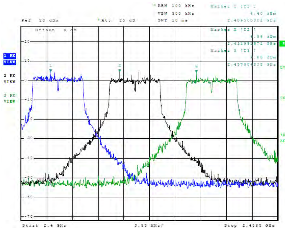
Figure 72 Plot of Antenna Port Conducted (2GHz, chain2, Operational Band, 20MHz Mode)
