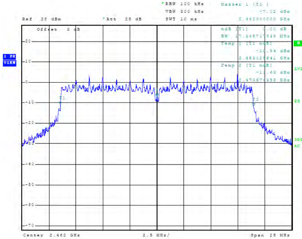
Figure 79 Plot of Antenna Port Conducted 6dB Band width (chain2, 2462 MHz, 20 MHz Mode)
