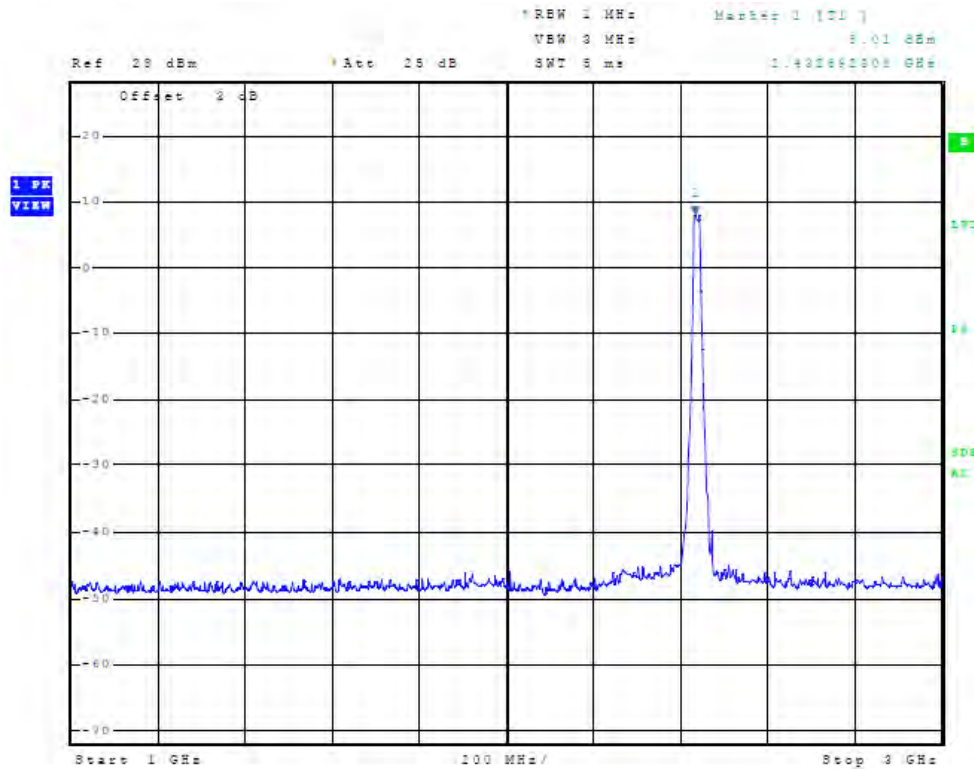
Figure 93 Plot of Antenna Port Conducted Emissions (chain2, 2.4MHz Operation)
