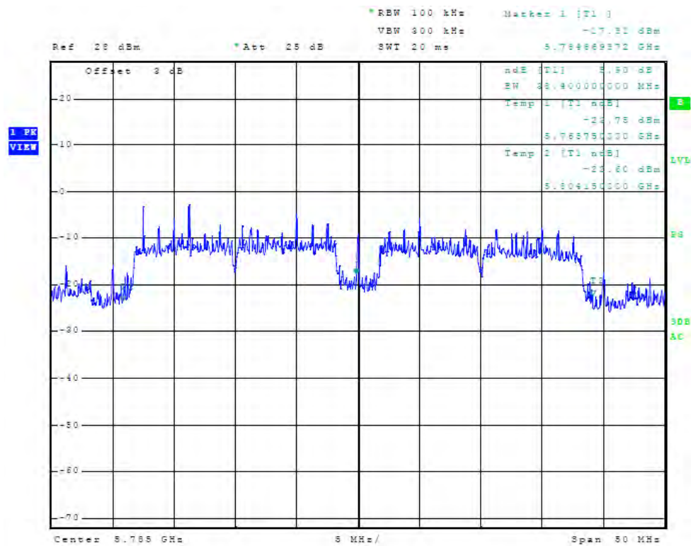
Figure 50 Plot of Antenna Port Conducted 6dB Band width (chain 1, 5785 MHz, 40 MHz Mode)
