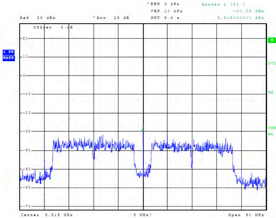
Figure 119 Plot of Antenna Port Conducted Power Spectral Density (chain2, 5815 GHz, 40MHz Mode)
