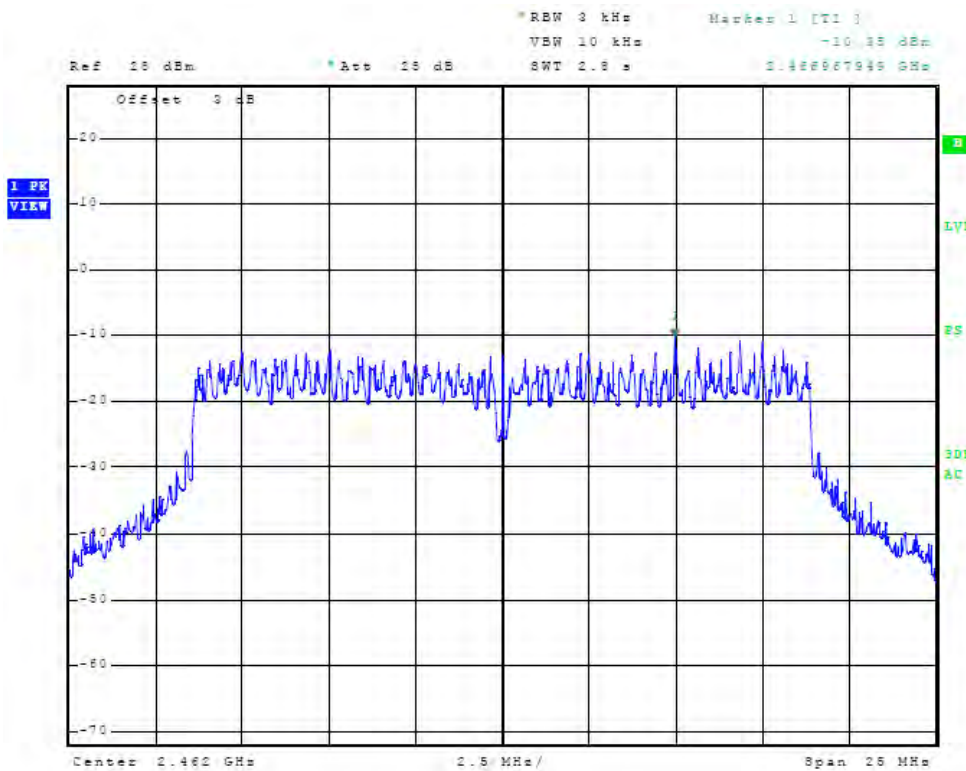
Figure 88 Plot of Antenna Port Conducted Power Spectral Density (chain2, 2462 MHz, 20 MHz Mode)
