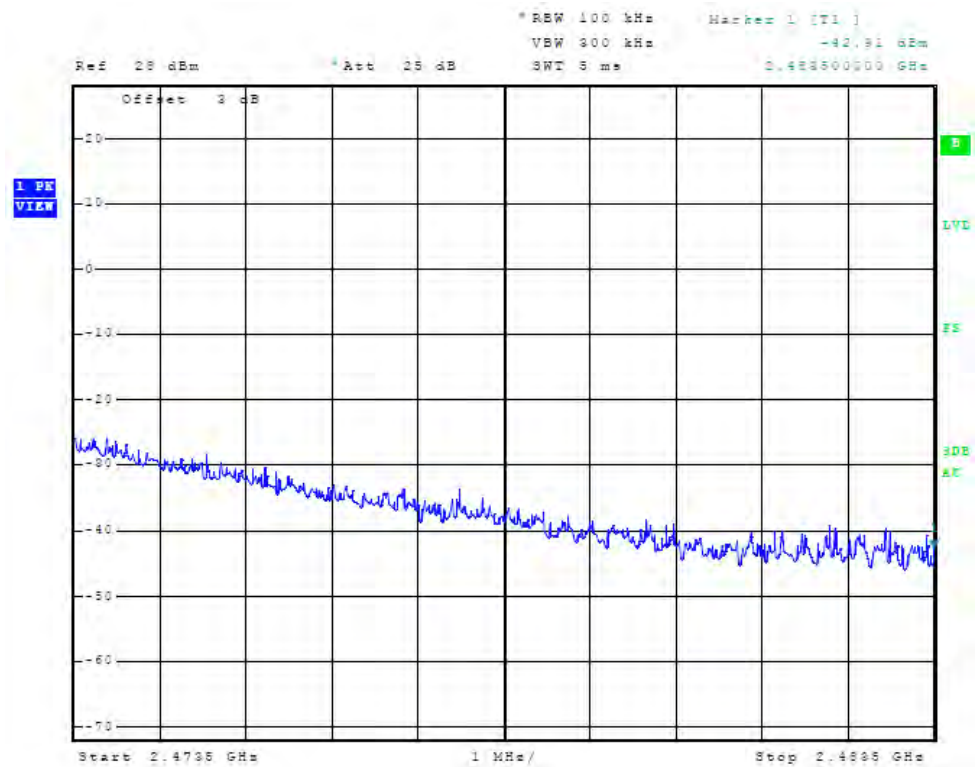
Figure 98 Plot of High Band Edge Compliance at Antenna Port (chain2, 2.4MHz Operation)
