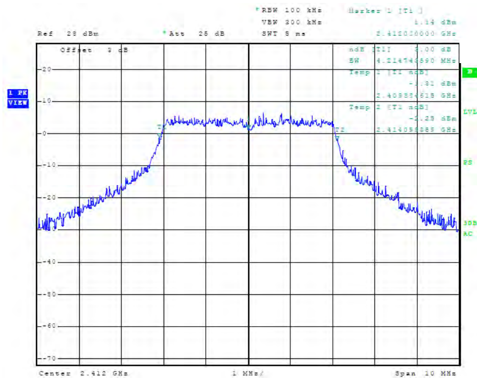
Figure 74 Plot of Antenna Port Conducted 6dB Band width (chain2, 2412 MHz, 5 MHz Mode)
