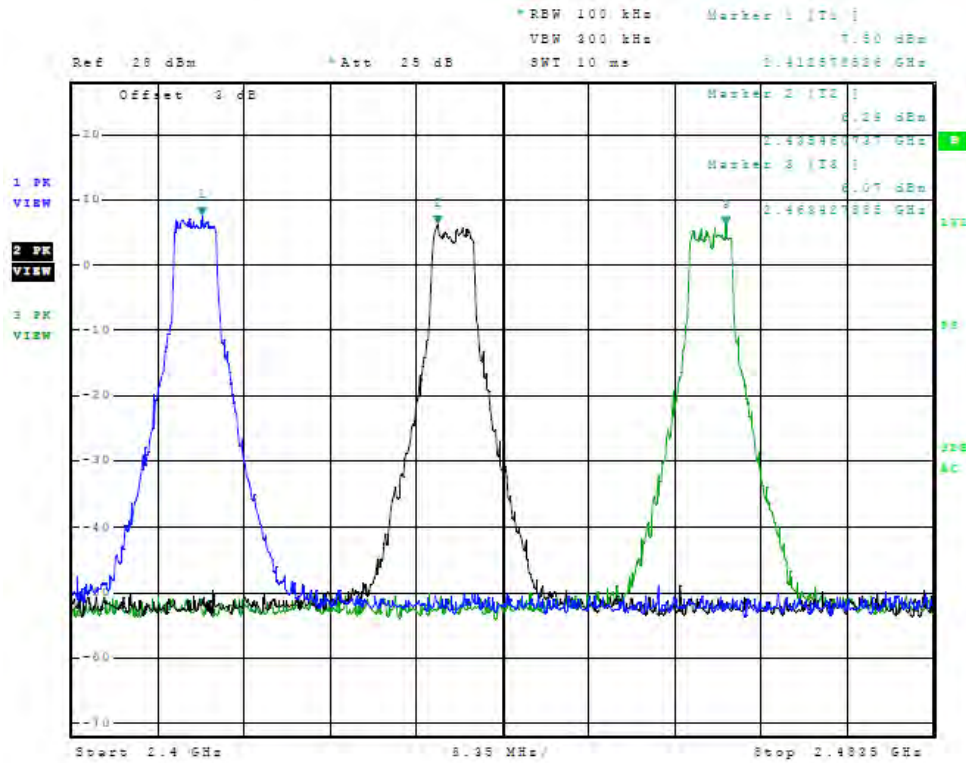
Figure 71 Plot of Antenna Port Conducted (2GHz, chain2, Operational Band, 5MHz Mode)
