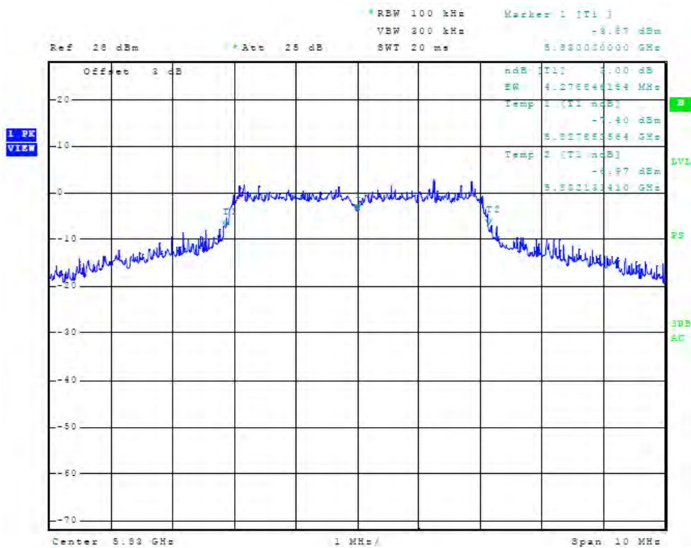
Figure 104 Plot of Antenna Port Conducted 6dB Band width (chain2, 5830 MHz, 5 MHz Mode)
