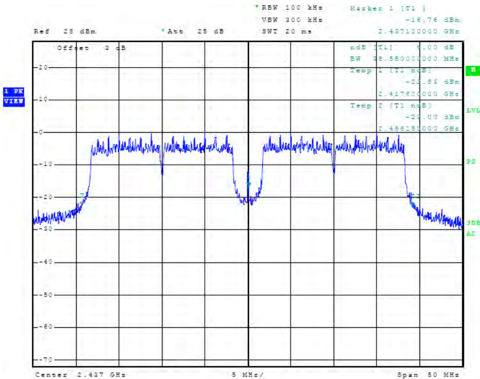
Figure 22 Plot of Antenna Port Conducted 6dB Band width (chain1, 2437 MHz, 40 MHz Mode)
