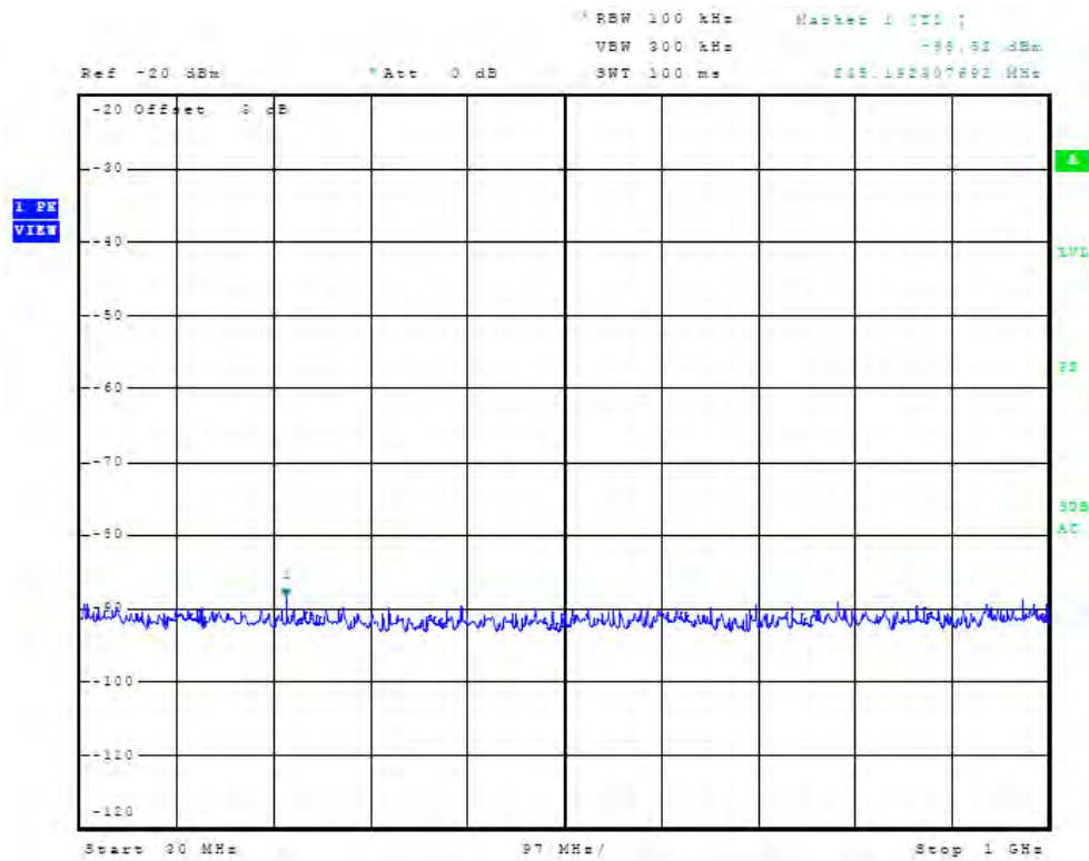
Figure 131 Plot of Receiver Antenna Port Conducted Emissions
