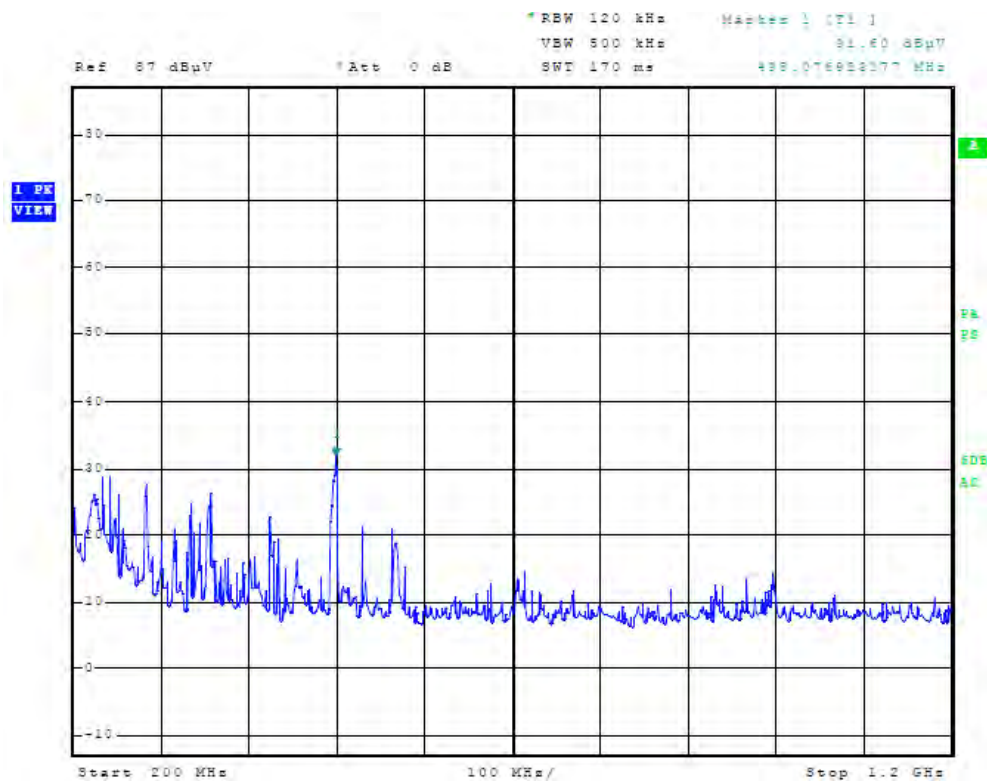
Figure 138 Plot of Receiver Radiated Spurious Emissions taken at 1 meter
