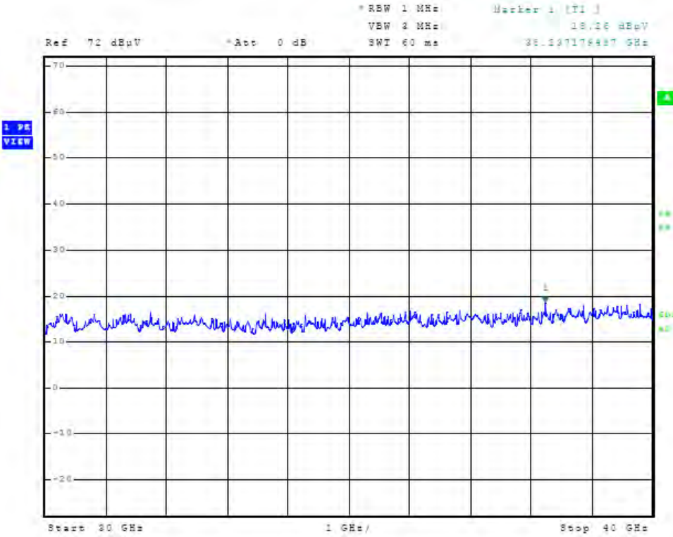
Figure 11 General Radiated Emissions taken at 1 meter in screen room
