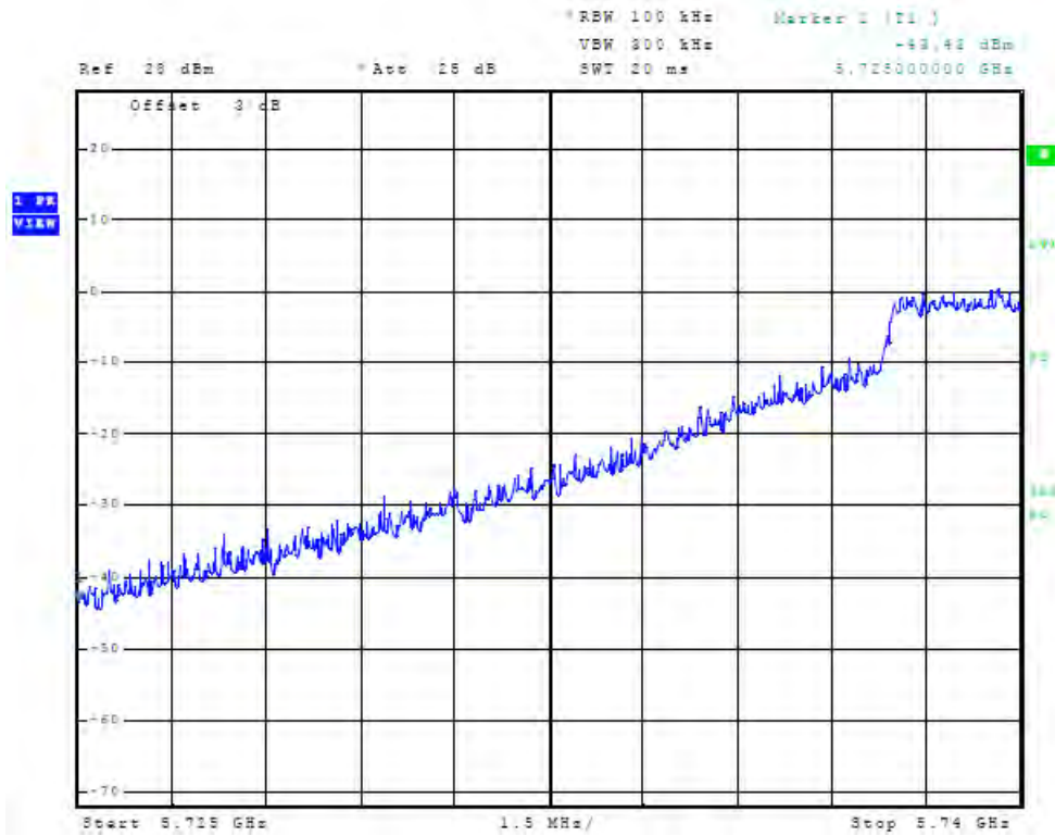
Figure 69 Plot of Antenna Port Conducted Low Band Edge Compliance (5 GHz, chain1, operation)
