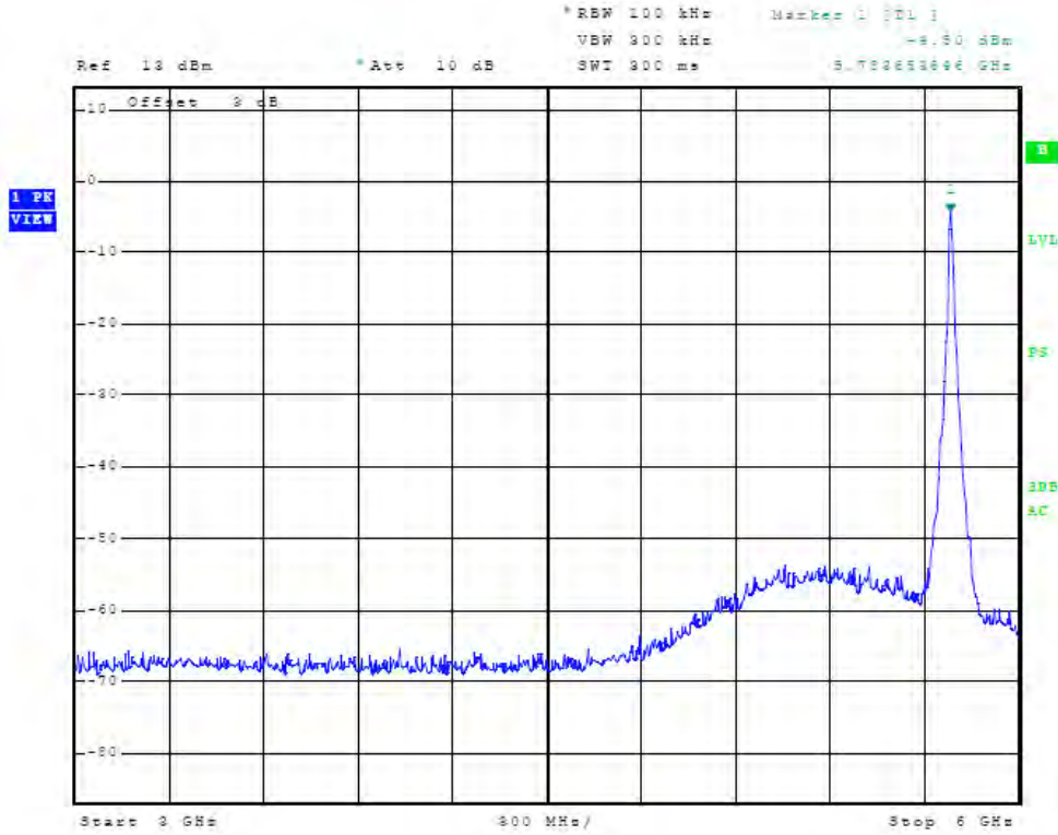
Figure 63 Plot of Antenna Port Conducted Emissions (5 GHz, chain 1, operation)
