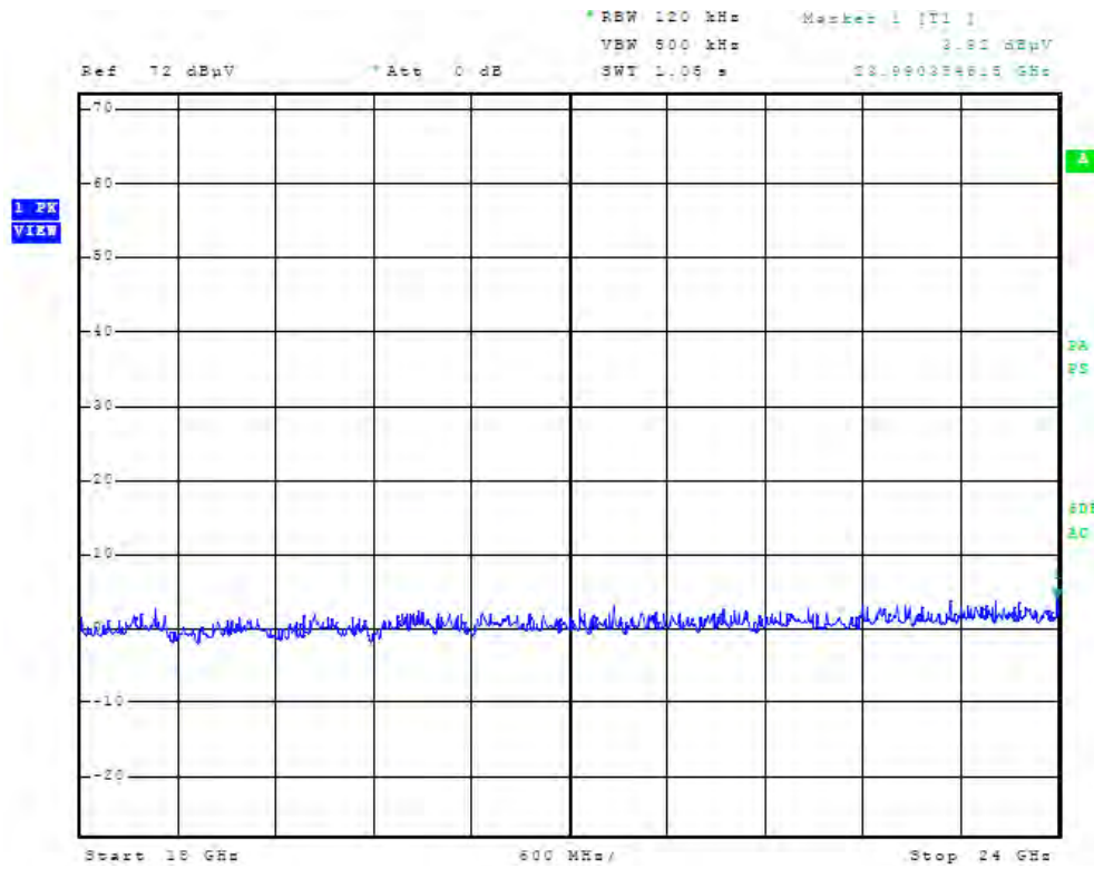
Figure 143 Plot of Receiver Radiated Spurious Emissions taken at 1 meter
