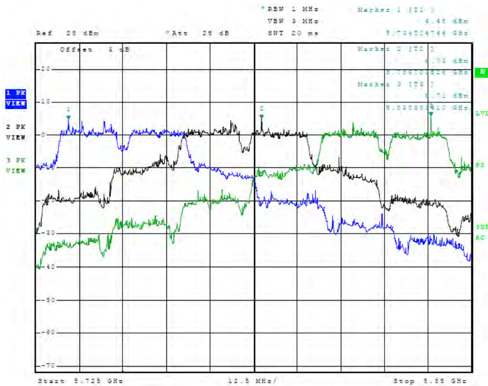
Figure 42 Plot of Antenna Port Conducted (5GHz, chain1, Operational Band, 40MHz Mode)
