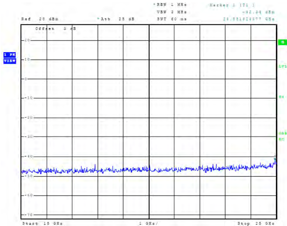
Figure 96 Plot of Antenna Port Conducted Emissions (chain2, 2.4MHz Operation)
