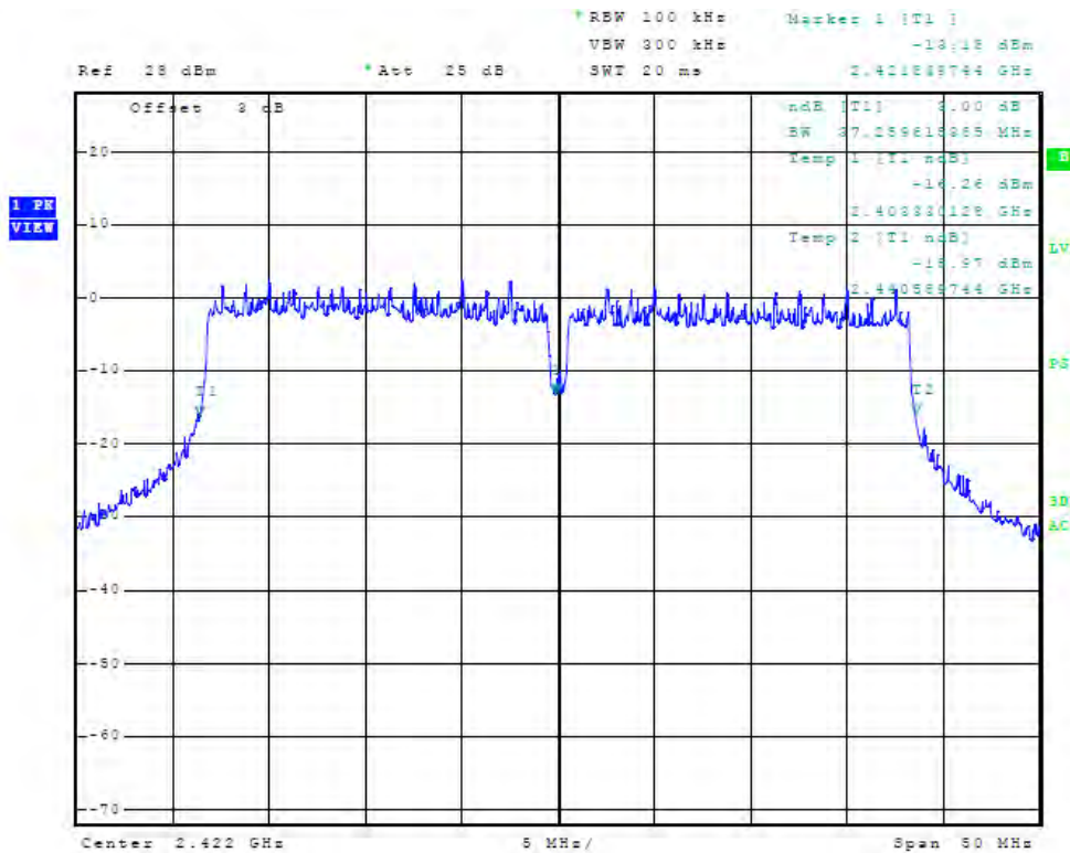
Figure 80 Plot of Antenna Port Conducted 6dB Band width (chain2, 2422 MHz, 40 MHz Mode)
