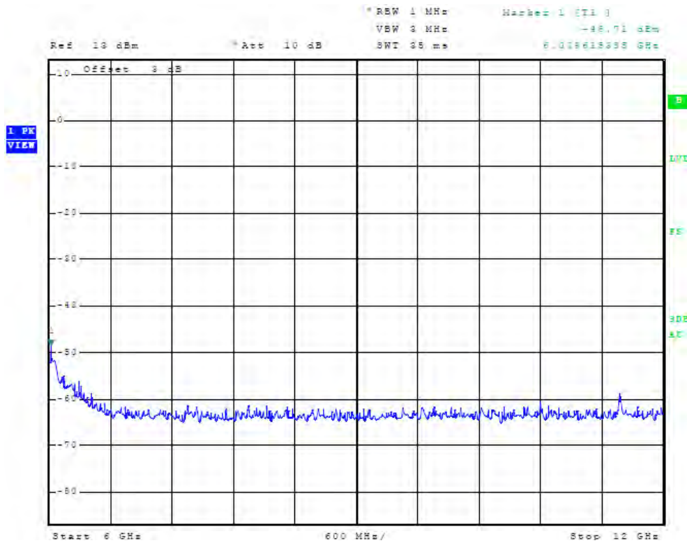
Figure 64 Plot of Antenna Port Conducted Emissions (5 GHz, chain 1, operation)
