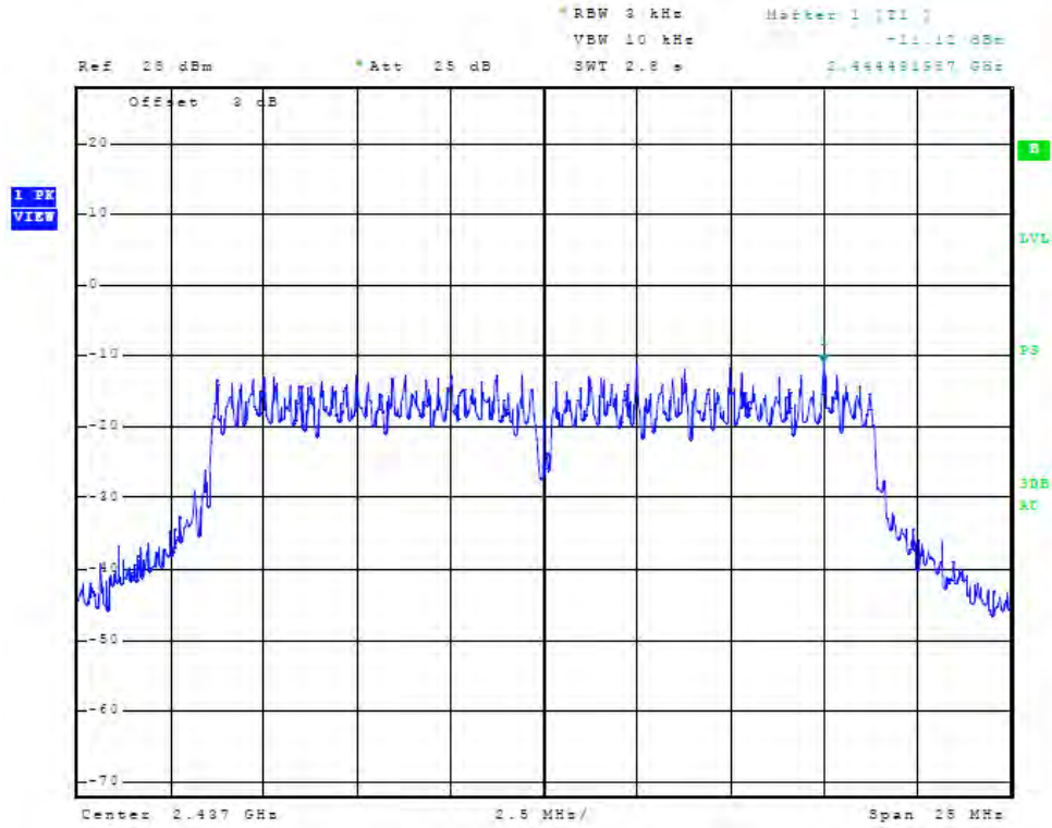
Figure 87 Plot of Antenna Port Conducted Power Spectral Density (chain2, 2437 MHz, 20 MHz Mode)
