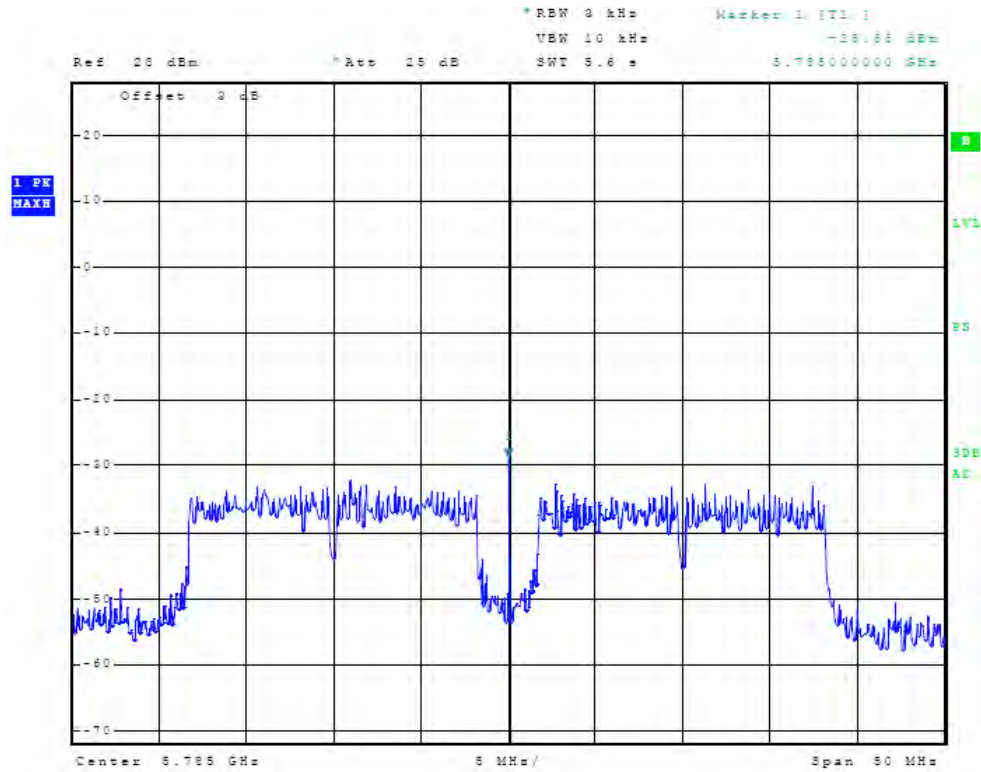
Figure 59 Plot of Antenna Port Conducted Power Spectral Density (chain 1, 5785 GHz, 40MHz Mode)
