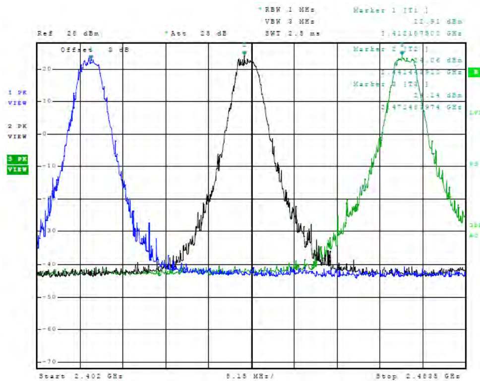
Figure 12 Plot of Antenna Port Conducted (2 GHz, chain1, Operational Band, 5MHz Mode)
