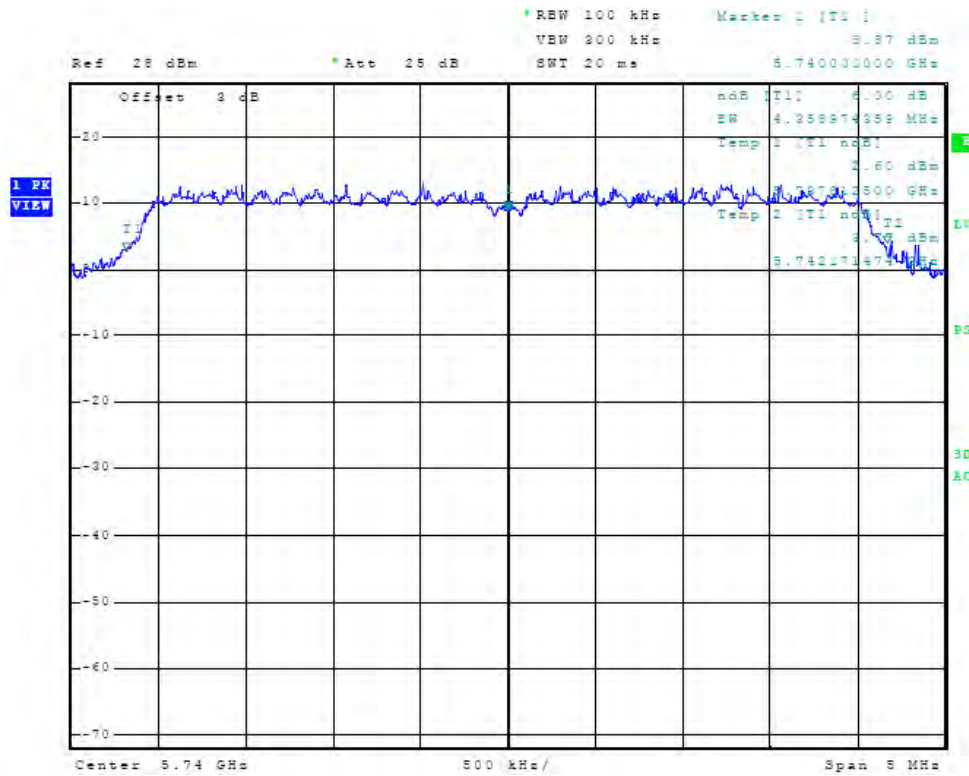
Figure 43 Plot of Antenna Port Conducted 6dB Band width (chain 1, 5740 MHz, 5 MHz Mode)
