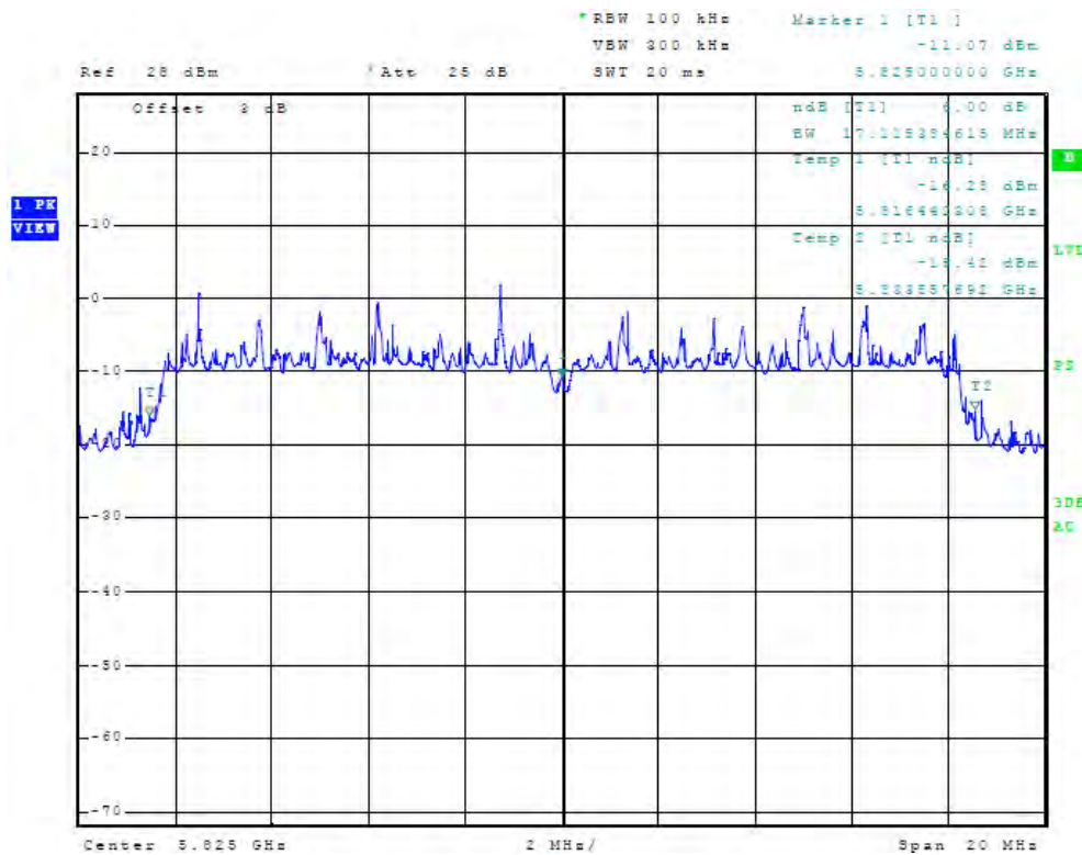
Figure 48 Plot of Antenna Port Conducted 6dB Band width (chain 1, 5825 MHz, 20 MHz Mode)
