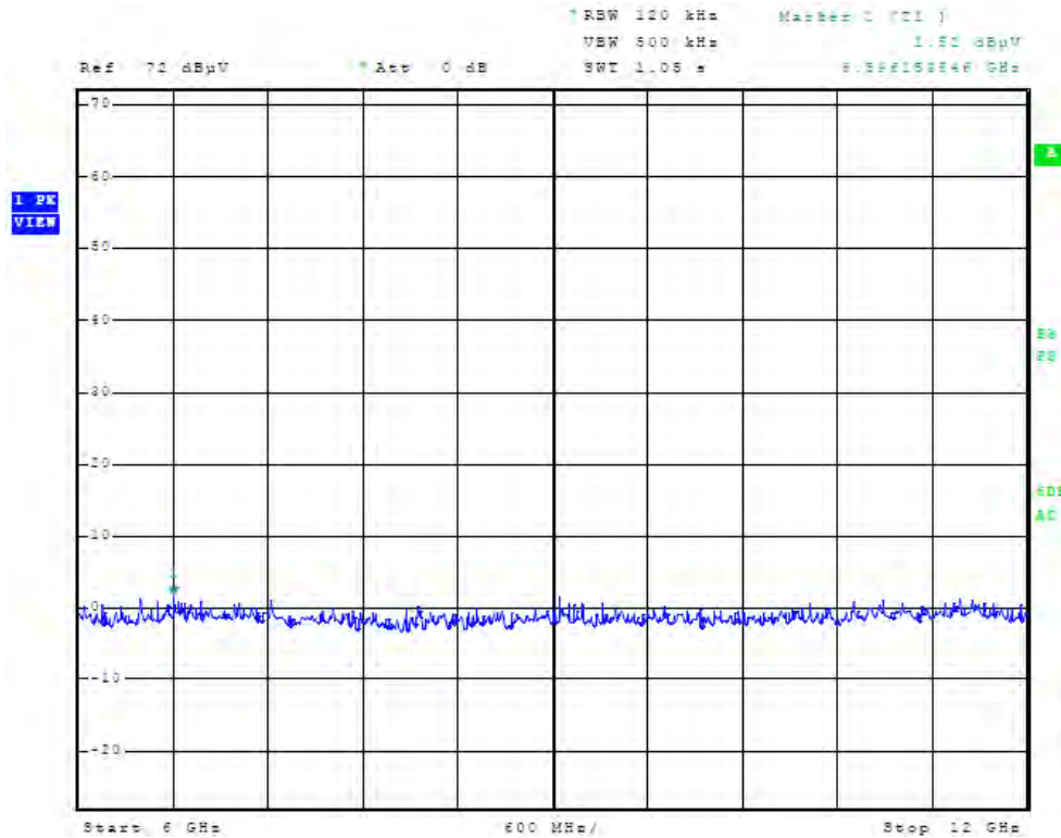
Figure 141 Plot of Receiver Radiated Spurious Emissions taken at 1 meter
