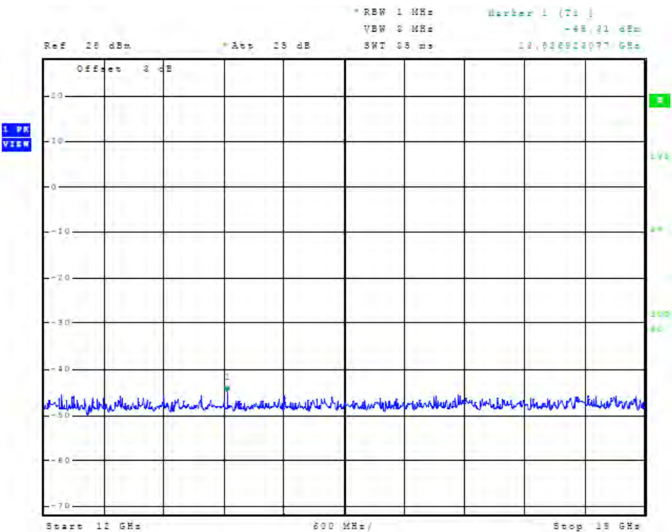
Figure 124 Plot of Antenna Port Conducted Emissions (5 GHz chain2, operation)
