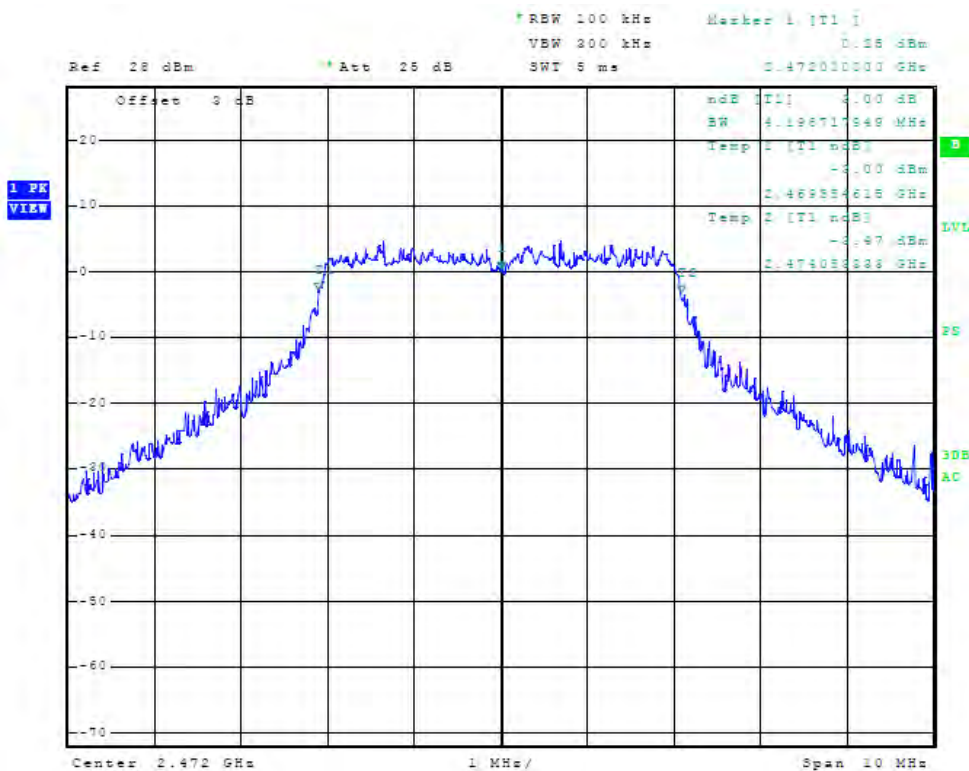
Figure 76 Plot of Antenna Port Conducted 6dB Band width (chain2, 2472 MHz, 5 MHz Mode)
