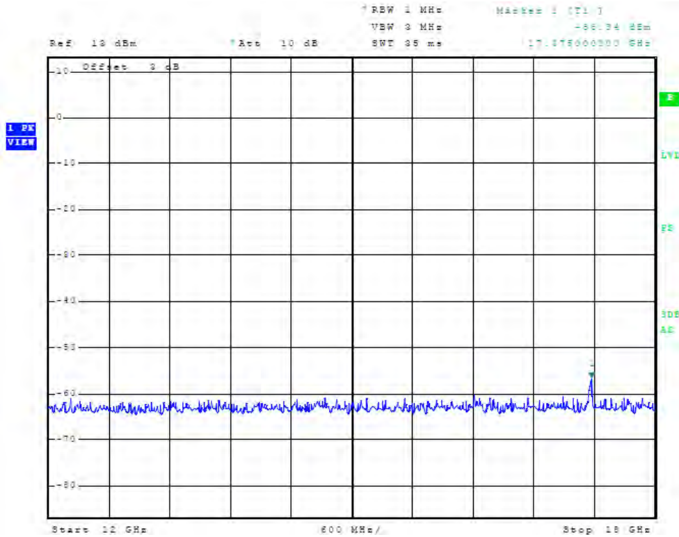
Figure 65 Plot of Antenna Port Conducted Emissions (5 GHz, chain 1, operation)
