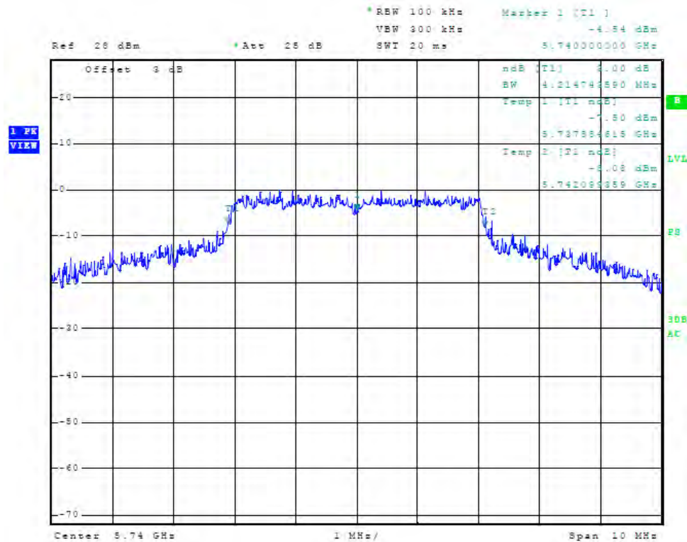
Figure 102 Plot of Antenna Port Conducted 6dB Band width (chain2, 5740 MHz, 5 MHz Mode)
