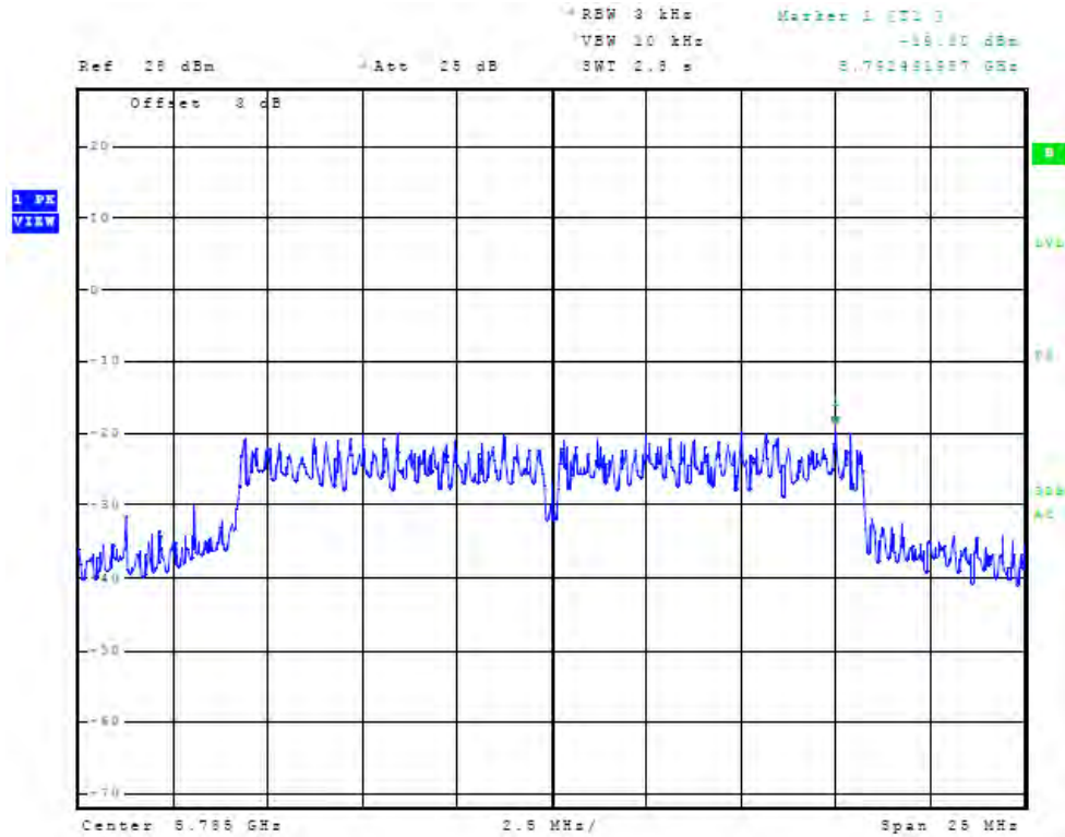
Figure 115 Plot of Antenna Port Conducted Power Spectral Density (chain2, 5785 GHz, 20MHz Mode)
