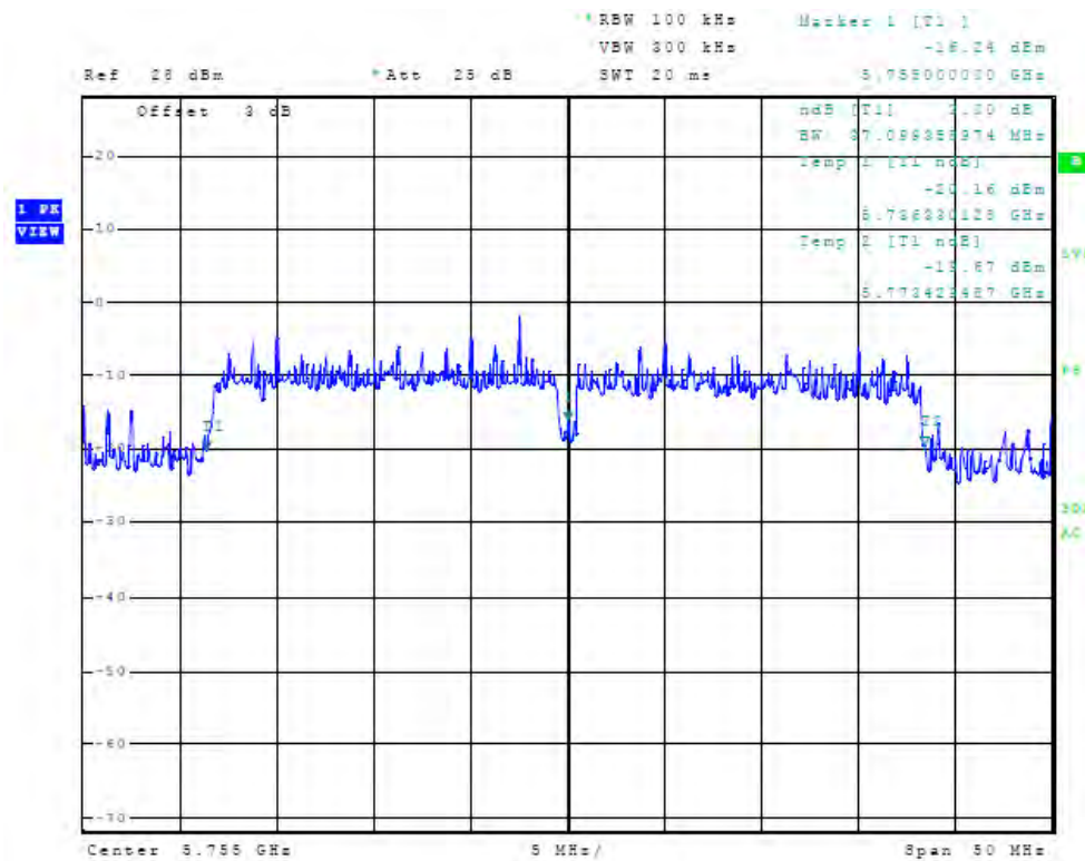
Figure 108 Plot of Antenna Port Conducted 6dB Band width (chain2, 5755 MHz, 40 MHz Mode)
