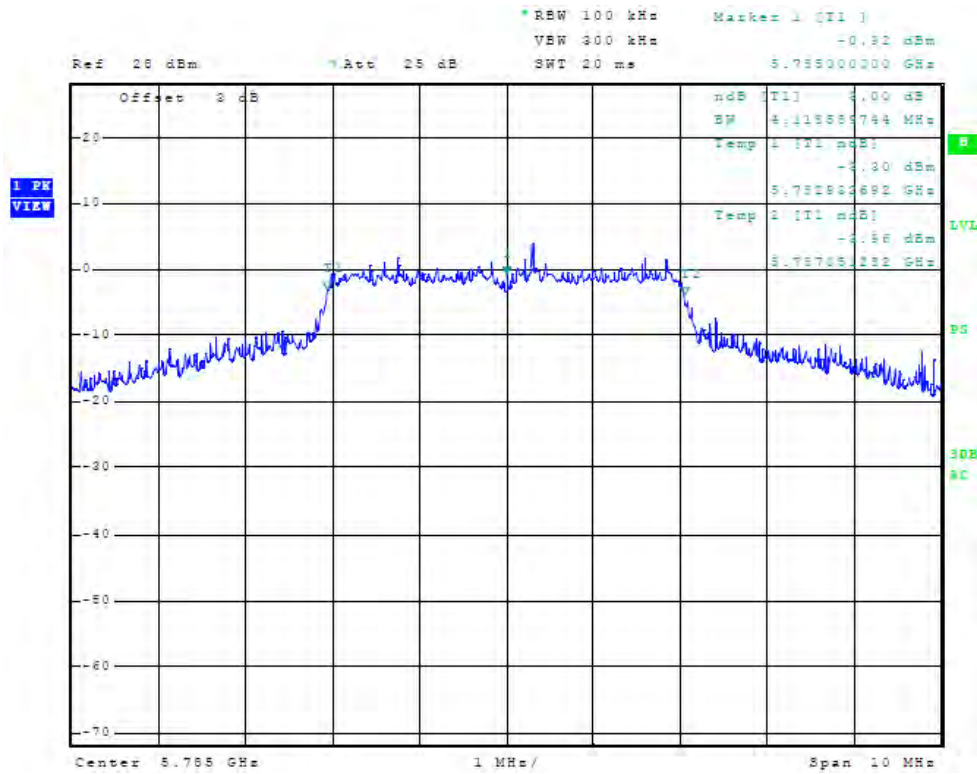
Figure 103 Plot of Antenna Port Conducted 6dB Band width (chain2, 5785 MHz, 5 MHz Mode)
