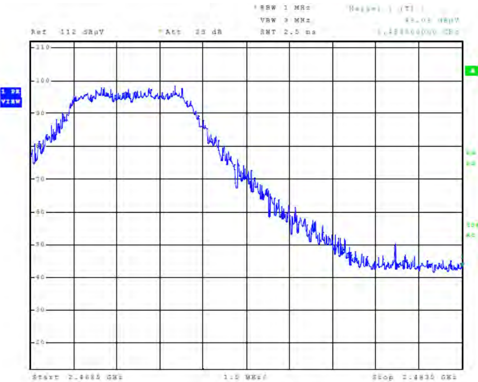
Figure 130 Plot of Radiated Emissions at High Band Edge
