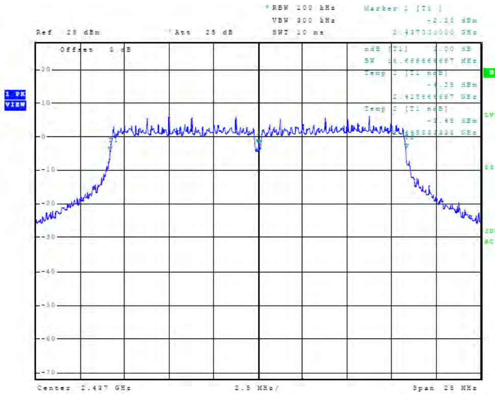
Figure 19 Plot of Antenna Port Conducted 6dB Band width (chain1, 2437 MHz, 20 MHz Mode,)
