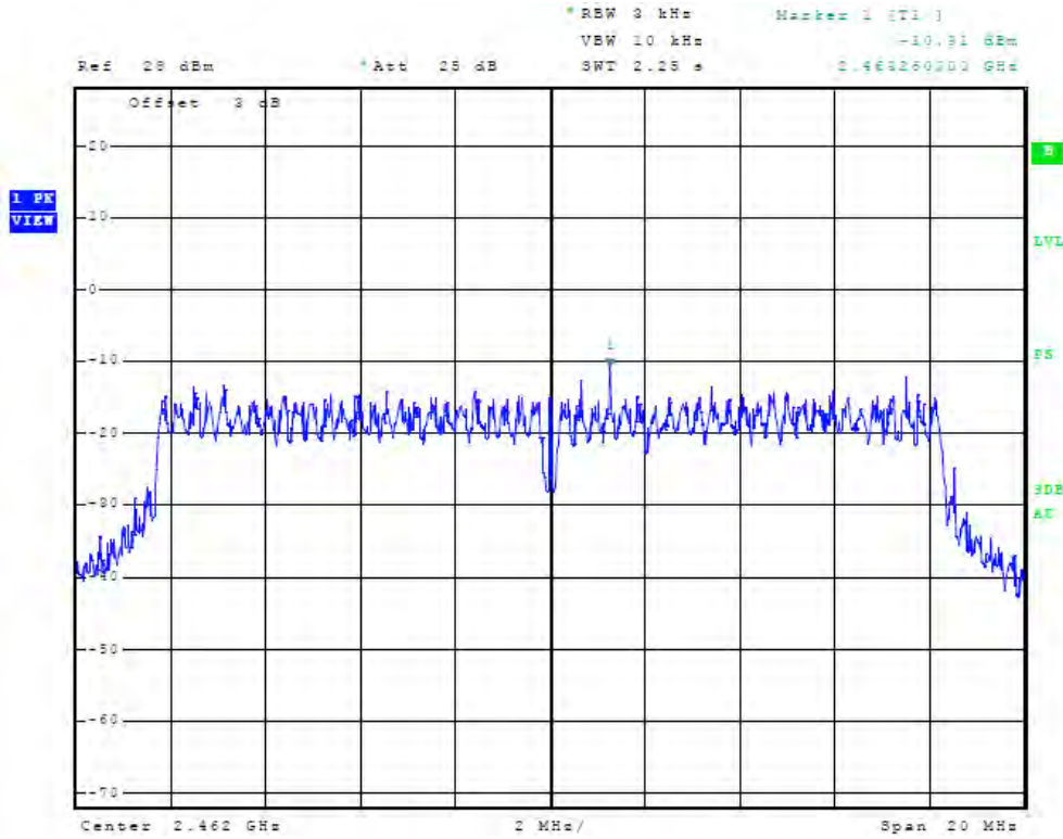
Figure 29 Plot of Antenna Port Conducted Power Spectral Density (chain1, 2462 MHz, 20 MHz Mode)
