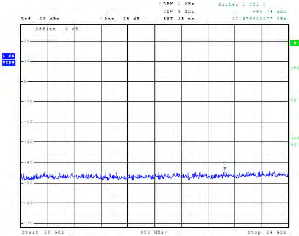
Figure 125 Plot of Antenna Port Conducted Emissions (5 GHz chain2, operation)
