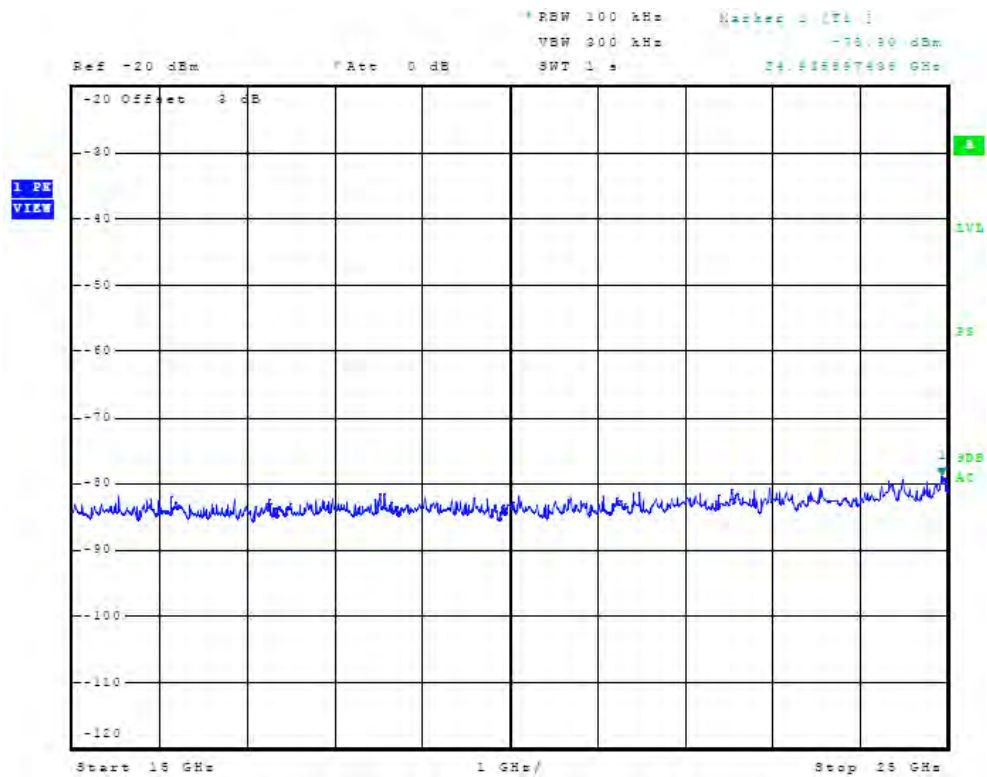
Figure 136 Plot of Receiver Antenna Port Conducted Emissions
