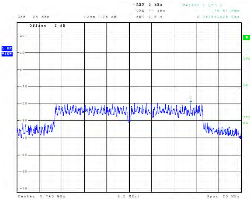
Figure 114 Plot of Antenna Port Conducted Power Spectral Density (chain2, 5745 GHz, 20MHz Mode)
