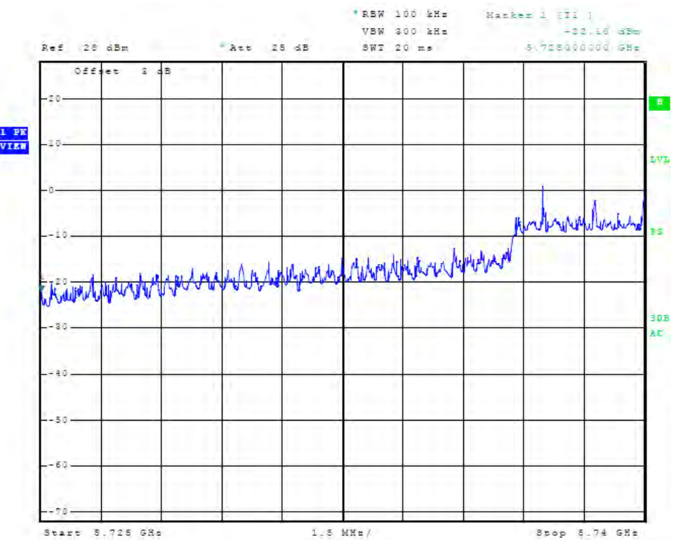
Figure 128 Plot of Antenna Port Conducted Low Band Edge Compliance (5 GHz chain2, operation)
