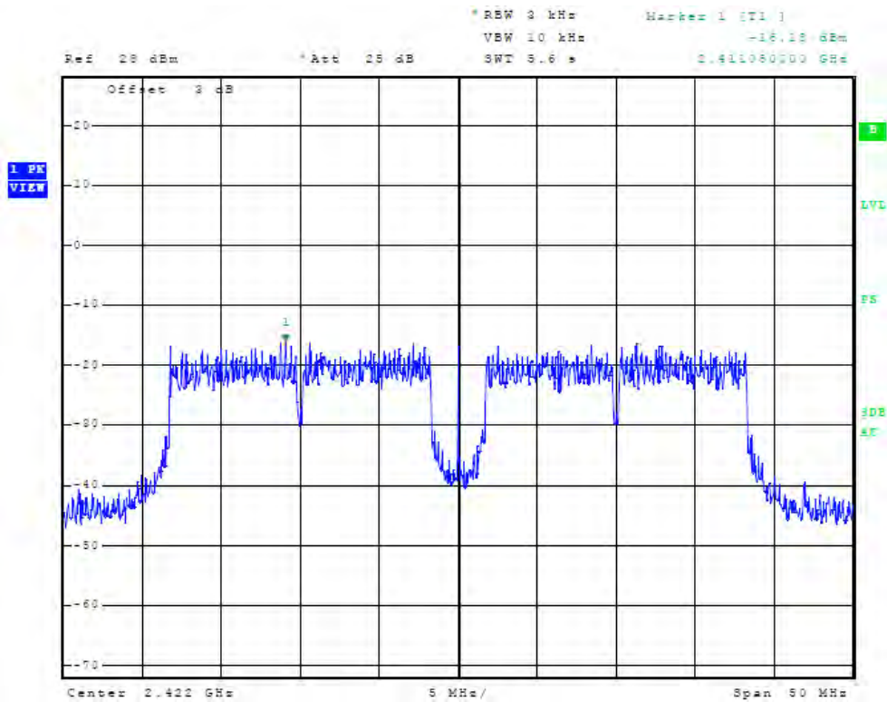
Figure 30 Plot of Antenna Port Conducted Power Spectral Density (chain1, 2422 MHz, 40 MHz Mode)
