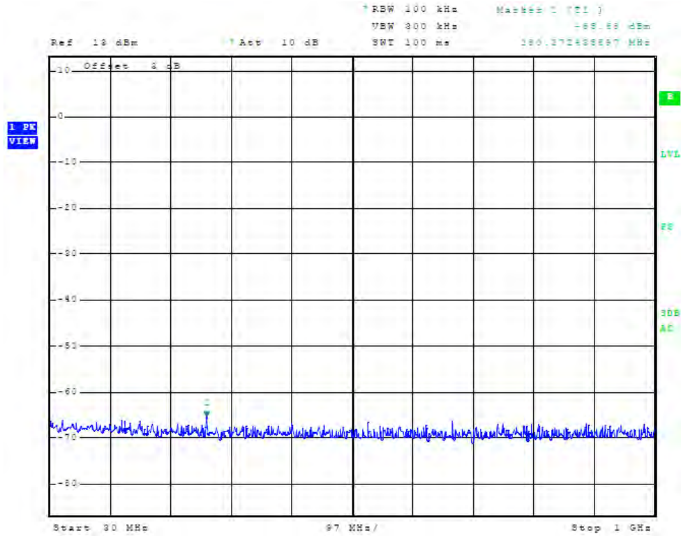
Figure 61 Plot of Antenna Port Conducted Emissions (5 GHz, chain 1, operation)
