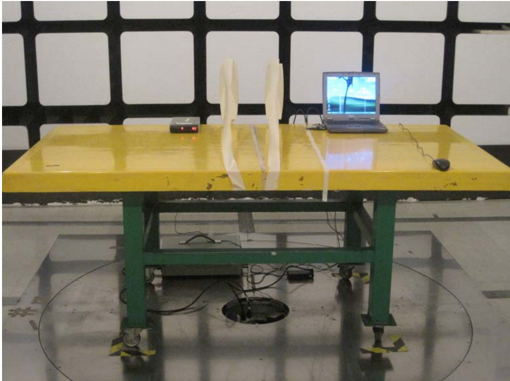
Transmitter Radiated Spurious Emissions (Below 1GHz)
