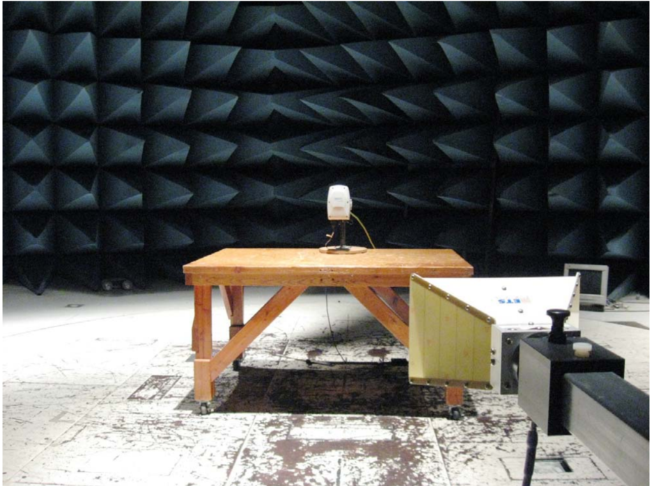
Radiated Emission Limits Test Setup 1 - 5GHz
