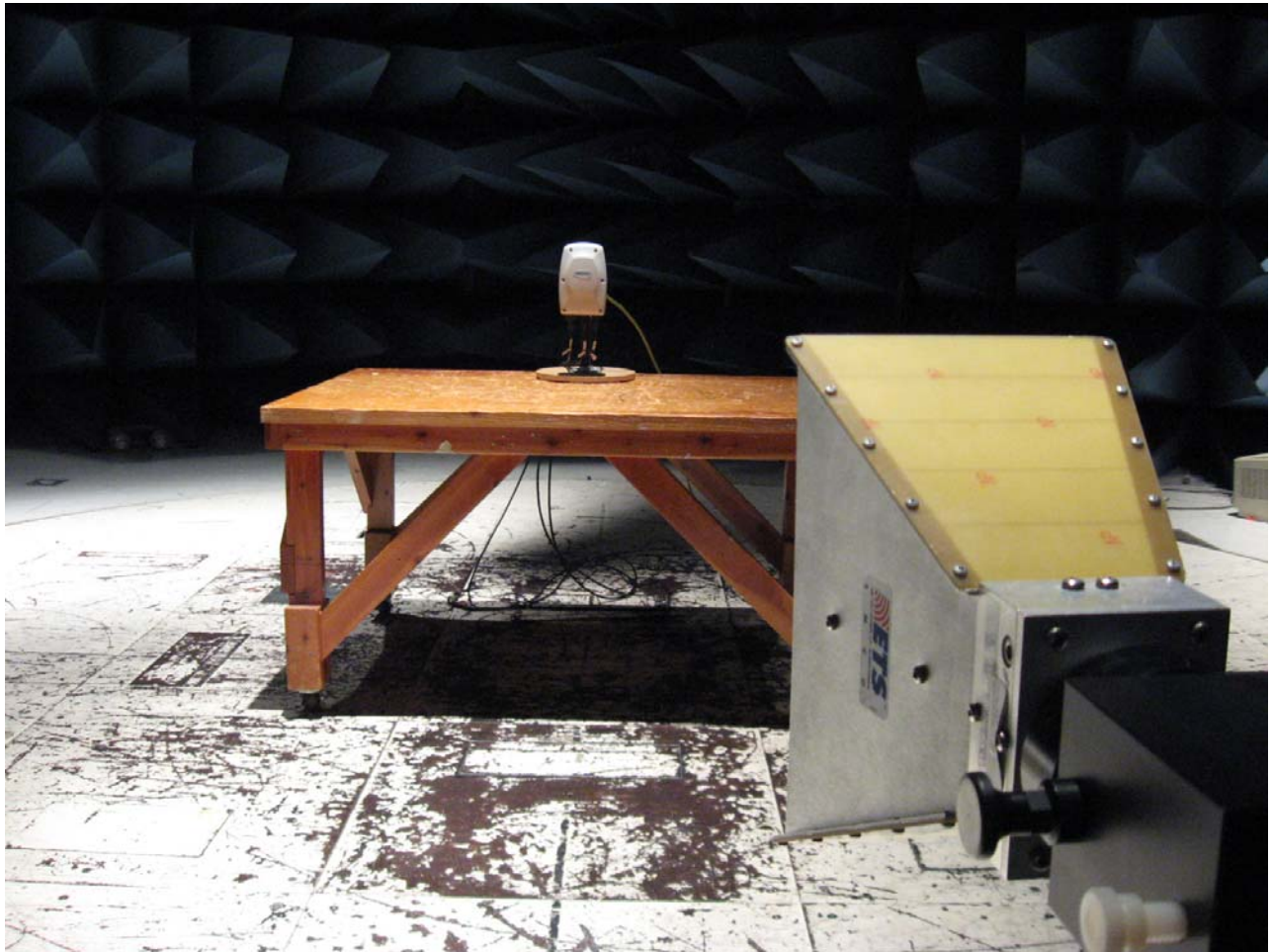
Test Equipment and setup for various Radiated Measurements (Integrated Antenna)
