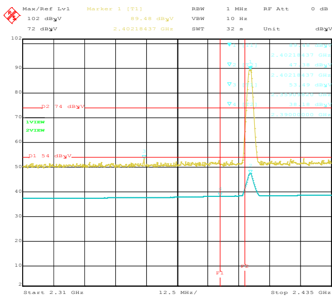
Title: RDS7. Comment A: Lower Band Edge-Horizontal. Date: 5.MAR.2013 12:25:47
