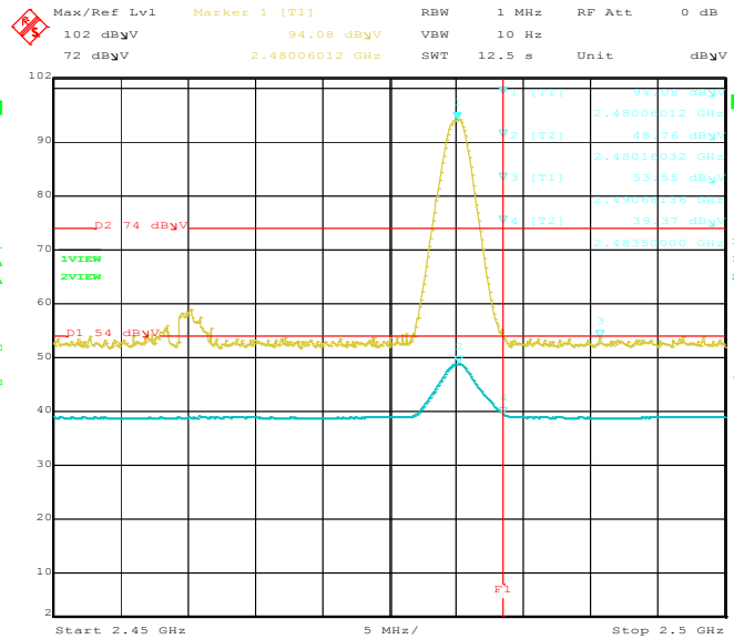
Title: RDS7. Comment A: Upper Band Edge-Horizontal. Date: 5.MAR.2013 12:35:53
