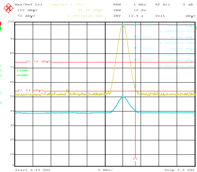
Title: RDS7. Comment A: Upper Band Edge-Vertical. Date: 5.MAR.2013 13:32:12
