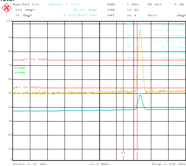
Title: RDS7. Comment A: Lower Band Edge-Vertical Date: 5.MAR.2013 12:22:44
