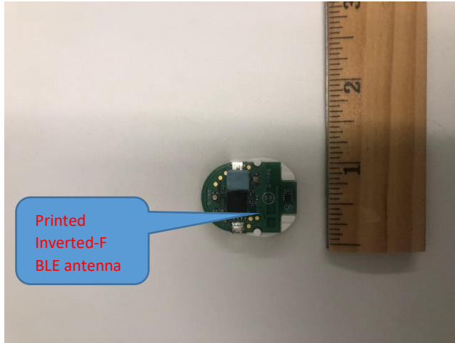
Figure 1: Top Layer of DR-301317 Showing Inverted-F Antenna
