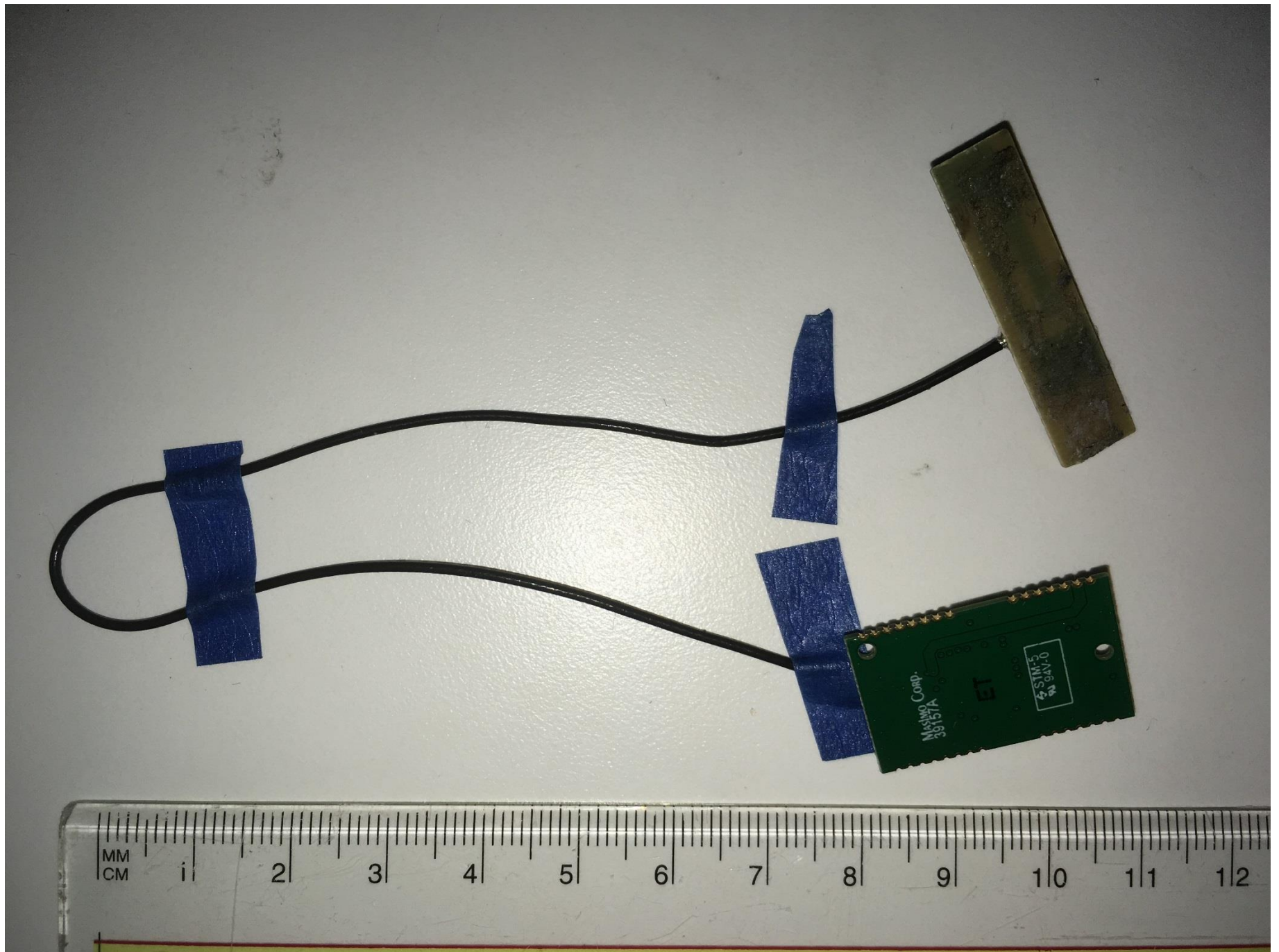
Figure 2: Rear view of MWMII with antenna (P/N: 1000672)
