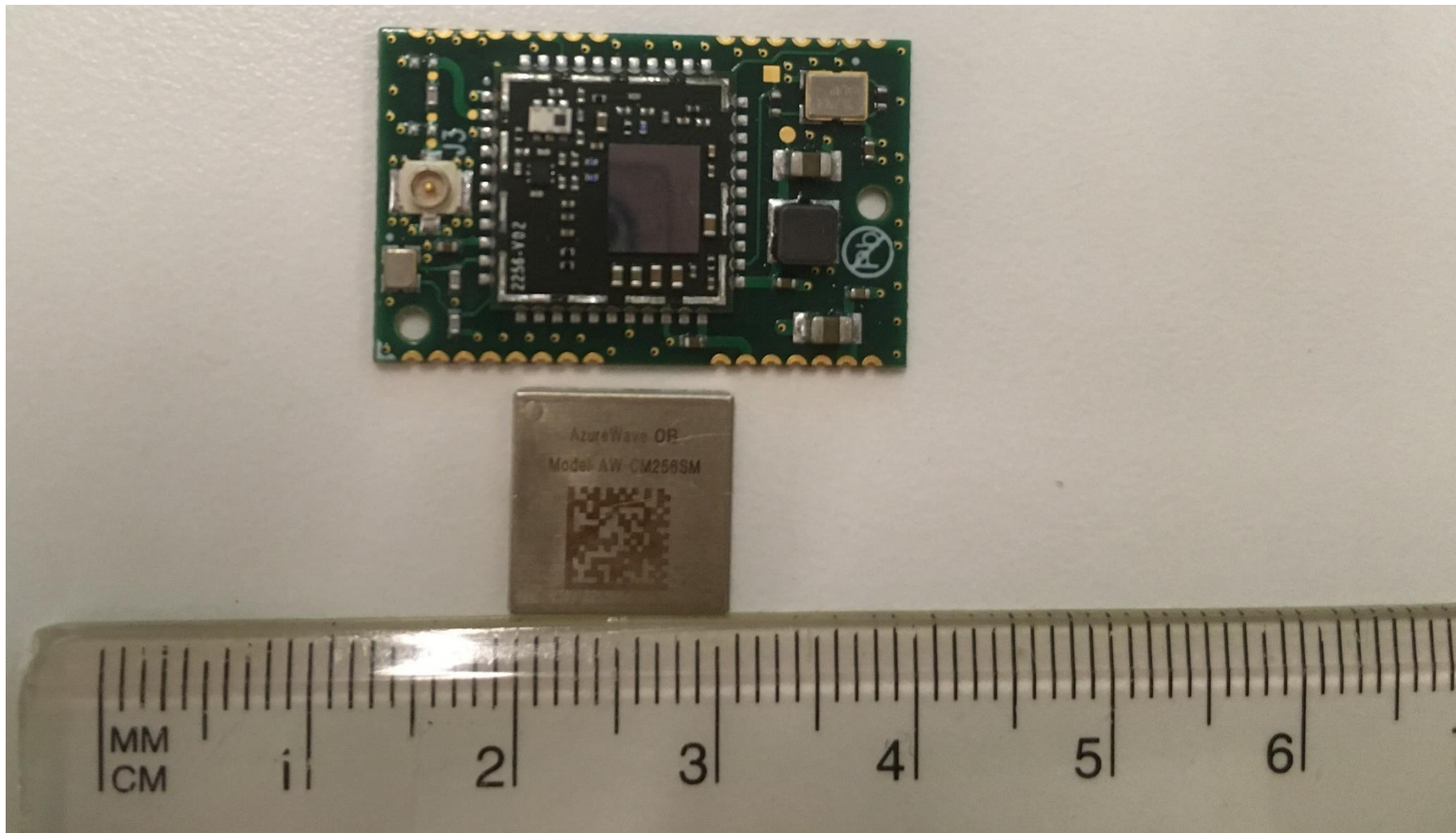
Figure 5: Radio module with the shield removed
