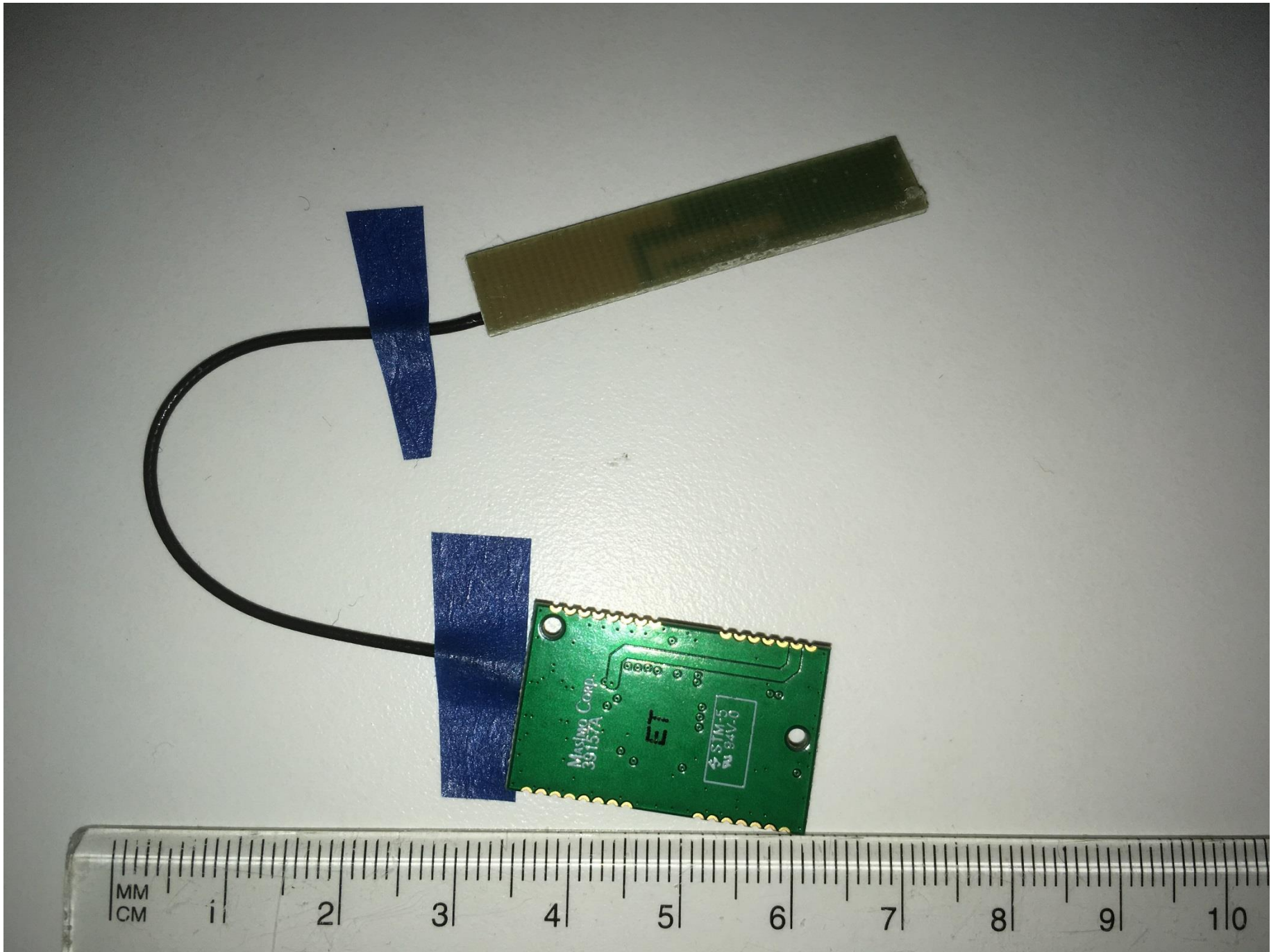
Figure 4: Rear view of MWMII with antenna (P/N 9000129)
