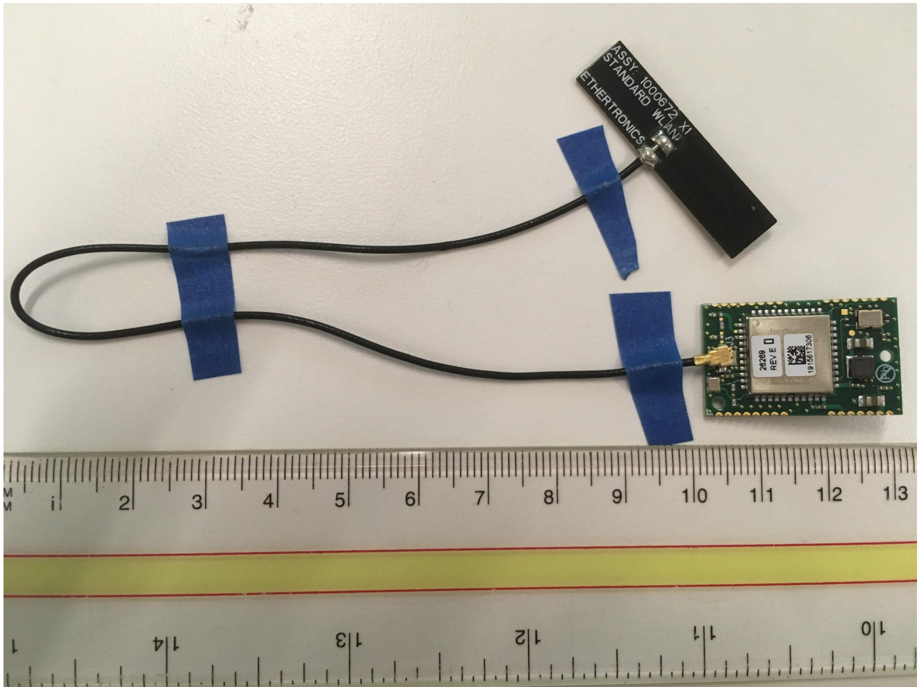
Figure 1: Front view of MWMII with antenna (P/N: 1000672)
