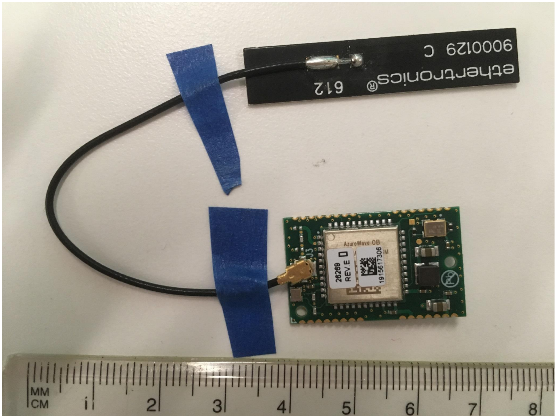
Figure 3: Front view of MWMII with antenna (P/N 9000129)
