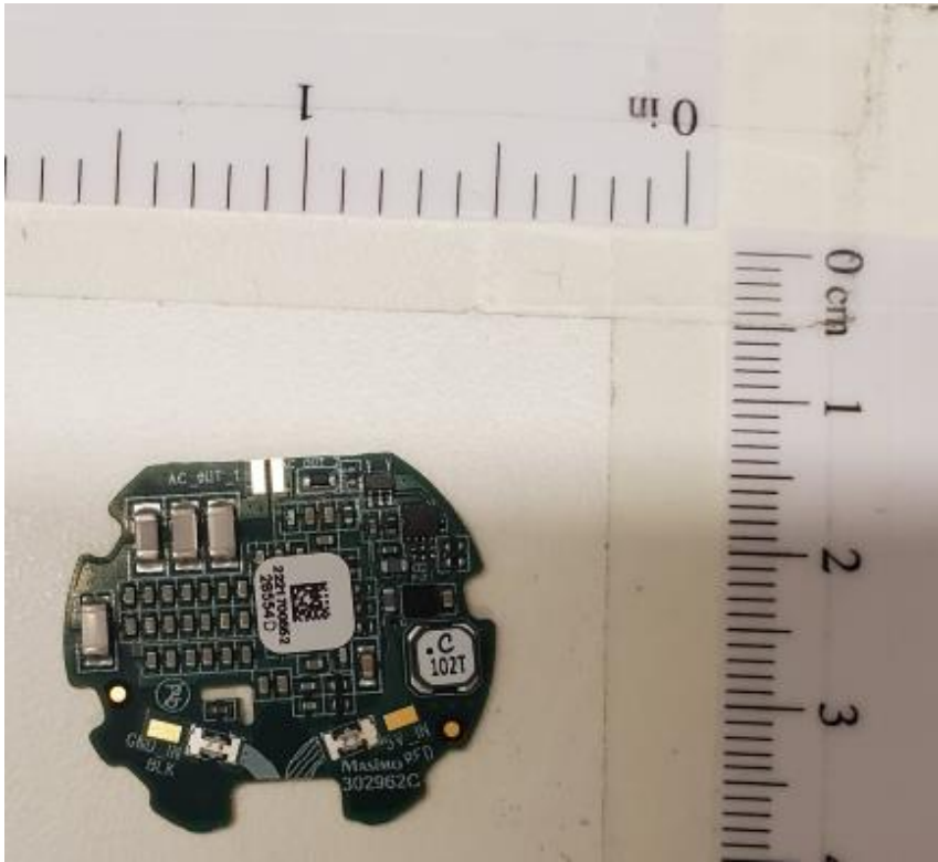
Photo 8: PCB- back view
