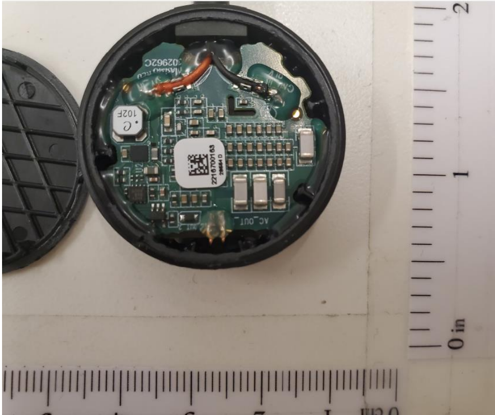
Photo 4: Wireless Charger opened in below picture and bottom view
