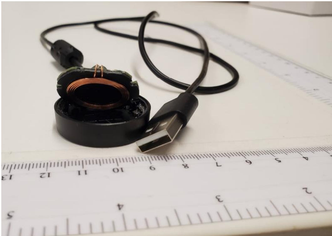
Photo 4: Wireless Charger opened in below picture and bottom view
