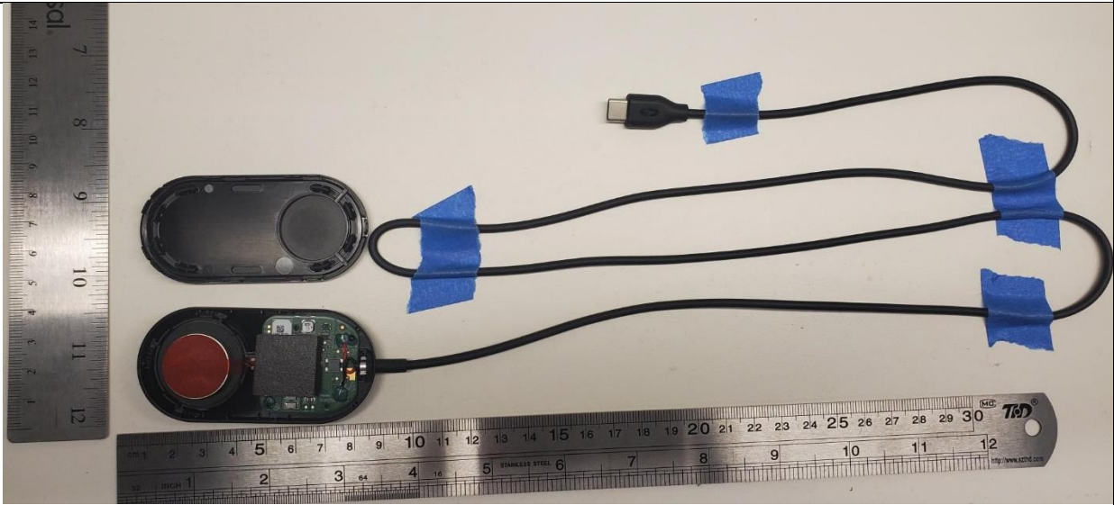
Internal view of Masimo Wireless Charger with the cover open
