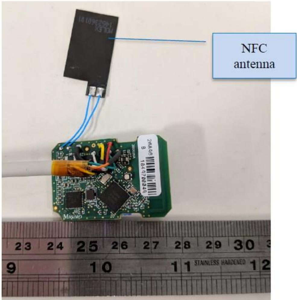
Radius PPG Receiver with NFC antenna
