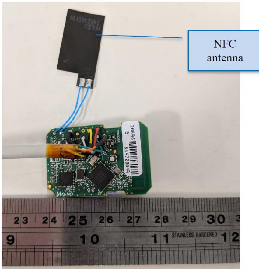
Figure 1: NFC antenna location in Receiver housing
