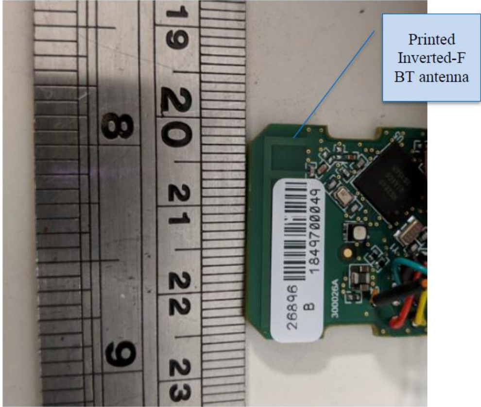
Figure 2: Top Layer of DR-300026 Showing Printed Inverted-F Antenna
