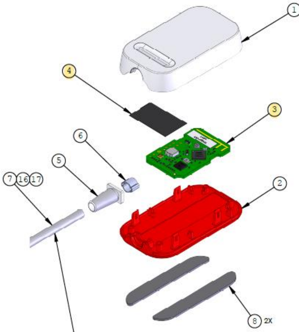
Figure 3: Assembly drawing of Radius PPG wireless receiver showing item # 3 that is Bluetooth antenna and item #4 is NFC antenna, both of these are enclosed in the outer housing indicated by item #1. Both the antennas are permanently attached and are non-replaceable.
