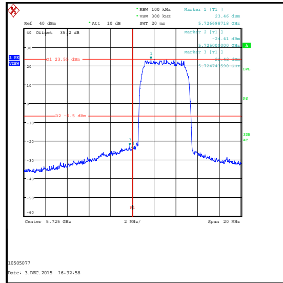
32QAM
