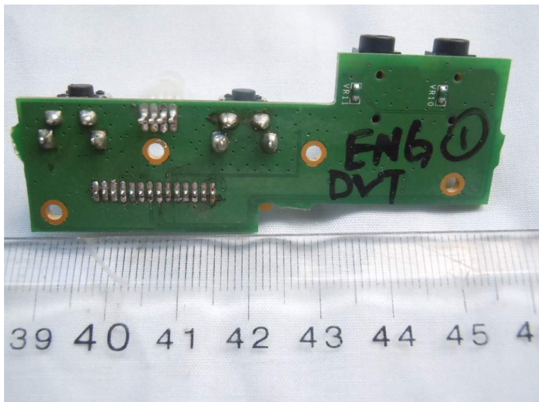
FIGURE 12 WIRELESS AIRPLAY SPEAKER (M/N: MA5000) BUTTON BOARD #1 (SOLDERED SIDE)
