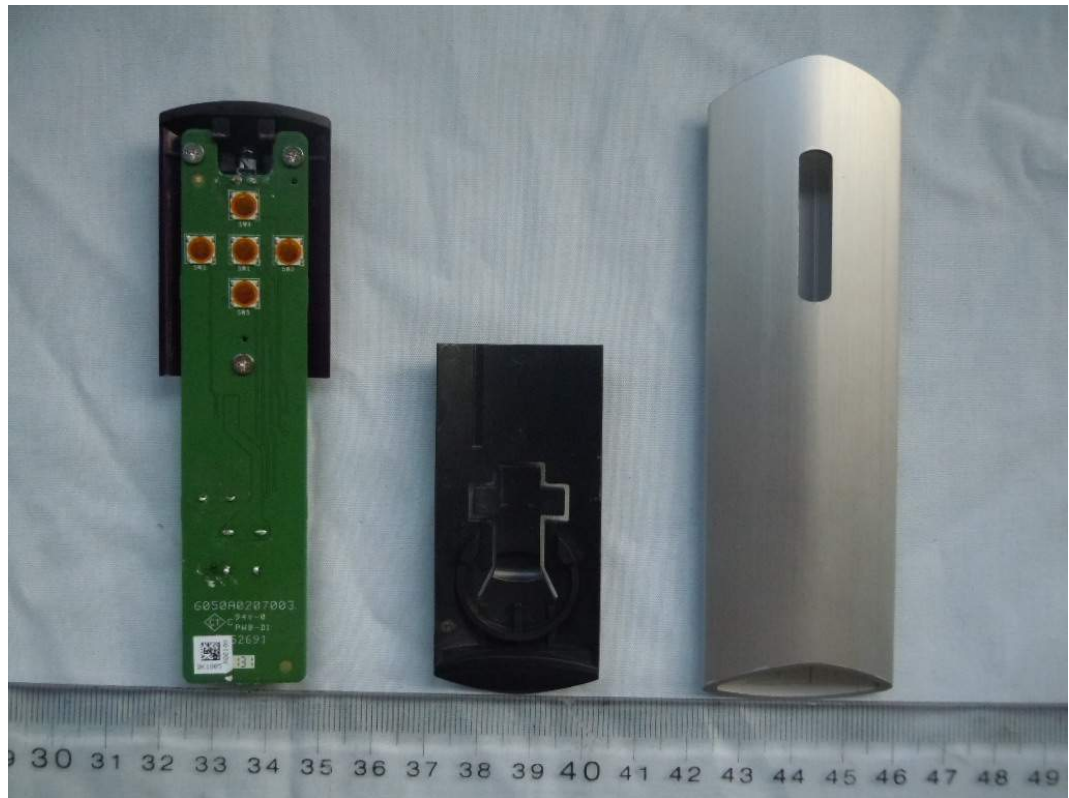
FIGURE 20 WIRELESS AIRPLAY SPEAKER (M/N: MA5000) CONTROLLER (COVER REMOVED)
