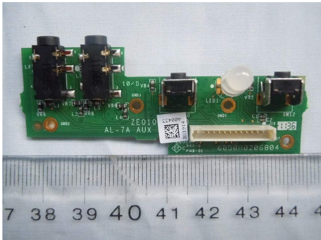
FIGURE 11 WIRELESS AIRPLAY SPEAKER (M/N: MA5000) BUTTON BOARD #1 (COMPONENT SIDE)
