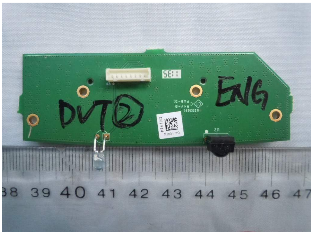
FIGURE 14 WIRELESS AIRPLAY SPEAKER (M/N: MA5000) BUTTON BOARD #2 (SOLDERED SIDE)
