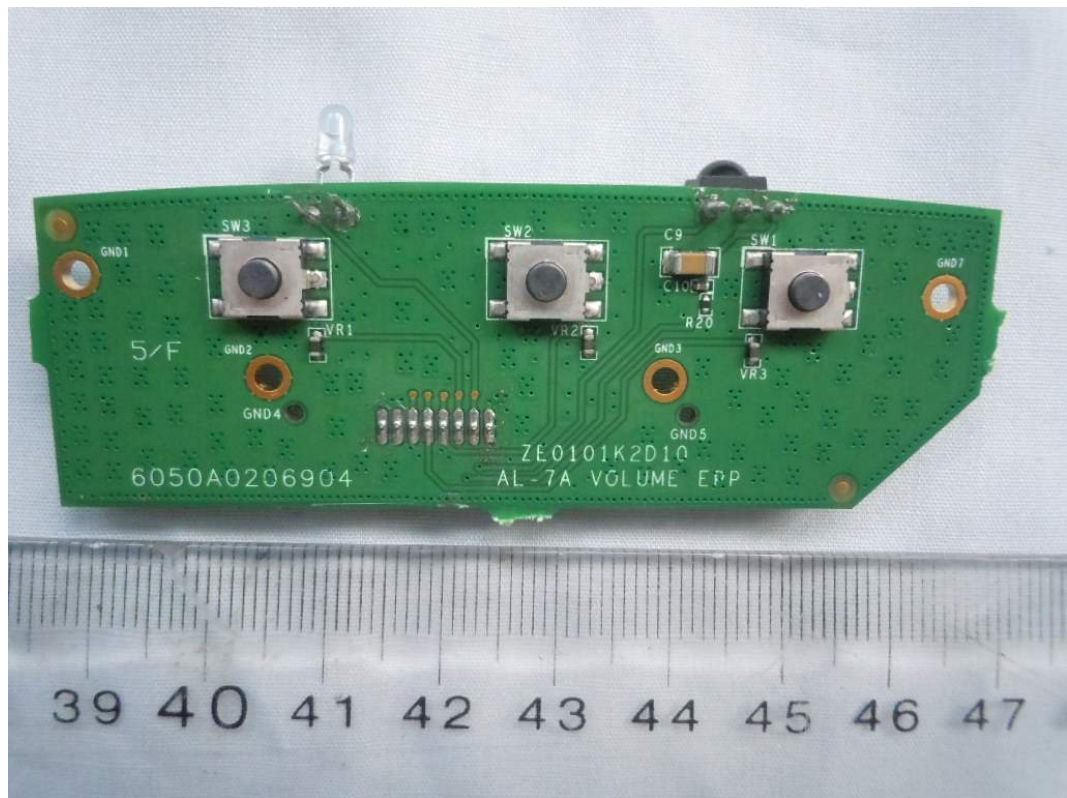
FIGURE 13 WIRELESS AIRPLAY SPEAKER (M/N: MA5000) BUTTON BOARD #2 (COMPONENT SIDE)
