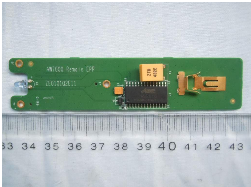
FIGURE 22 WIRELESS AIRPLAY SPEAKER (M/N: MA5000) CONTROLLER (BOARD – SOLDERED SIDE)
