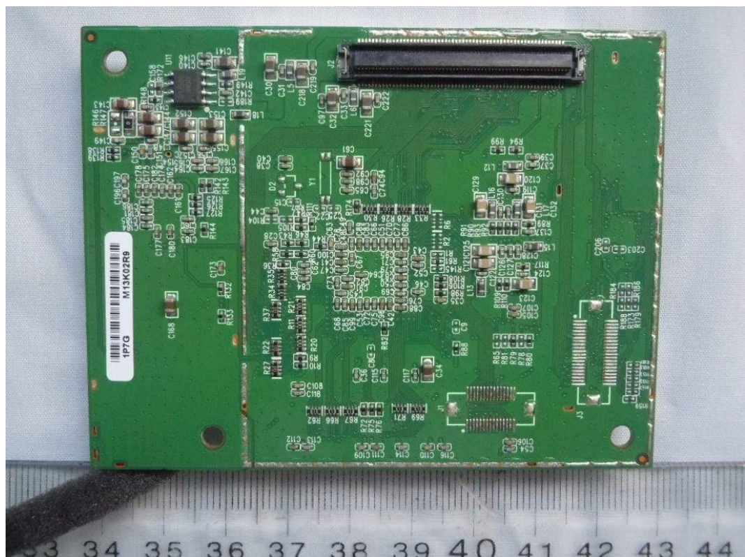
FIGURE 9 WIRELESS AIRPLAY SPEAKER (M/N: MA5000) RF BOARD (SOLDERED SIDE)
