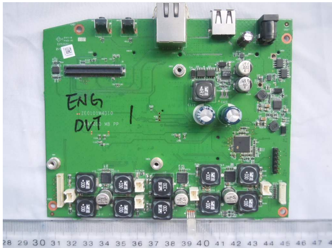
FIGURE 4 WIRELESS AIRPLAY SPEAKER (M/N: MA5000) MAIN BOARD (COMPONENT SIDE)
