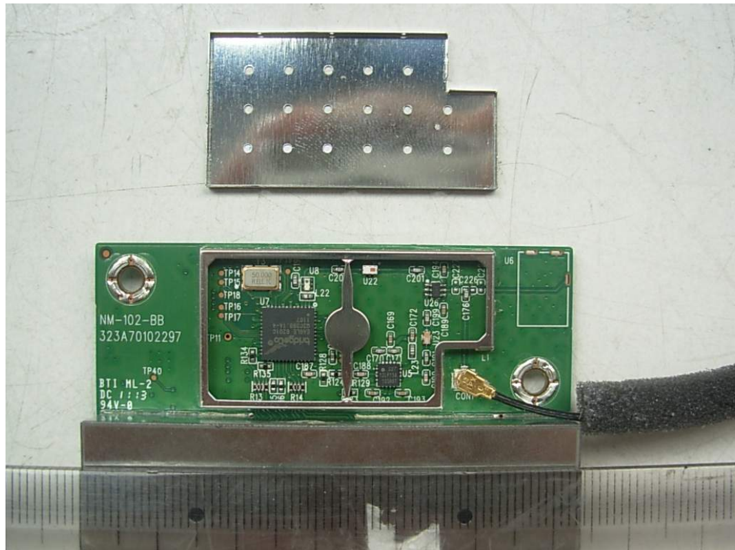
FIGURE 8 WIRELESS AIRPLAY SPEAKER (M/N: MA5000) RF BOARD (SHIELDED COVER REMOVED #2)
