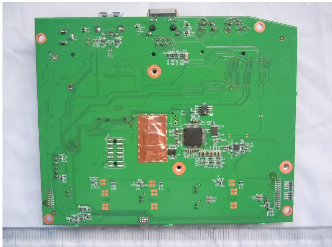
FIGURE 5 WIRELESS AIRPLAY SPEAKER (M/N: MA5000) MAIN BOARD (SOLDERED SIDE)
