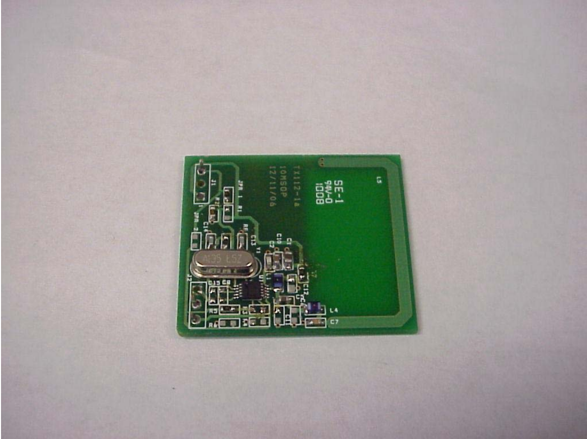
TX Transmitter Board – Top
