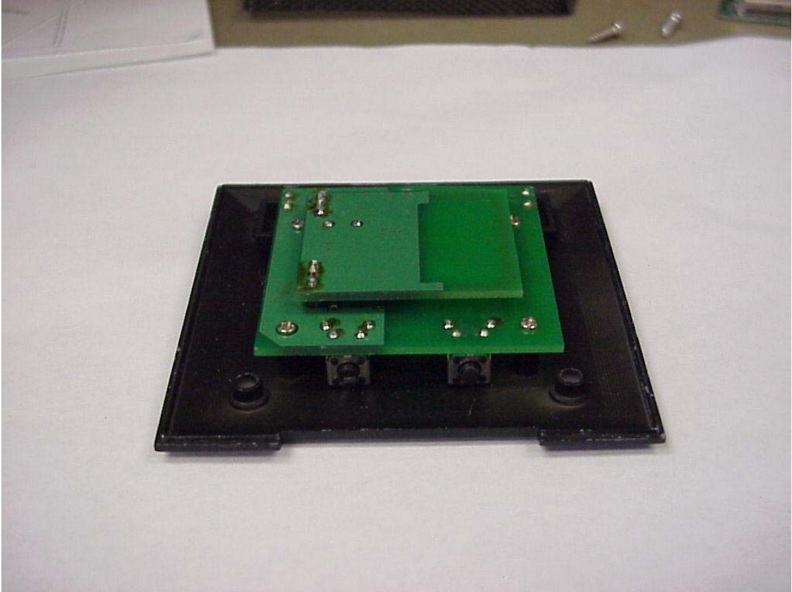
TX Assembly – Side View
