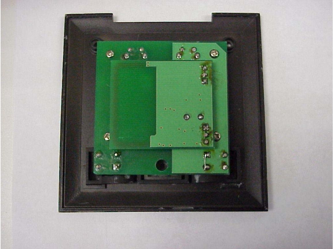
TX Assembly – Top View
