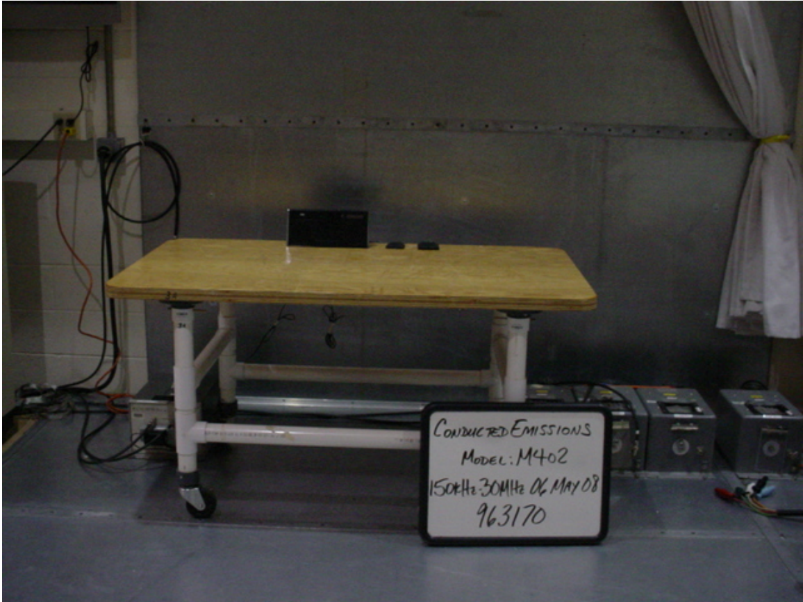
Conducted Emissions
