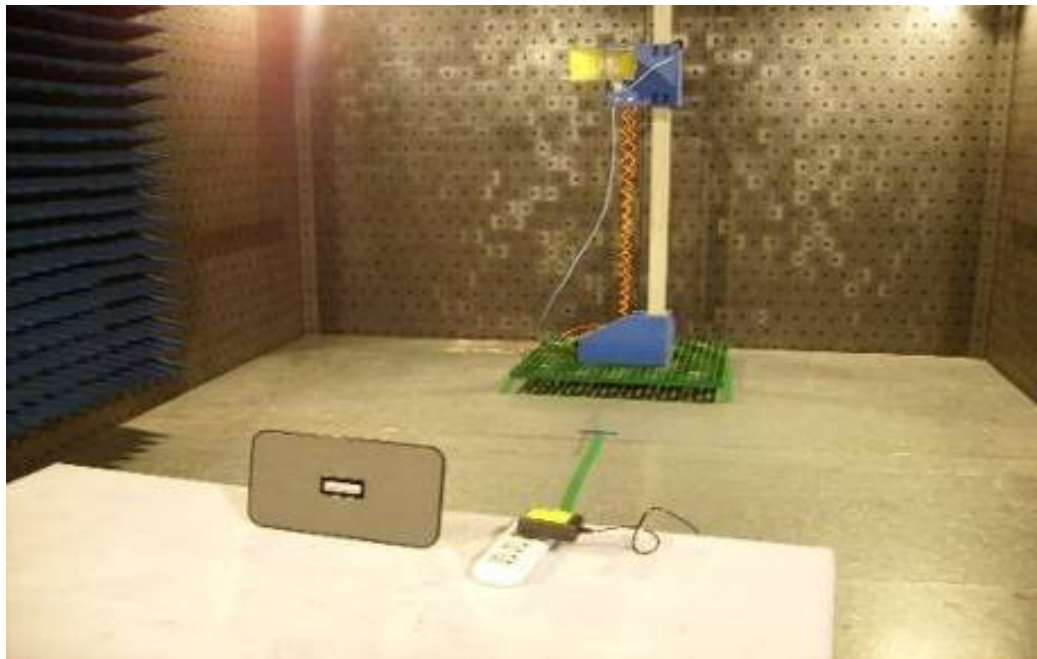
Spurious Emission
