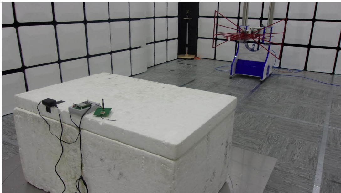
Photo 1.3-1 – Radiated Emissions 30-1000 MHz
