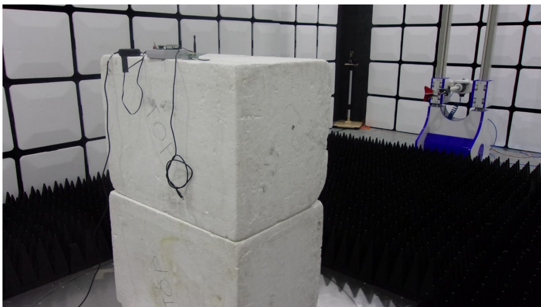
Photo 1.3-2 – Radiated Emissions Above 1 GHz
