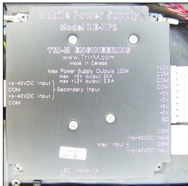
Power Supply
