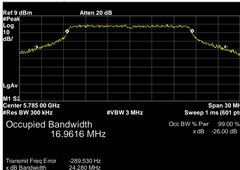
Figure 13: 26dB Bandwidth, 5785MHz, Chain 1
