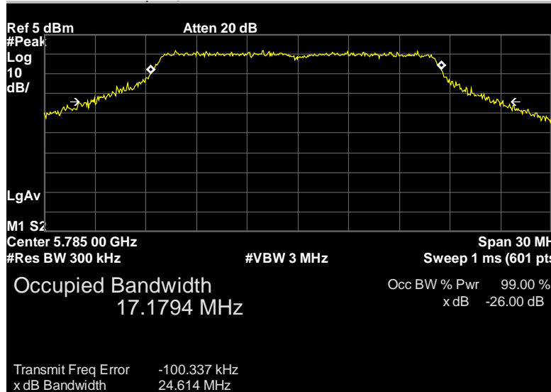
Figure 12: 26dB Bandwidth, 5785MHz, Chain 0
