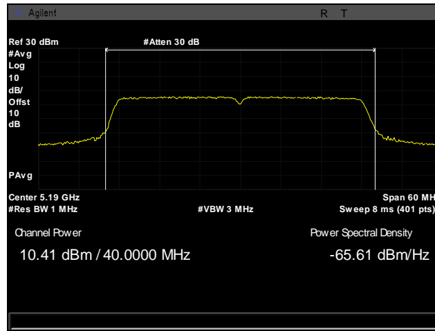
Plot 53. Conducted Transmitter Output Power, 802.11n 40 MHz, 5190 MHz, Channel 36, H, 16
