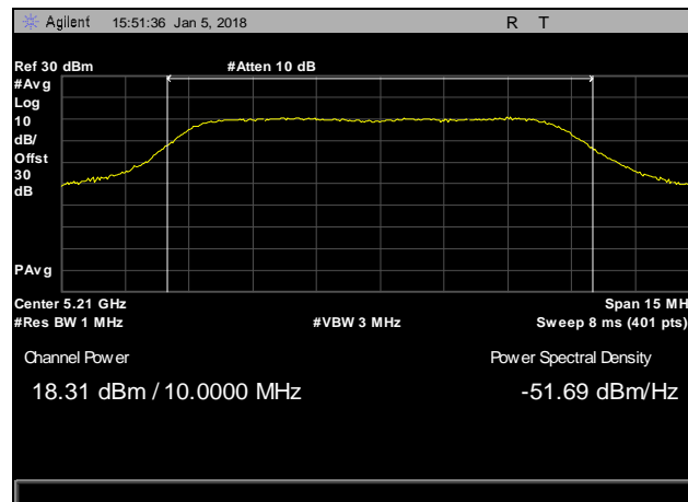
Plot 37. Conducted Transmitter Output Power, 10 MHz, 5210 MHz, Channel 42, H, 24
