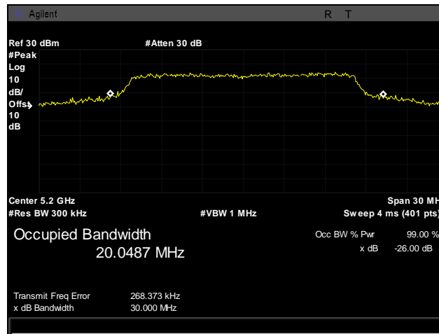
Plot 22. Occupied Bandwidth, 802.11n 20 MHz, 5200 MHz, Channel 40 I, 28
