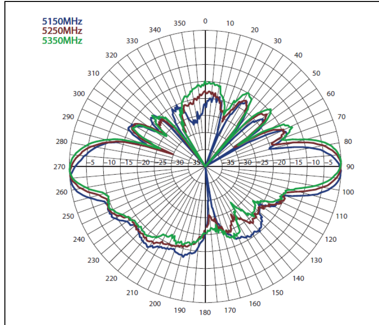
Plot 57. E-Plane, 0°
