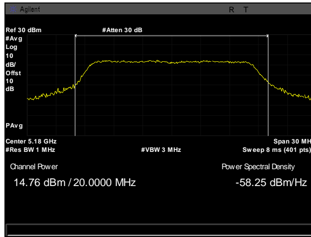
Plot 47. Conducted Transmitter Output Power, 802.11n 20 MHz, 5180 MHz, Channel 36, H, 21
