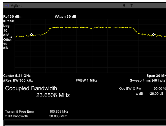
Plot 23. Occupied Bandwidth, 802.11n 20 MHz, 5240 MHz, Channel 48, H, 29
