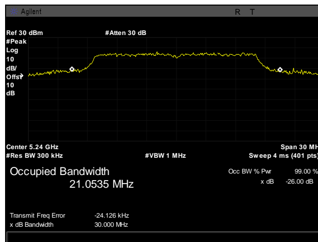
Plot 24. Occupied Bandwidth, 802.11n 20 MHz, 5240 MHz, Channel 48, I, 29
