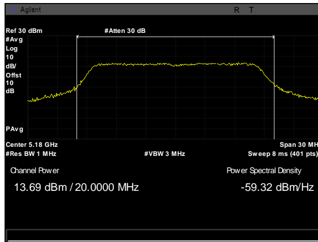
Plot 48. Conducted Transmitter Output Power, 802.11n 20 MHz, 5180 MHz, Channel 36, I, 21
