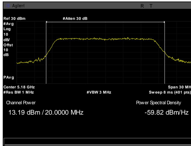
Plot 41. Conducted Transmitter Output Power, 20 MHz, 5180 MHz, Channel 36, H, 20
