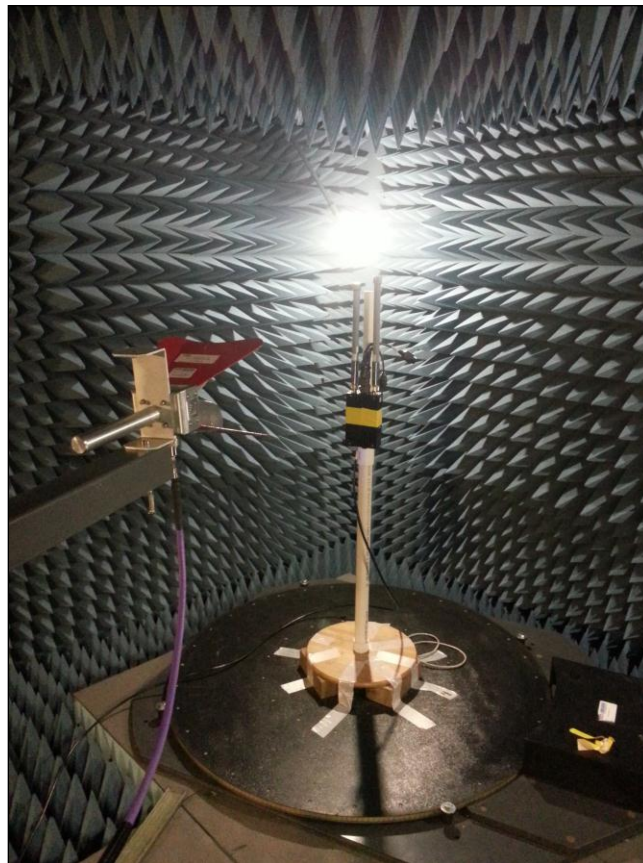
Photograph 7. Radiated Spurious Emissions, Test Setup, Above 1 GHz
