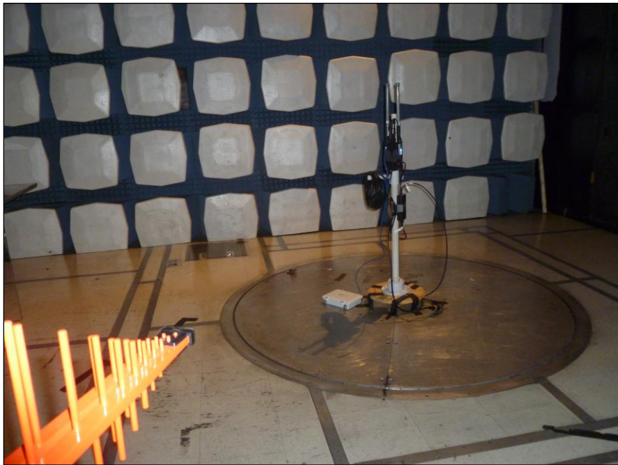
Photograph 3. Radiated Emissions, Test Setup, Blue and Black
