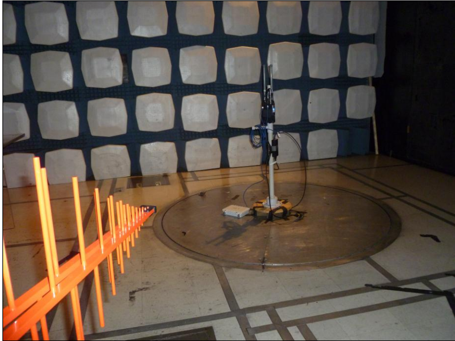
Photograph 2. Radiated Emissions, Test Setup, Blue Cable
