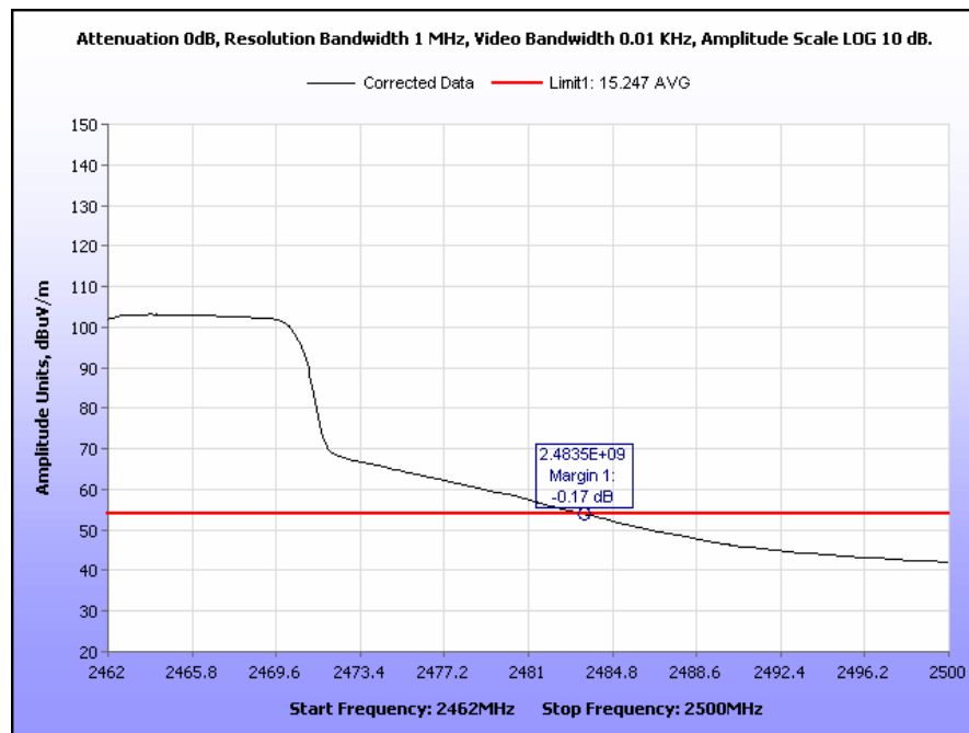
Plot 90. Radiated Restricted Band Edge, Channel 11, 2462 MHz – 2500 MHz, 802.11g Average
