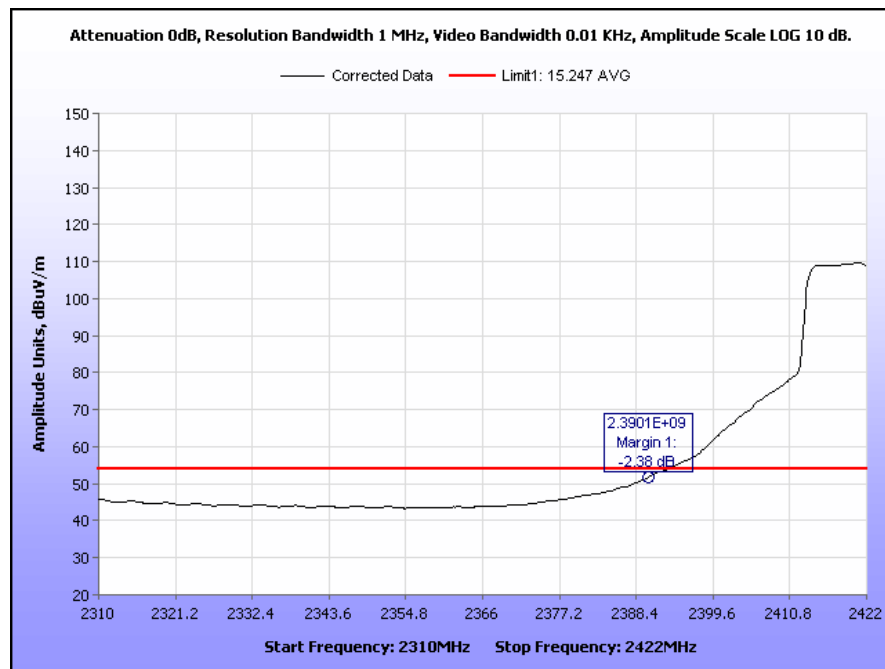
Plot 52. Radiated Restricted Band Edge, Channel 3, 2310 MHz – 2422 MHz, 802.11g, Average
