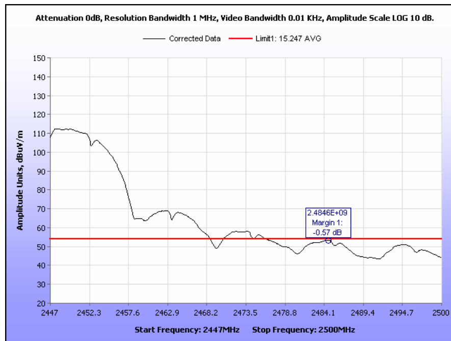
Plot 76. Radiated Restricted Band Edge, Channel 8, 2447 MHz – 2500 MHz, 802.11b, Average
