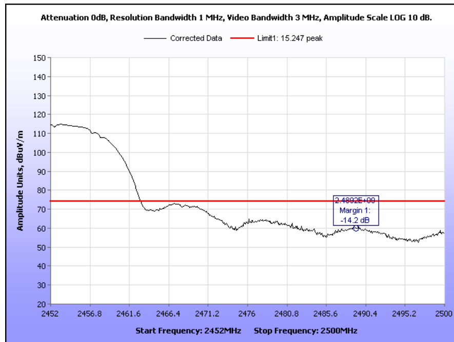
Plot 81. Radiated Restricted Band Edge, Channel 9, 2452 MHz – 2500 MHz, 802.11b, Peak
