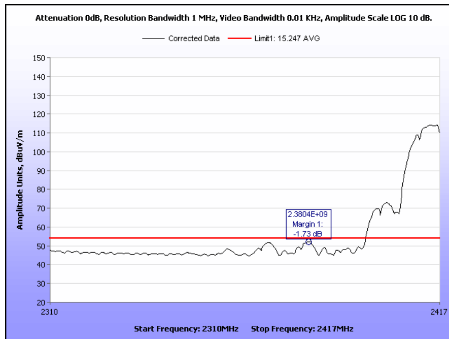
Plot 50. Radiated Restricted Band Edge, Channel 2, 2310 MHz – 2417 MHz, 802.11b, Average
