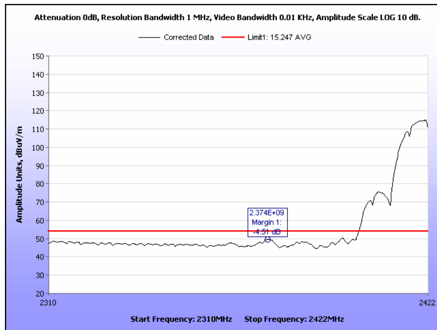
Plot 54. Radiated Restricted Band Edge, Channel 3, 2310 MHz – 2422 MHz, Average
