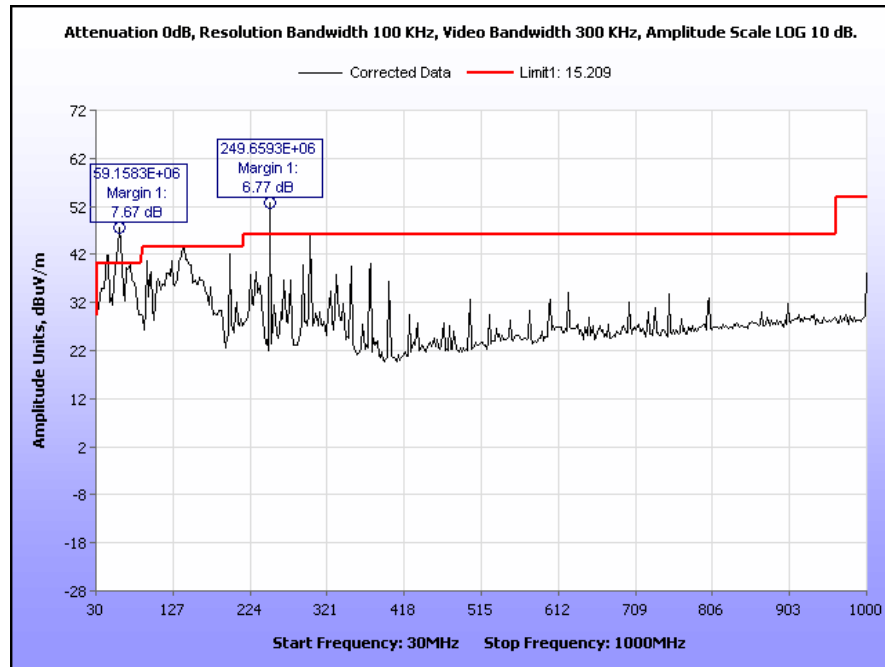
Plot 28. Radiated Spurious Emissions, Mid Channel, 802.11b, 13 dBm, 30 MHz – 1 GHz
