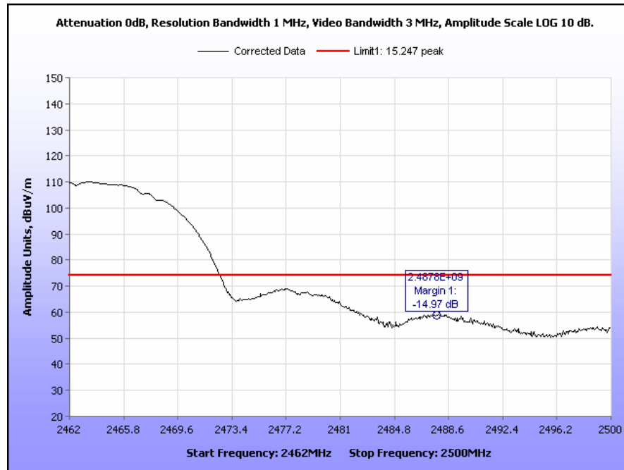
Plot 89. Radiated Restricted Band Edge, Channel 11, 2462 MHz – 2500 MHz, 802.11b Peak
