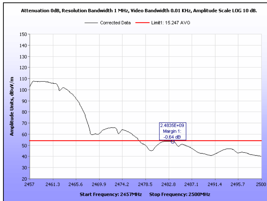
Plot 84. Radiated Restricted Band Edge, Channel 10, 2457 MHz – 2500 MHz, 802.11b Average
