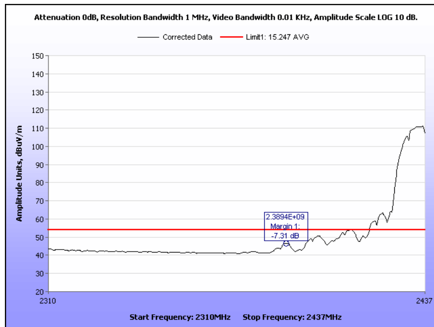
Plot 64. Radiated Restricted Band Edge, Channel 6, 2310 MHz – 2437 MHz, 802.11b, Average
