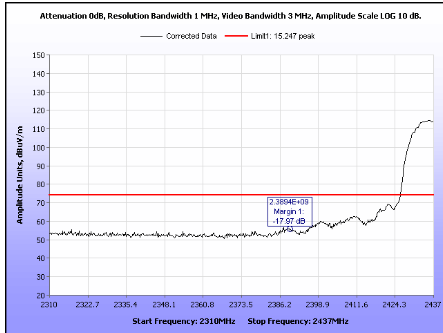
Plot 65. Radiated Restricted Band Edge, Channel 6, 2310 MHz – 2437 MHz, 802.11b, Peak
