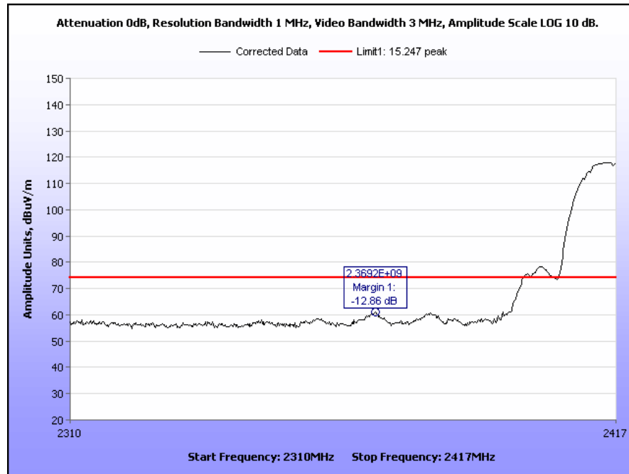
Plot 51. Radiated Restricted Band Edge, Channel 2, 2310 MHz – 2417 MHz, 802.11b, Peak
