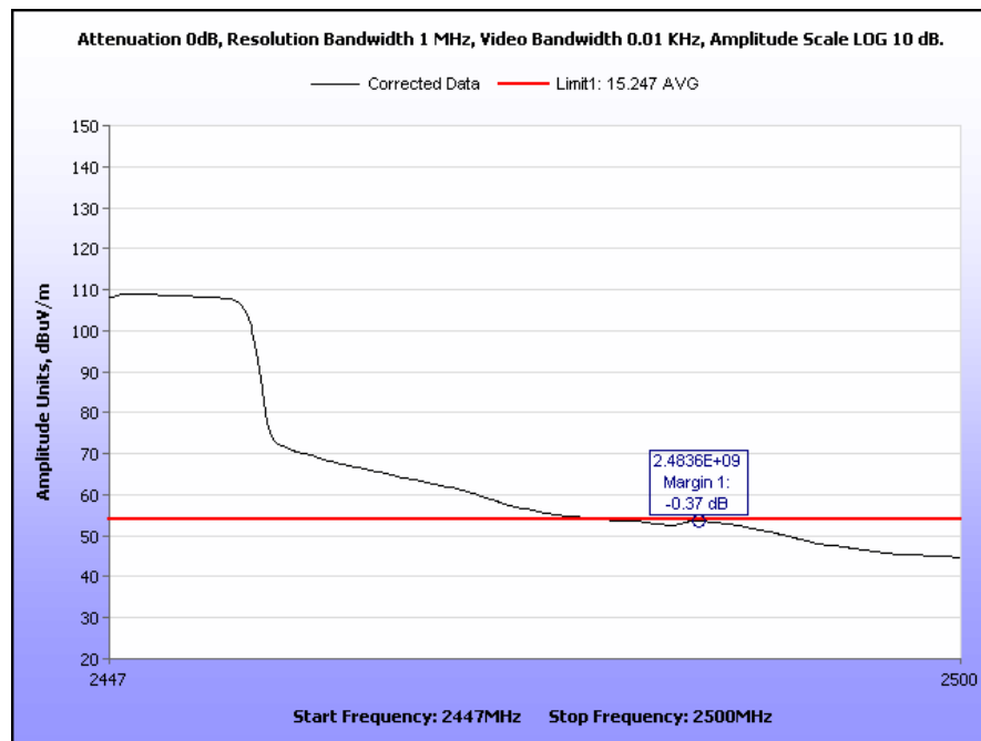
Plot 78. Radiated Restricted Band Edge, Channel 8, 2447 MHz – 2500 MHz, 802.11g, Average
