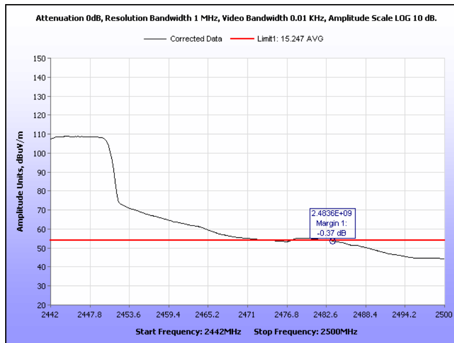
Plot 74. Radiated Restricted Band Edge, Channel 7, 2442 MHz – 2500 MHz, 802.11g, Average
