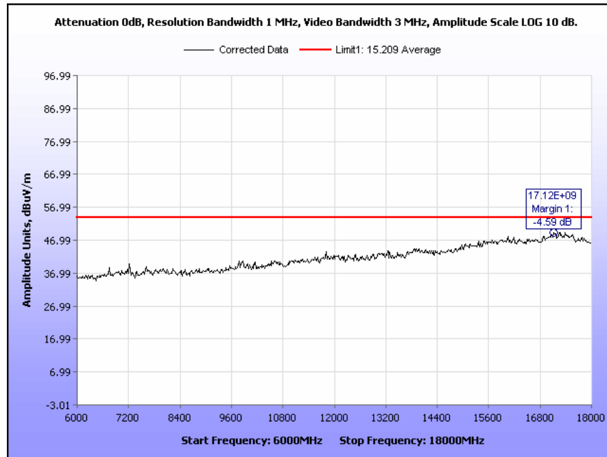
Plot 26. Radiated Spurious Emissions, Low Channel, 802.11g, 11 dBm, 6 GHz – 18 GHz
