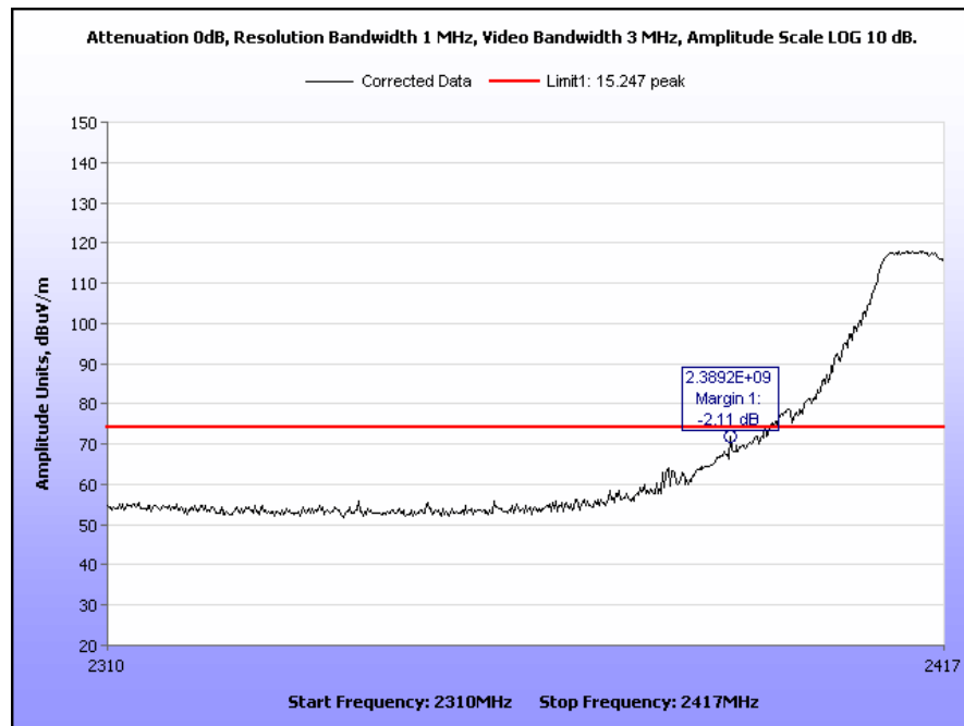
Plot 49. Radiated Restricted Band Edge, Channel 2, 2310 MHz – 2417 MHz, 802.11g, Peak
