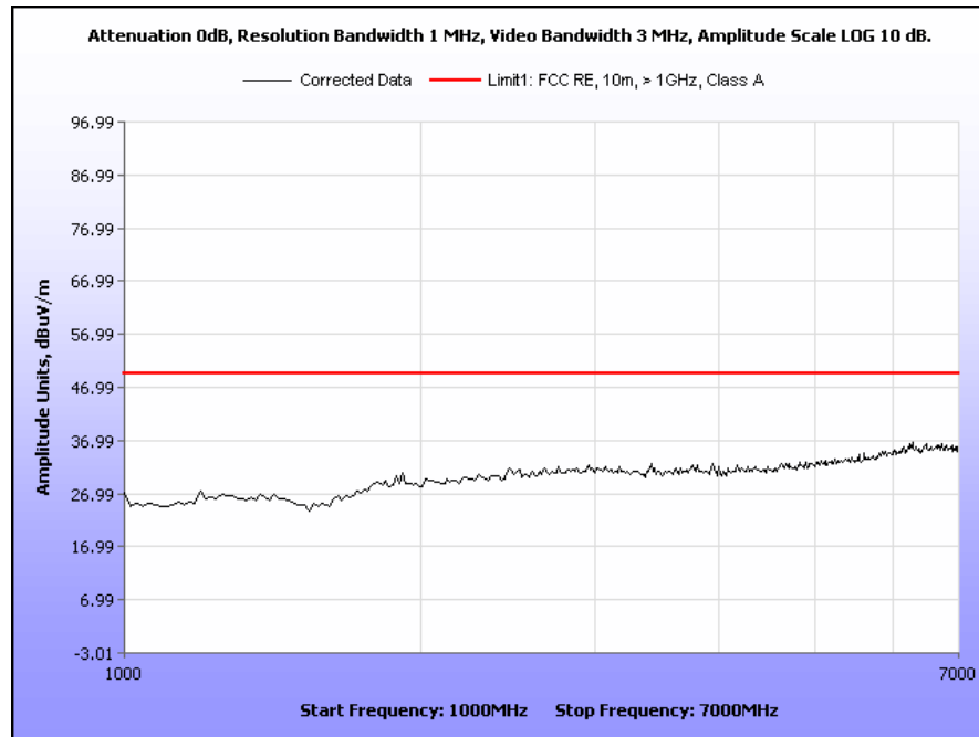
Plot 4. Radiated Emissions, Pre-Scan, 1 GHz – 7 GHz, FCC Limits
