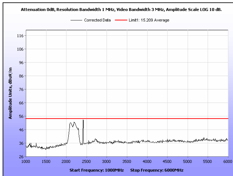
Plot 18. Radiated Spurious Emissions, Low Channel, 802.11b, 15 dBm, 1 GHz – 6 GHz
