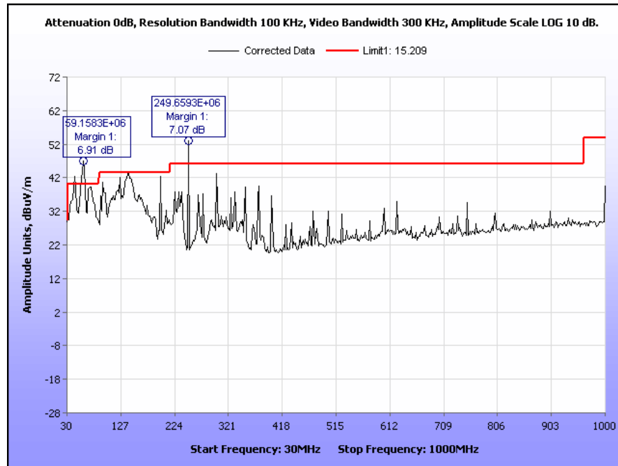
Plot 24. Radiated Spurious Emissions, Low Channel, 802.11g, 11 dBm, 30 MHz – 1 GHz
