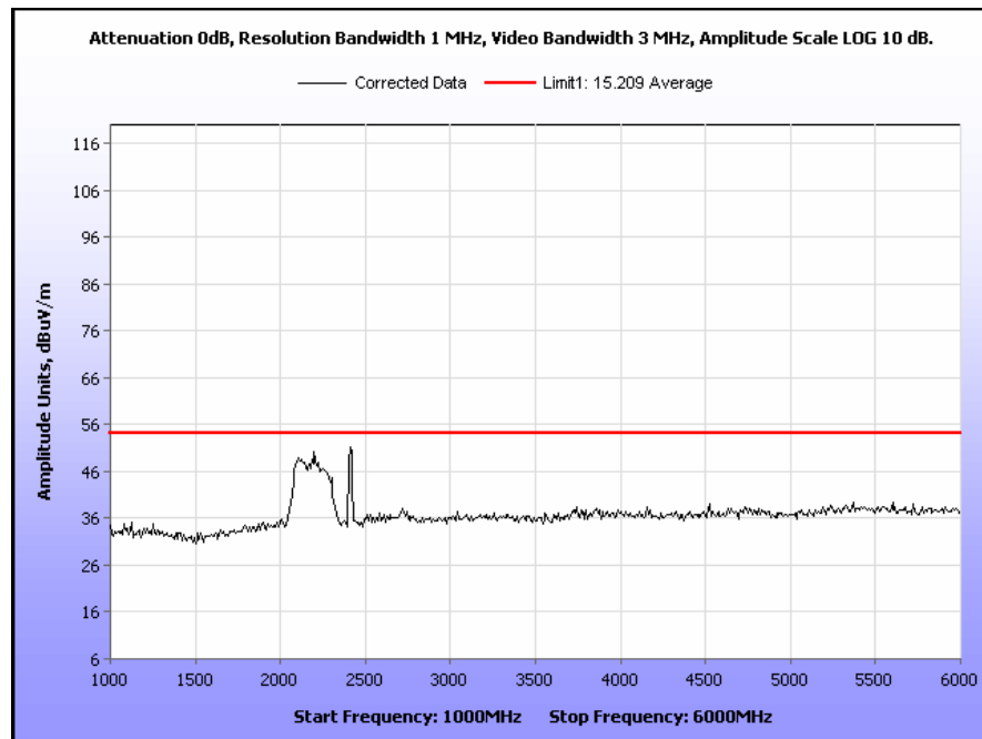
Plot 25. Radiated Spurious Emissions, Low Channel, 802.11g, 11 dBm, 1 GHz – 6 GHz
