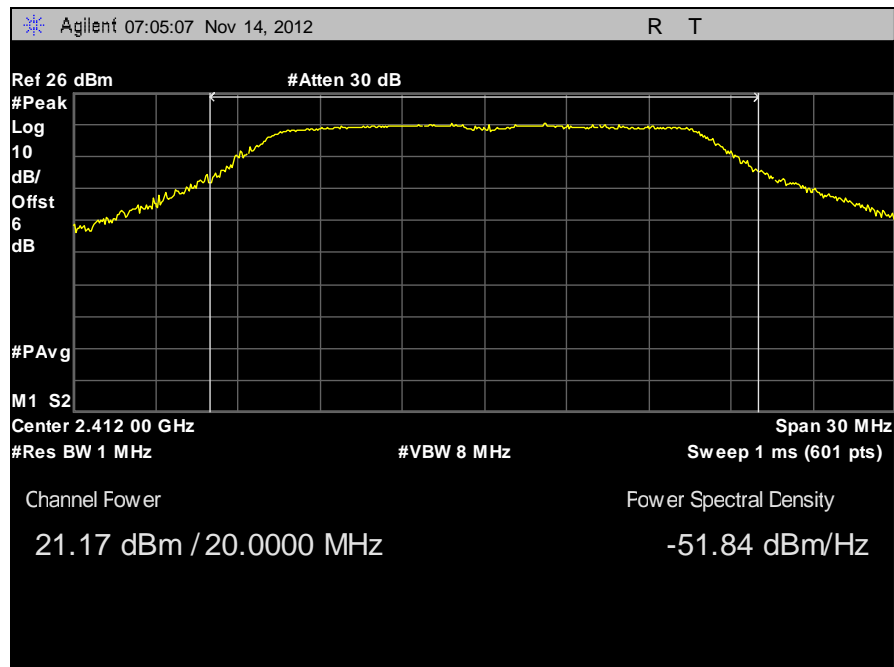
Plot 8. Peak Power Output, Channel 1, 802.11g
