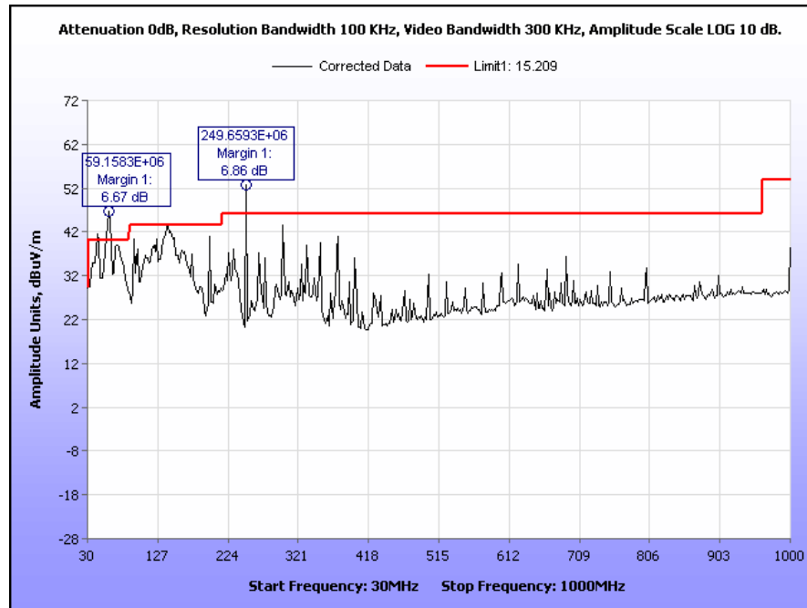
Plot 32. Radiated Spurious Emissions, Mid Channel, 802.11g, 15 dBm, 30 MHz – 1 GHz
