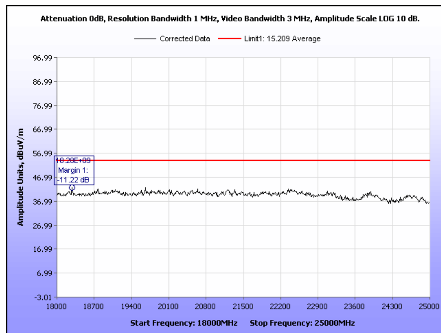
Plot 23. Radiated Spurious Emissions, Low Channel, 802.11b, 15 dBm, 18 GHz – 25 GHz
