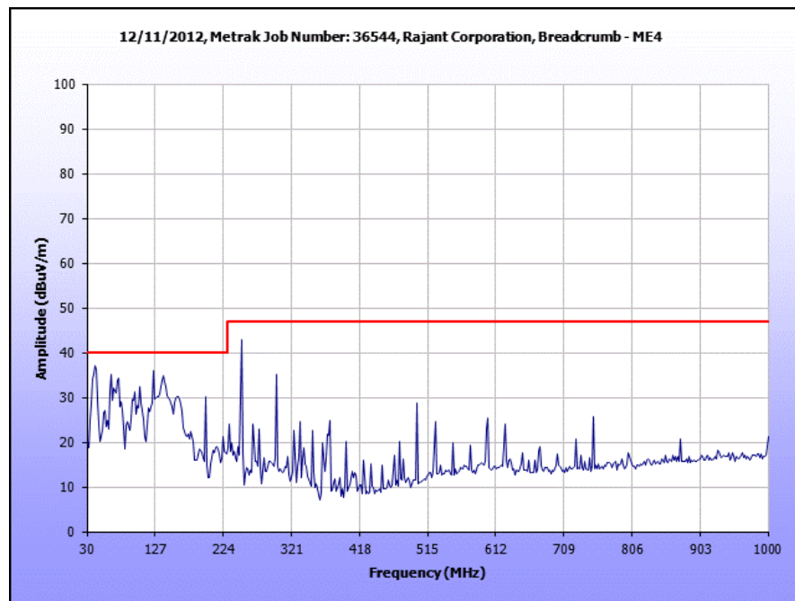
Plot 5. Radiated Emissions, Pre-Scan, ICES-003 Limits
