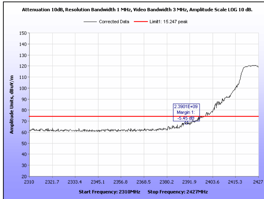
Plot 59. Radiated Restricted Band Edge, Channel 4, 2310 MHz – 2427 MHz, 802.11g, Peak
