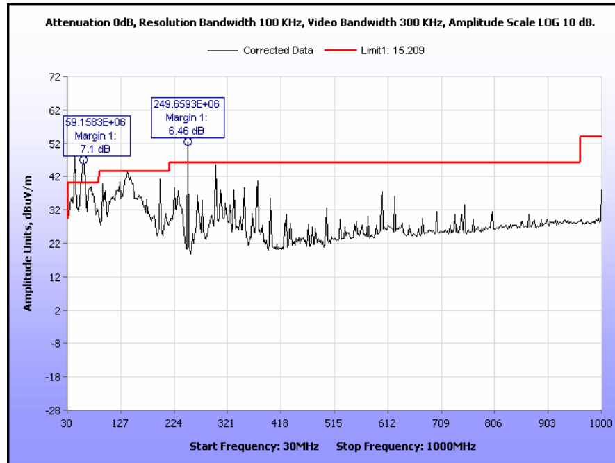
Plot 36. Radiated Spurious Emissions, High Channel, 802.11b, 9 dBm, 30 MHz – 1 GHz
