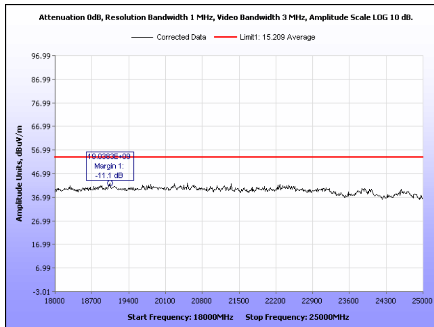
Plot 39. Radiated Spurious Emissions, High Channel, 802.11b, 9 dBm, 18 GHz – 25 GHz
