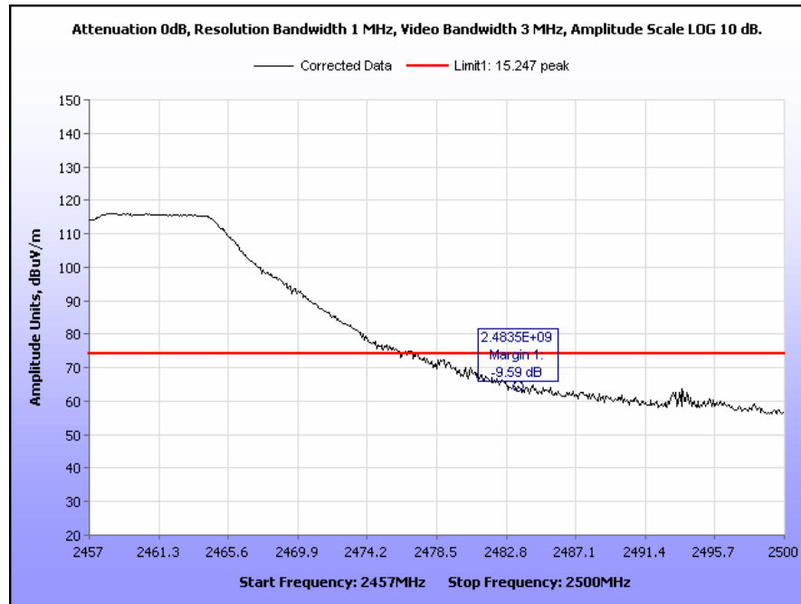
Plot 87. Radiated Restricted Band Edge, Channel 10, 2457 MHz – 2500 MHz, 802.11g Peak
