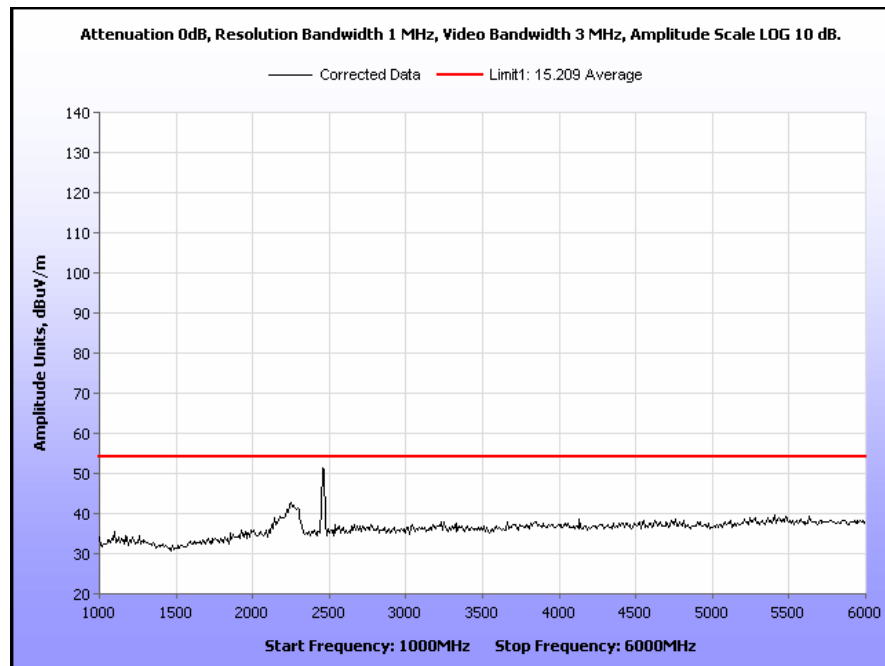
Plot 37. Radiated Spurious Emissions, High Channel, 802.11b, 9 dBm, 1 GHz – 6 GHz
