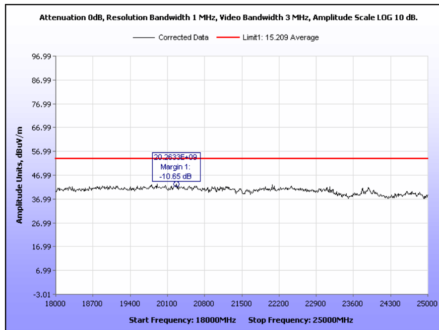
Plot 43. Radiated Spurious Emissions, High Channel, 802.11g, 9 dBm, 18 GHz – 25 GHz
