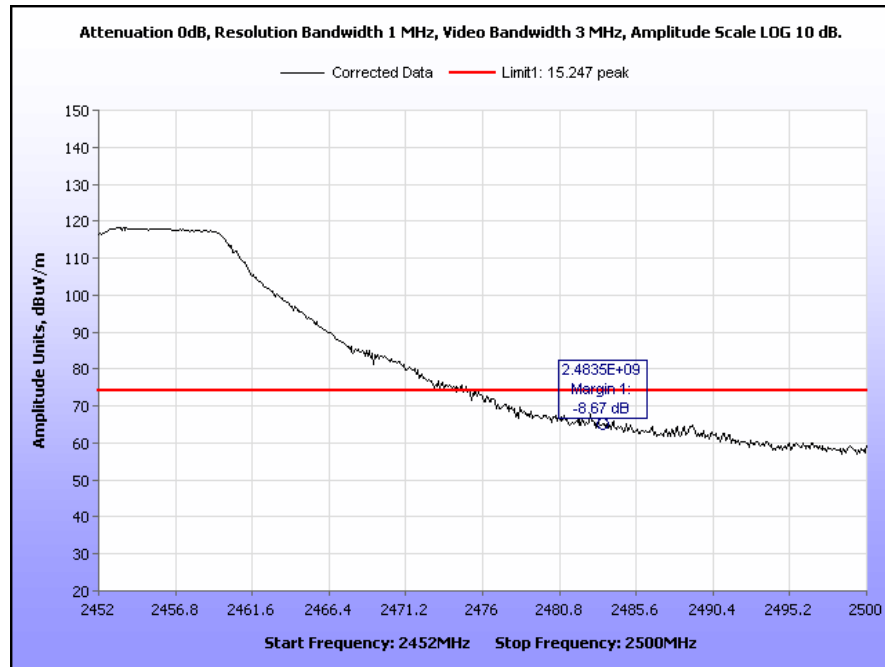
Plot 83. Radiated Restricted Band Edge, Channel 9, 2452 MHz – 2500 MHz, 802.11g, Peak
