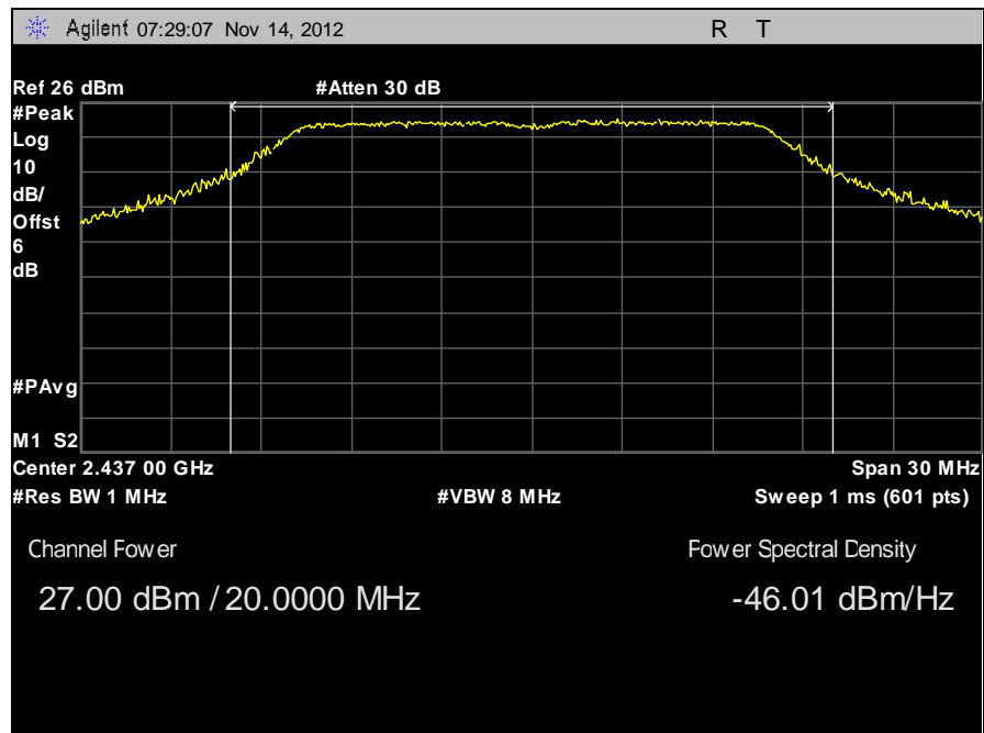
Plot 12. Peak Power Output, Channel 6, 802.11g
