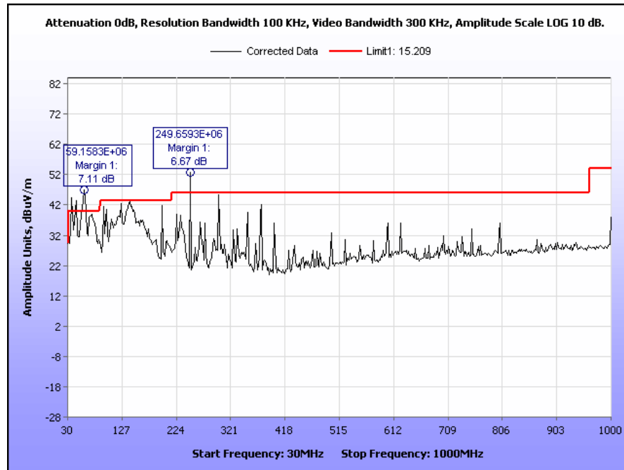
Plot 17. Radiated Spurious Emissions, Low Channel, 802.11b, 15 dBm, 30 MHz – 1 GHz
