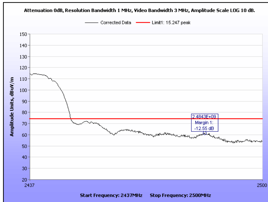
Plot 69. Radiated Restricted Band Edge, Channel 6, 2437 MHz – 2500 MHz, 802.11b, Peak
