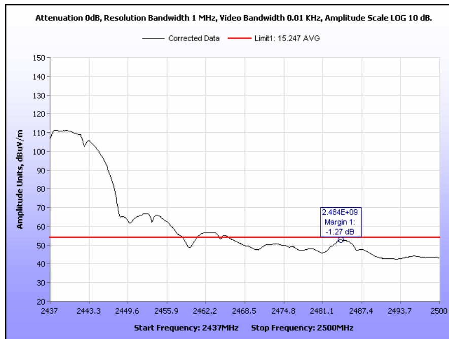
Plot 68. Radiated Restricted Band Edge, Channel 6, 2437 MHz – 2500 MHz, 802.11b, Average
