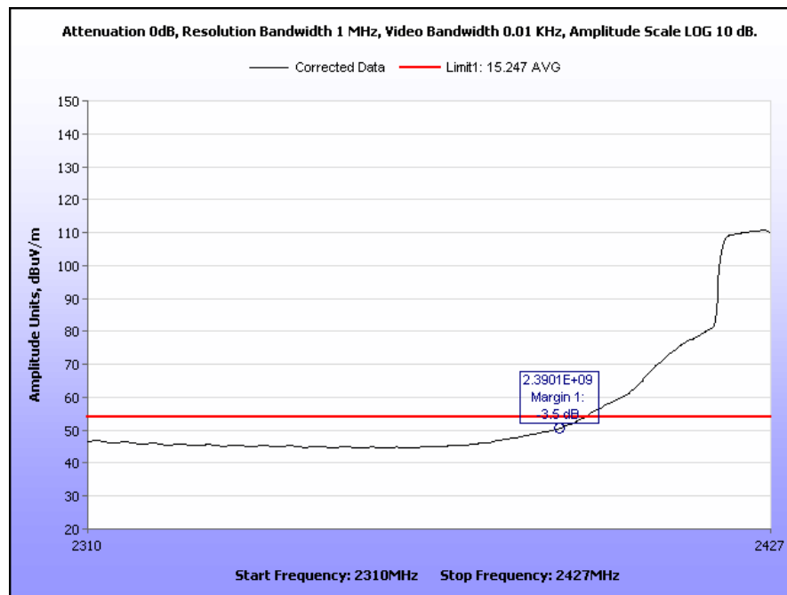
Plot 58. Radiated Restricted Band Edge, Channel 4, 2310 MHz – 2427 MHz, 802.11g, Average
