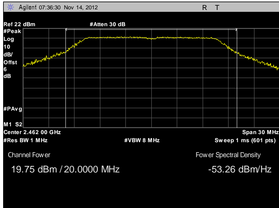
Plot 14. Peak Power Output, Channel 11, 802.11g
