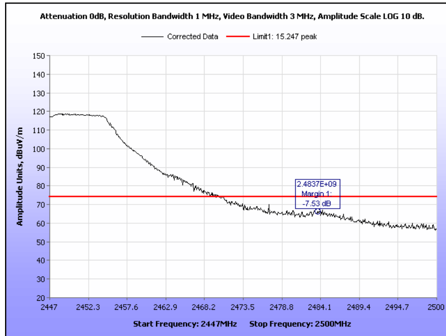
Plot 79. Radiated Restricted Band Edge, Channel 8, 2447 MHz – 2500 MHz, 802.11g, Peak
