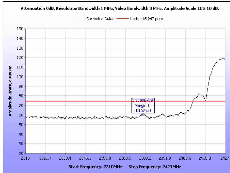
Plot 57. Radiated Restricted Band Edge, Channel 4, 2310 MHz – 2427 MHz, 802.11b, Peak
