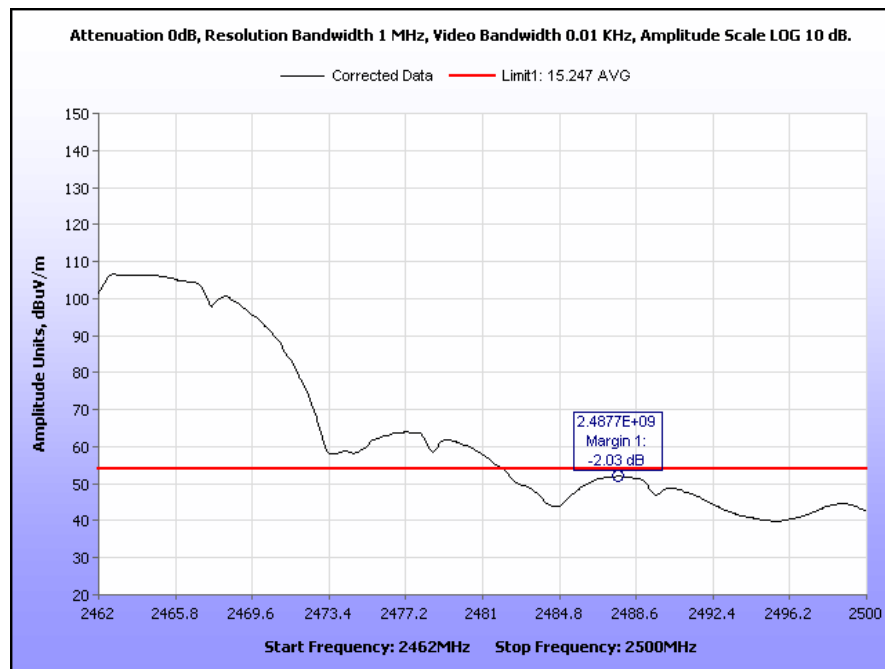
Plot 88. Radiated Restricted Band Edge, Channel 11, 2462 MHz – 2500 MHz, 802.11b Average
