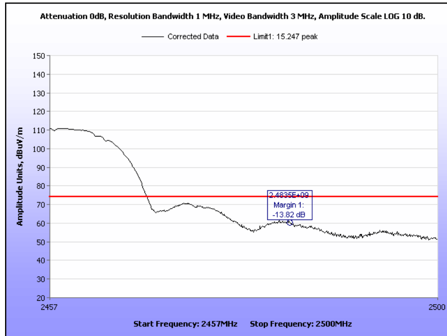
Plot 85. Radiated Restricted Band Edge, Channel 10, 2457 MHz – 2500 MHz, 802.11b Peak
