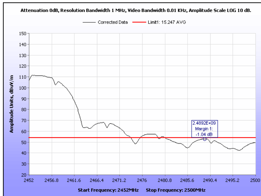
Plot 80. Radiated Restricted Band Edge, Channel 9, 2452 MHz – 2500 MHz, 802.11b, Average
