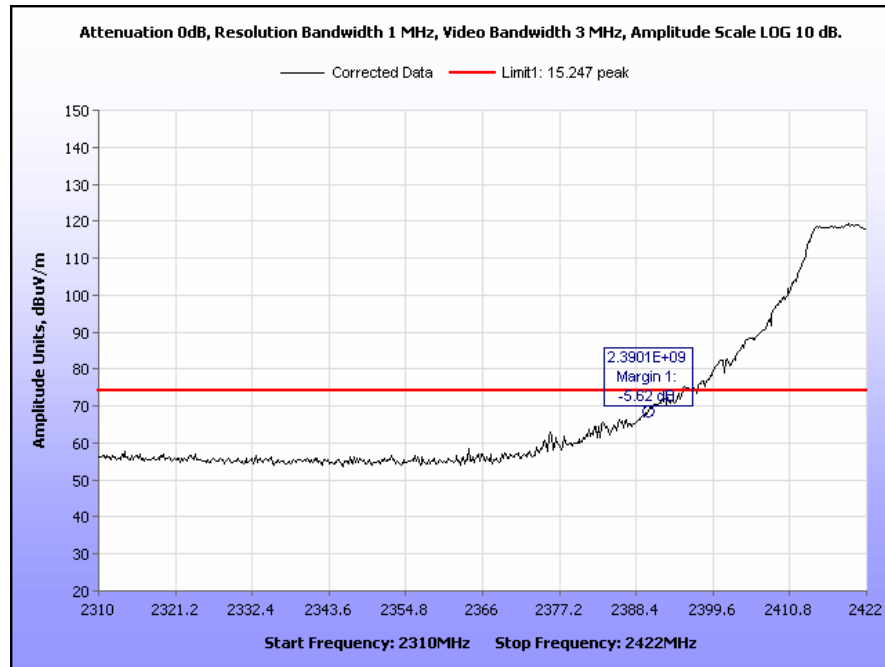
Plot 53. Radiated Restricted Band Edge, Channel 3, 2310 MHz – 2422 MHz, 802.11g, Peak
