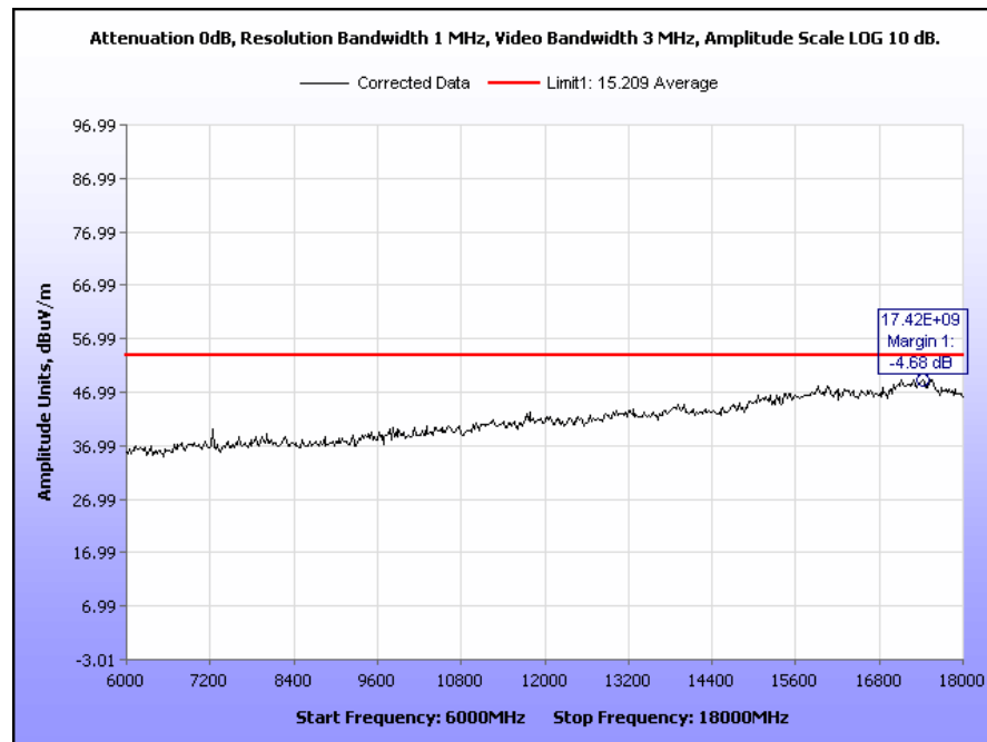
Plot 22. Radiated Spurious Emissions, Low Channel, 802.11b, 15 dBm, 6 GHz – 18 GHz
