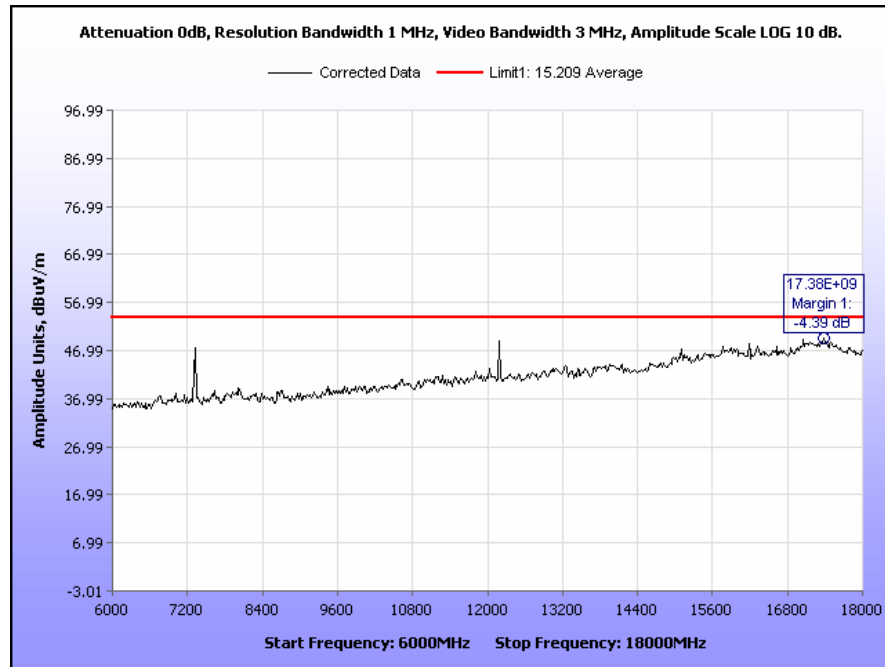
Plot 34. Radiated Spurious Emissions, Mid Channel, 802.11g, 15 dBm, 6 GHz – 18 GHz
