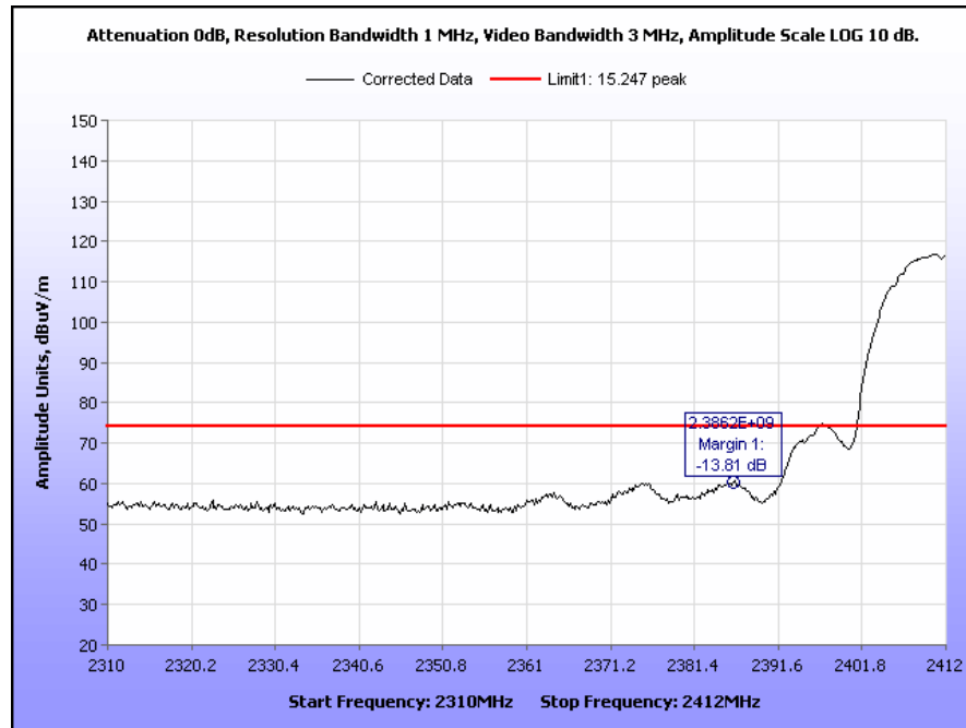
Plot 47. Radiated Restricted Band Edge, Channel 1, 2310 MHz – 2412 MHz, 802.11b, Peak
