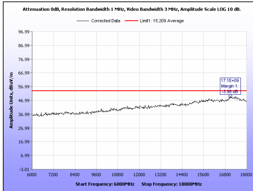
Plot 38. Radiated Spurious Emissions, High Channel, 802.11b, 9 dBm, 6 GHz – 18 GHz
