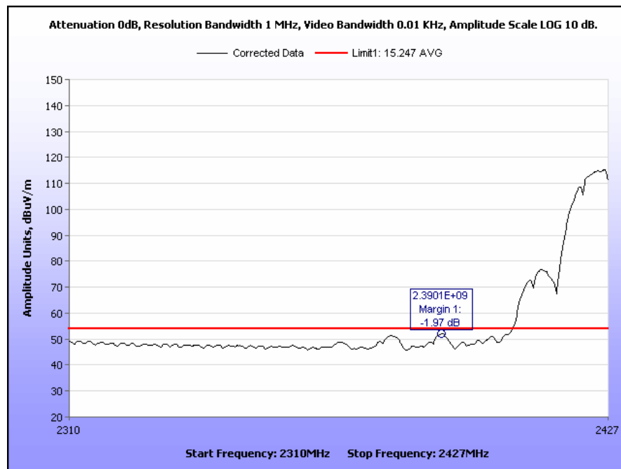
Plot 56. Radiated Restricted Band Edge, Channel 4, 2310 MHz – 2427 MHz, 802.11b, Average
