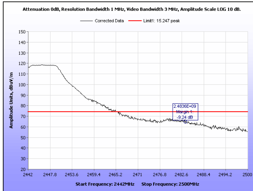
Plot 75. Radiated Restricted Band Edge, Channel 7, 2442 MHz – 2500 MHz, 802.11g, Peak
