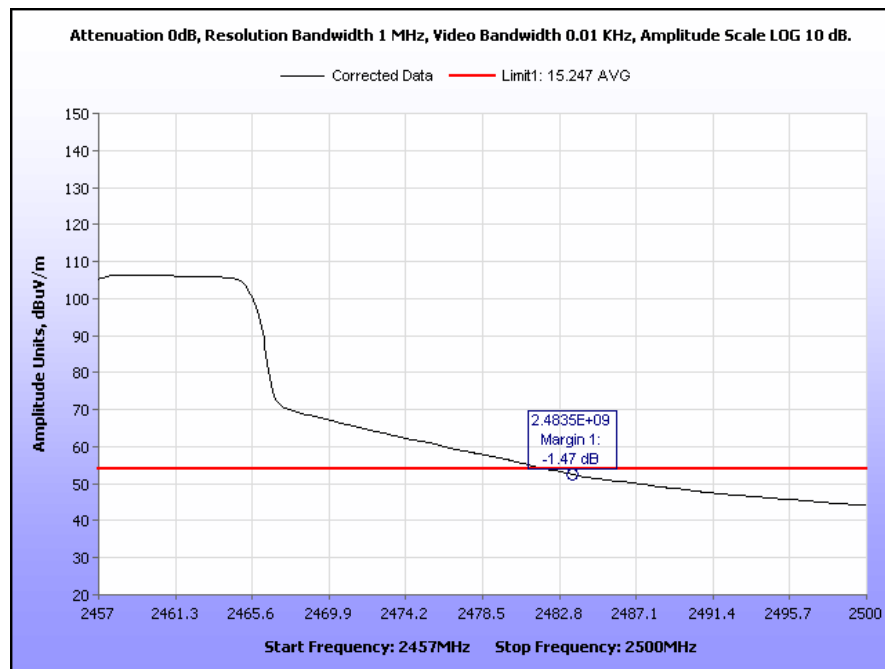
Plot 86. Radiated Restricted Band Edge, Channel 10, 2457 MHz – 2500 MHz, 802.11g Average
