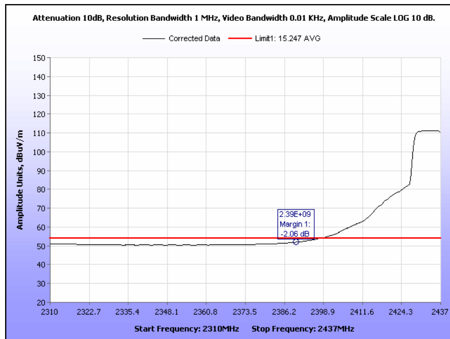
Plot 66. Radiated Restricted Band Edge, Channel 6, 2310 MHz – 2437 MHz, 802.11g, Average
