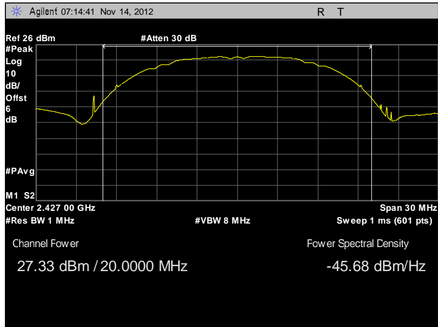
Plot 9. Peak Power Output, Channel 4, 802.11b
