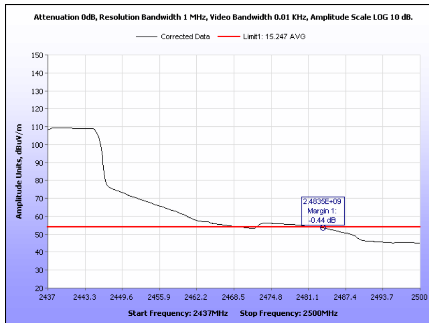
Plot 70. Radiated Restricted Band Edge, Channel 6, 2437 MHz – 2500 MHz, 802.11g, Average
