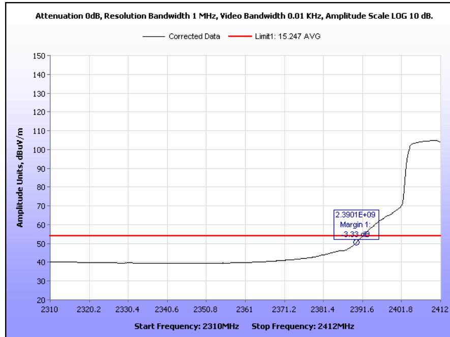
Plot 44. Radiated Restricted Band Edge, Channel 1, 2310 MHz – 2412 MHz, 802.11g, Average
