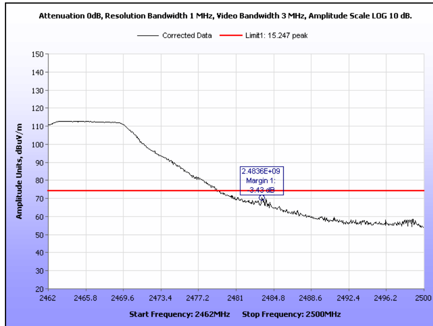
Plot 91. Radiated Restricted Band Edge, Channel 11, 2462 MHz – 2500 MHz, 802.11g Peak
