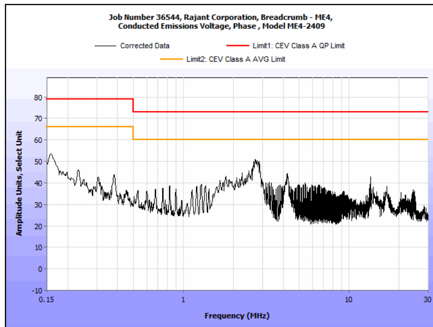
Plot 8. Conducted Emissions, 15.207(a), Phase Line
