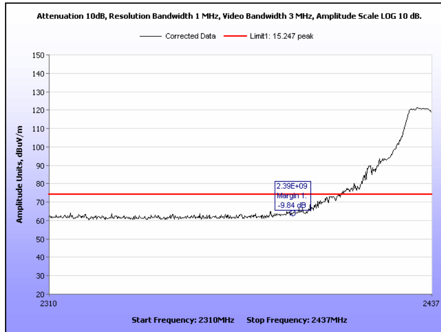
Plot 67. Radiated Restricted Band Edge, Channel 6, 2310 MHz – 2437 MHz, 802.11g, Peak
