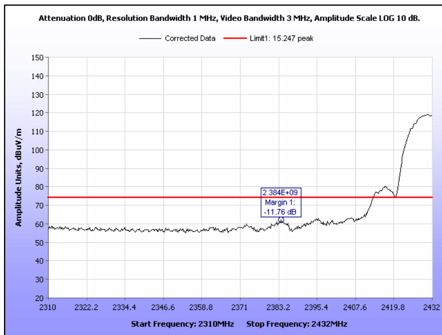
Plot 61. Radiated Restricted Band Edge, Channel 5, 2310 MHz – 2432 MHz, 802.11b, Peak
