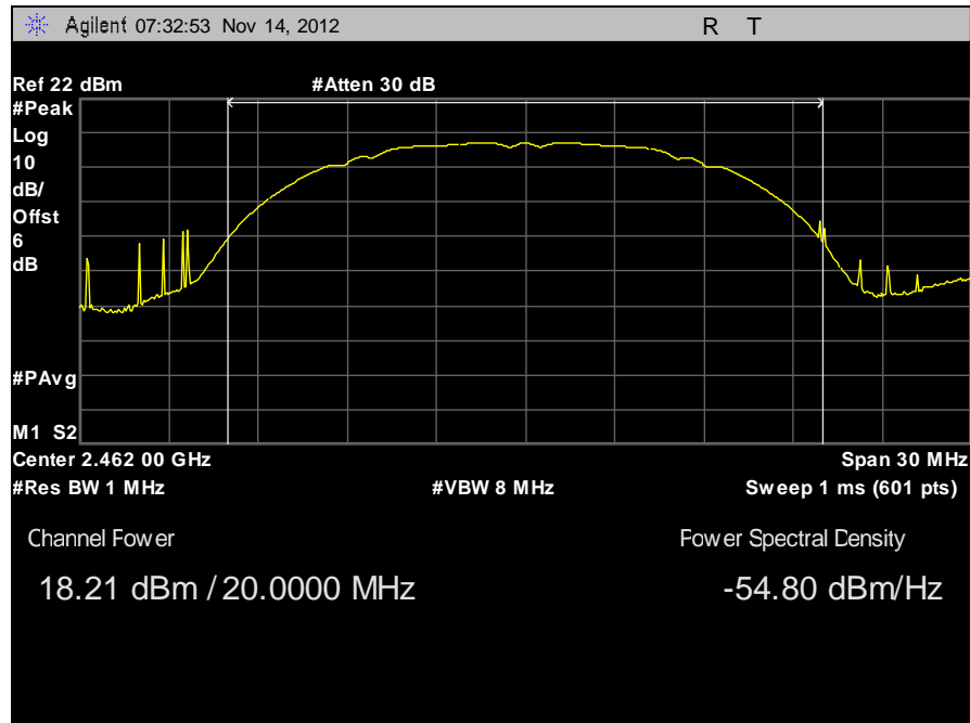
Plot 13. Peak Power Output, Channel 11, 802.11b
