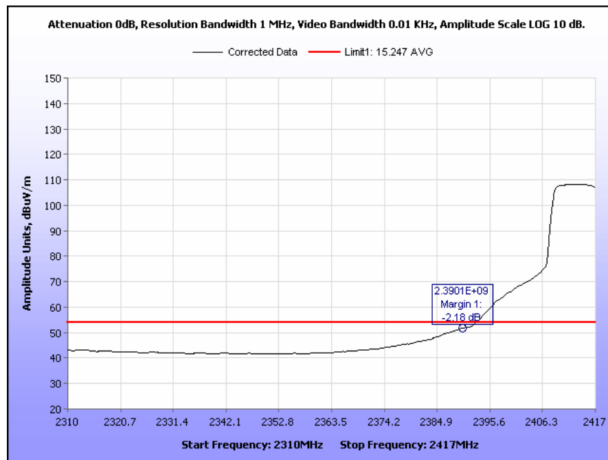
Plot 48. Radiated Restricted Band Edge, Channel 2, 2310 MHz – 2417 MHz, 802.11g, Average
