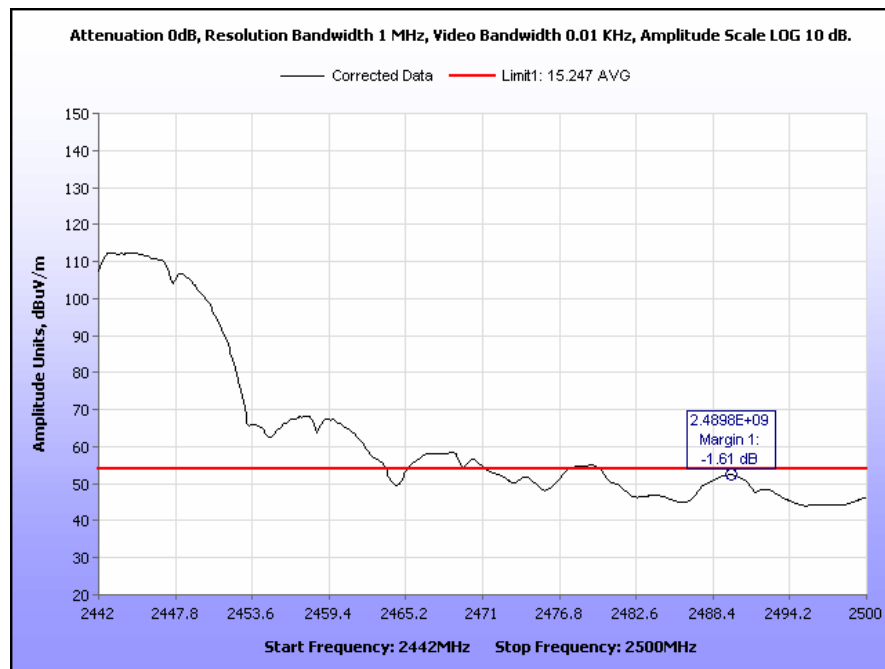
Plot 72. Radiated Restricted Band Edge, Channel 7, 2442 MHz – 2500 MHz, 802.11b, Average
