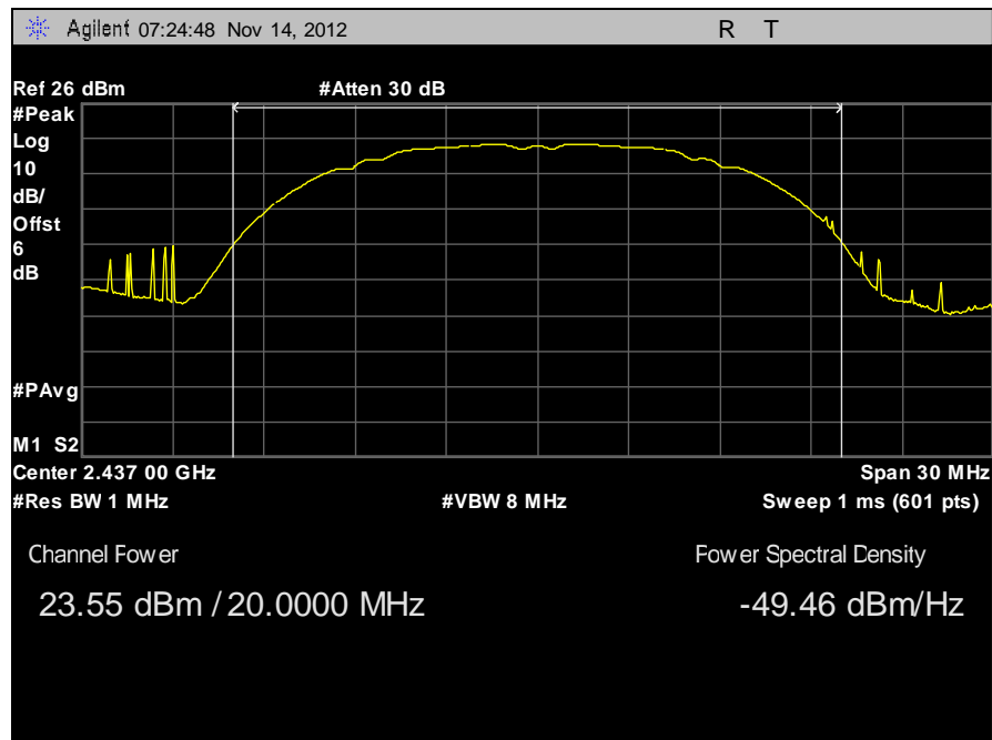
Plot 11. Peak Power Output, Channel 6, 802.11b
