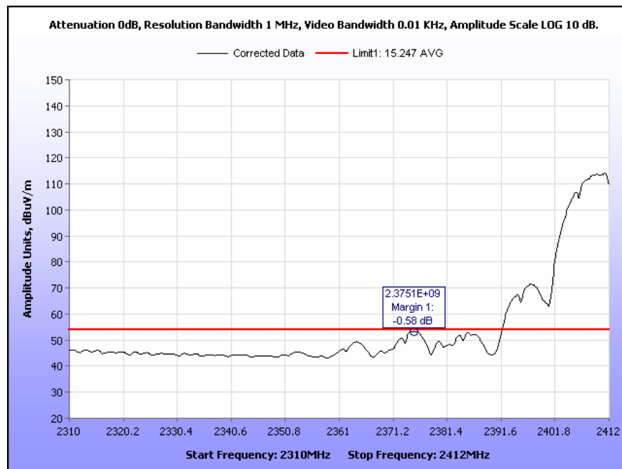
Plot 46. Radiated Restricted Band Edge, Channel 1, 2310 MHz – 2412 MHz, 802.11b, Average
