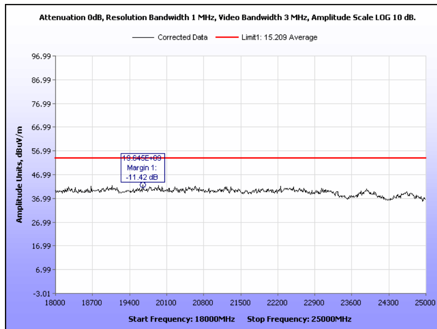
Plot 31. Radiated Spurious Emissions, Mid Channel, 802.11b, 13 dBm, 18 GHz – 25 GHz
