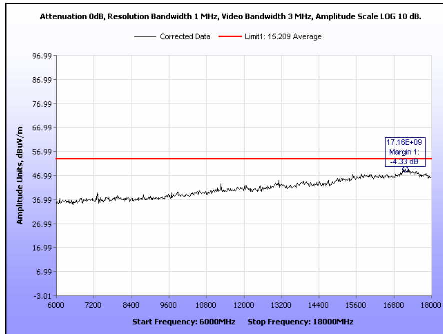
Plot 30. Radiated Spurious Emissions, Mid Channel, 802.11b, 13 dBm, 6 GHz – 18 GHz
