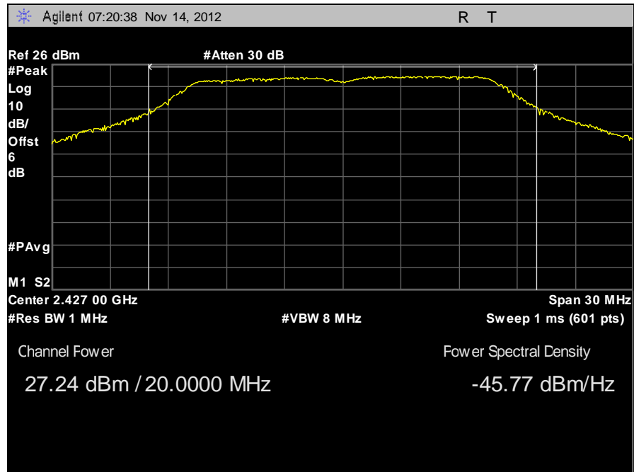
Plot 10. Peak Power Output, Channel 4, 802.11g
