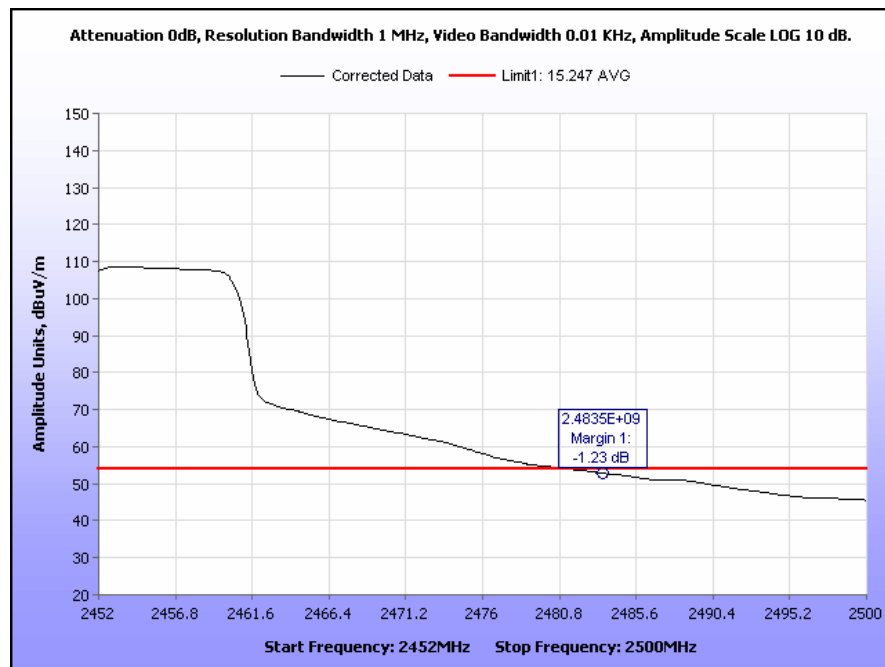
Plot 82. Radiated Restricted Band Edge, Channel 9, 2452 MHz – 2500 MHz, 802.11g, Average
