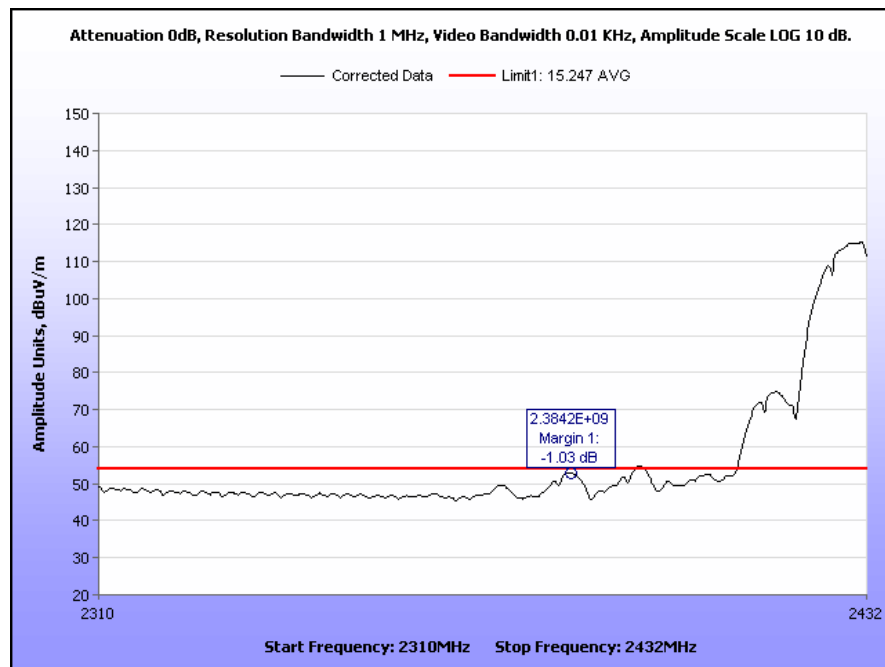
Plot 60. Radiated Restricted Band Edge, Channel 5, 2310 MHz – 2432 MHz, 802.11b, Average
