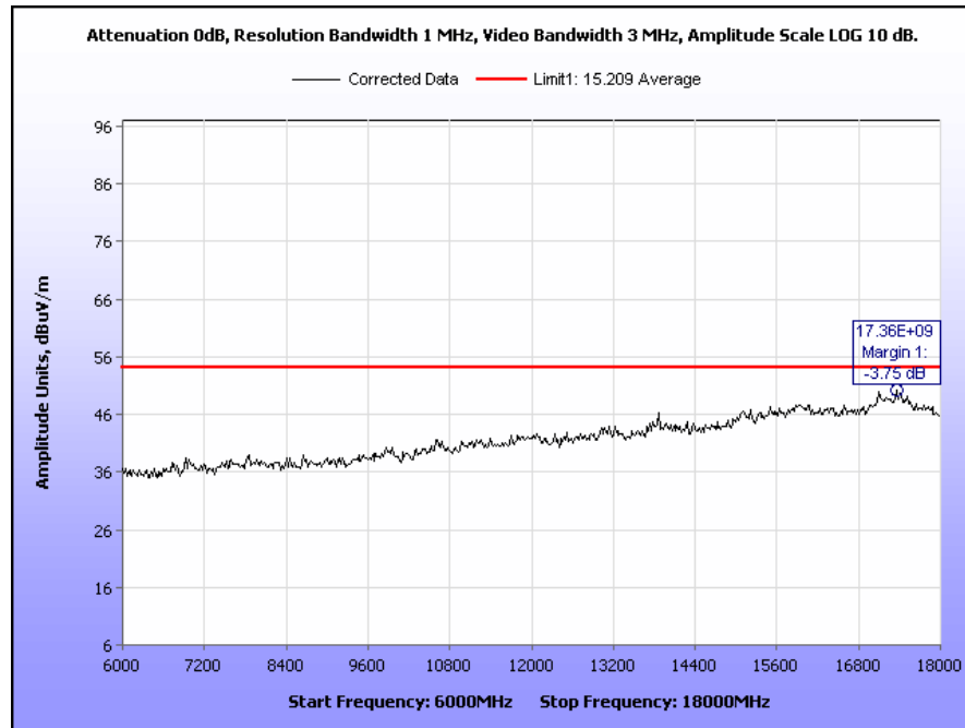
Plot 42. Radiated Spurious Emissions, High Channel, 802.11g, 9 dBm, 6 GHz – 18 GHz
