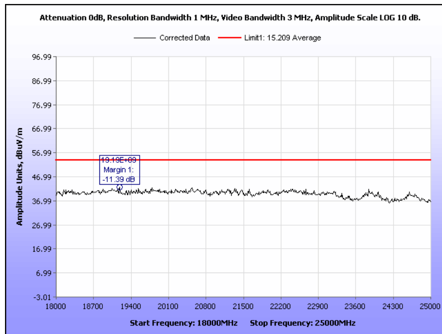
Plot 35. Radiated Spurious Emissions, Mid Channel, 802.11g, 15 dBm, 18 GHz – 25 GHz
