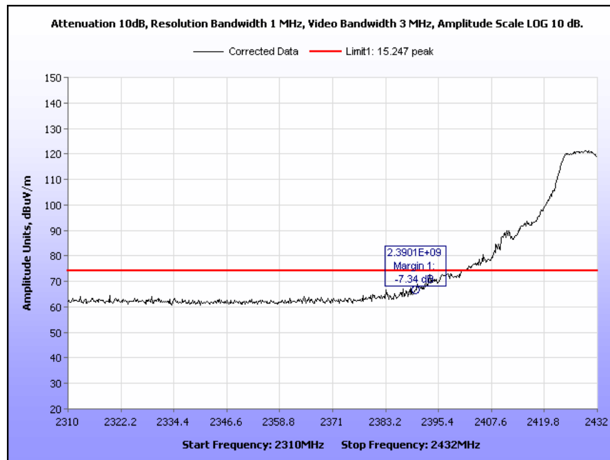
Plot 63. Radiated Restricted Band Edge, Channel 5, 2310 MHz – 2432 MHz, 802.11g, Peak
