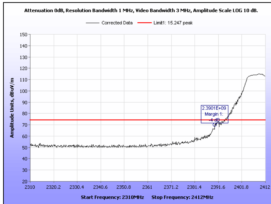
Plot 45. Radiated Restricted Band Edge, Channel 1, 2310 MHz – 2412 MHz, 802.11g, Peak
