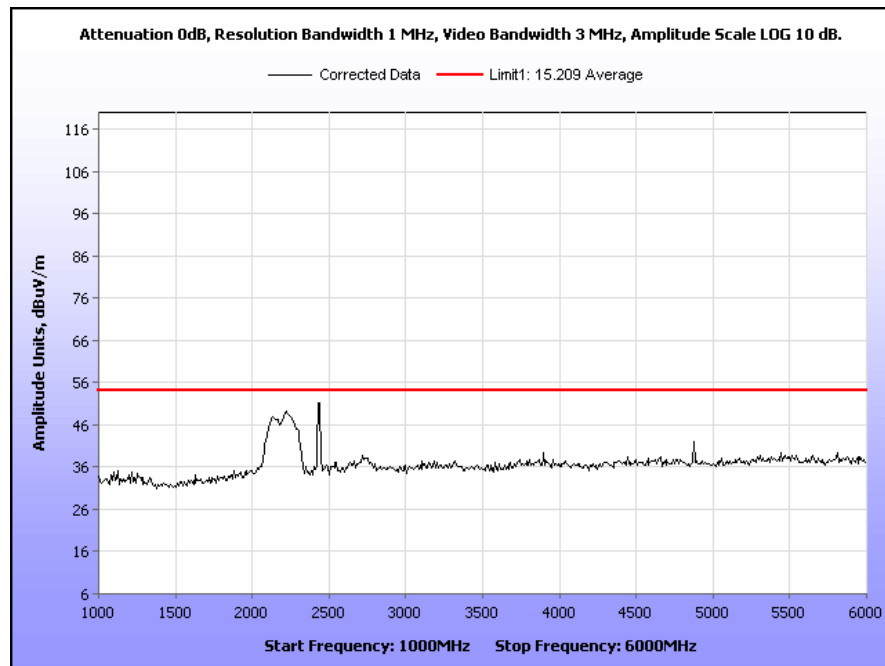
Plot 29. Radiated Spurious Emissions, Mid Channel, 802.11b, 13 dBm, 1 GHz – 6 GHz
