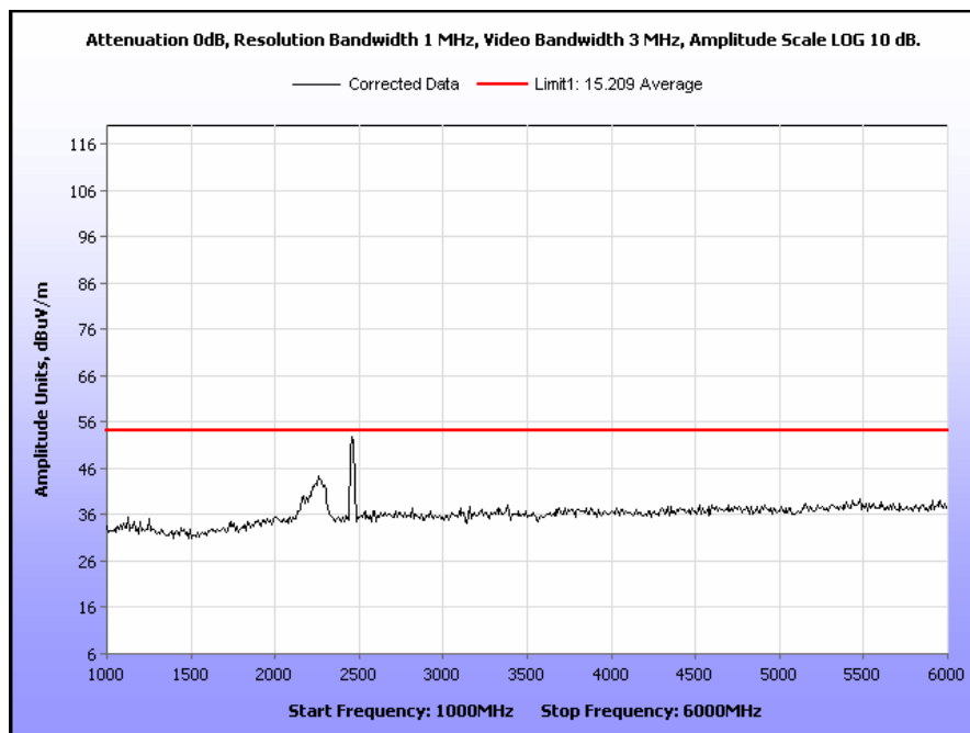
Plot 41. Radiated Spurious Emissions, High Channel, 802.11g, 9 dBm, 1 GHz – 6 GHz
