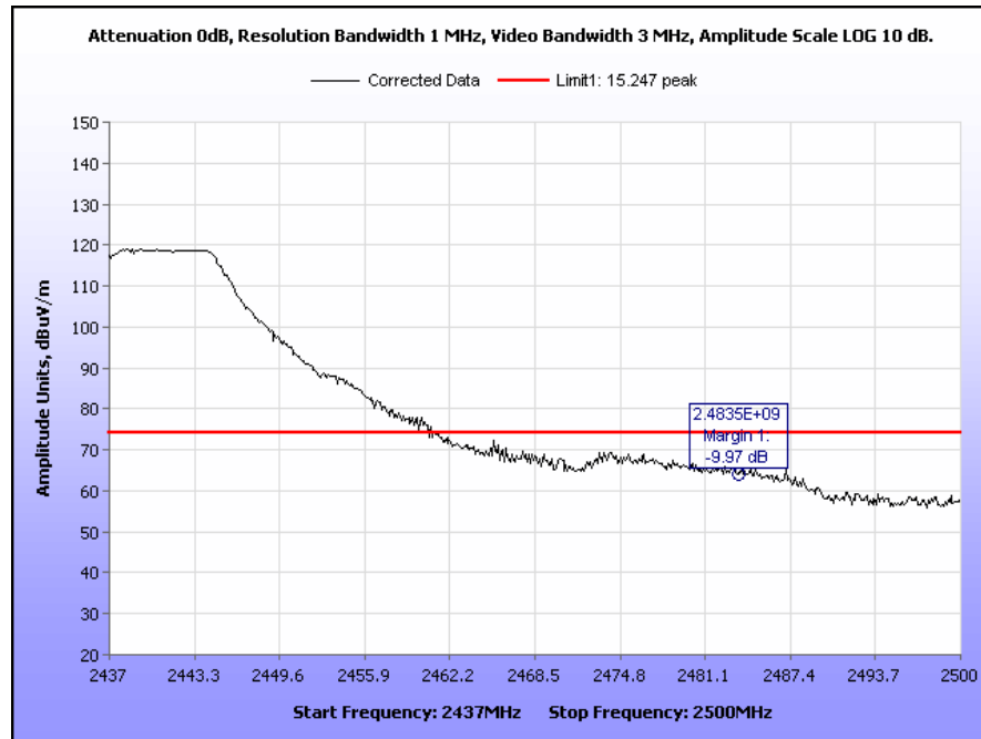
Plot 71. Radiated Restricted Band Edge, Channel 6, 2437 MHz – 2500 MHz, 802.11g, Peak
