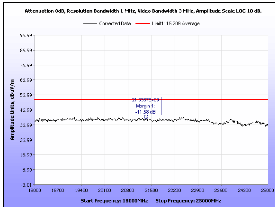
Plot 27. Radiated Spurious Emissions, Low Channel, 802.11g, 11 dBm, 18 GHz – 25 GHz
