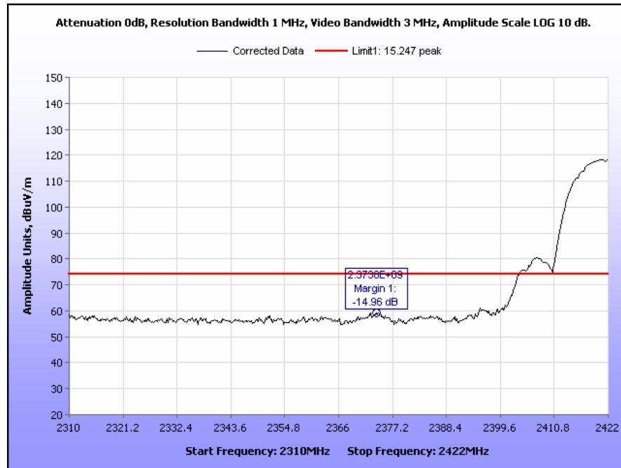
Plot 55. Radiated Restricted Band Edge, Channel 3, 2310 MHz – 2422 MHz, 802.11b, Peak
