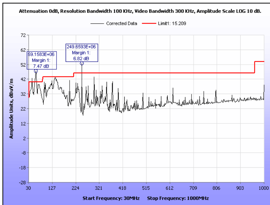
Plot 40. Radiated Spurious Emissions, High Channel, 802.11g, 9 dBm, 30 MHz – 1 GHz
