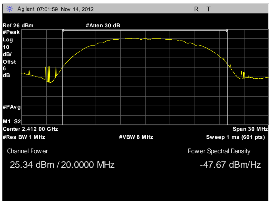
Plot 7. Peak Power Output, Channel 1, 802.11b
