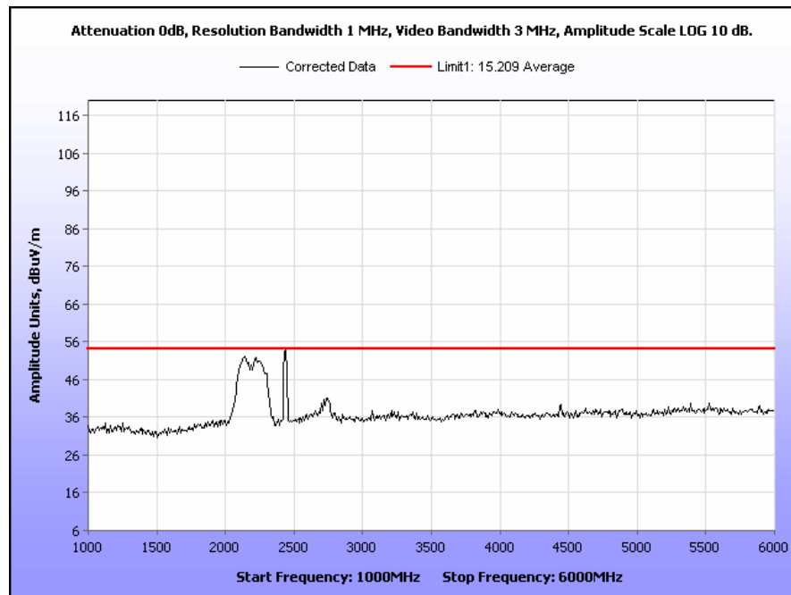
Plot 33. Radiated Spurious Emissions, Mid Channel, 802.11g, 15 dBm, 1 GHz – 6 GHz
