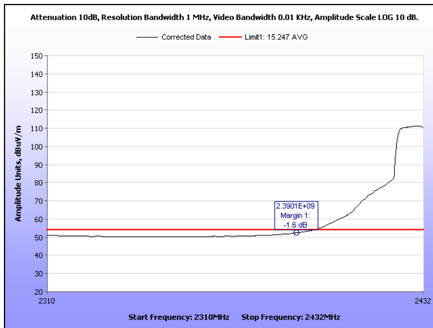
Plot 62. Radiated Restricted Band Edge, Channel 5, 2310 MHz – 2432 MHz, 802.11g, Average
