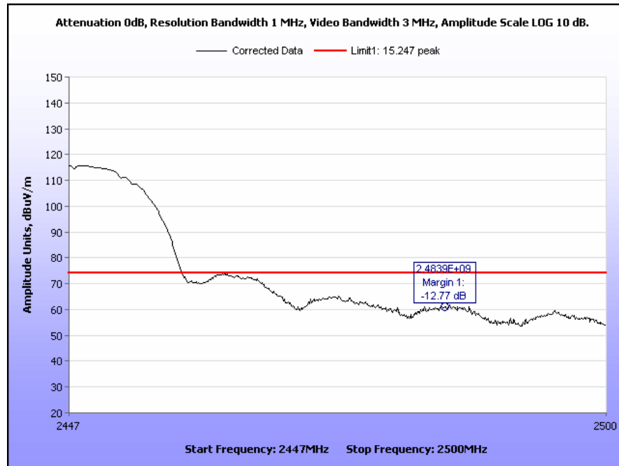
Plot 77. Radiated Restricted Band Edge, Channel 8, 2447 MHz – 2500 MHz, 802.11b, Peak
