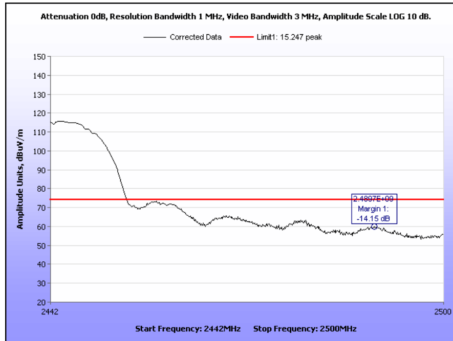
Plot 73. Radiated Restricted Band Edge, Channel 7, 2442 MHz – 2500 MHz, 802.11b, Peak
