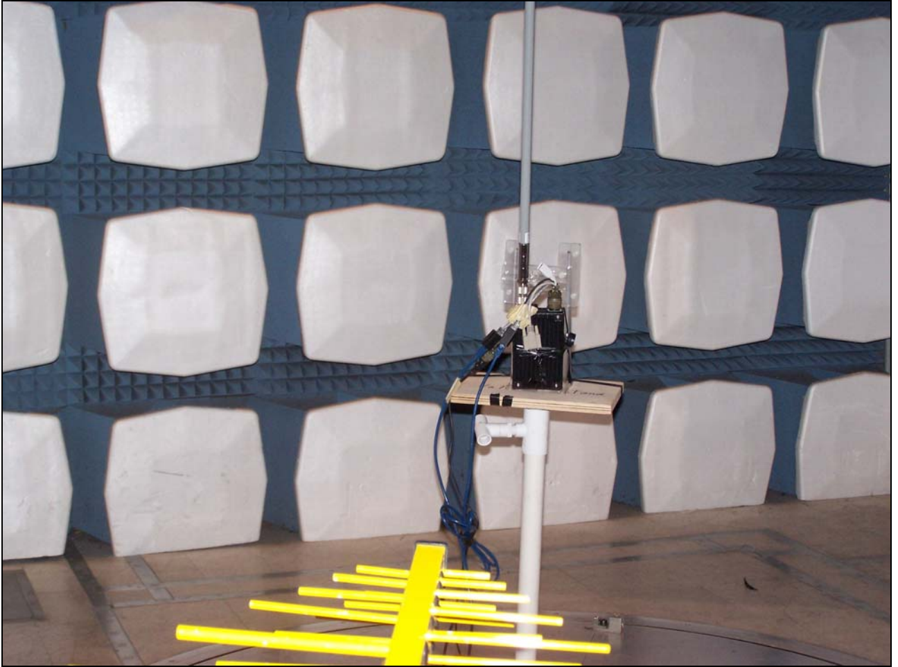
Photograph 2. Radiated Emission, Test Setup, ME3-09
