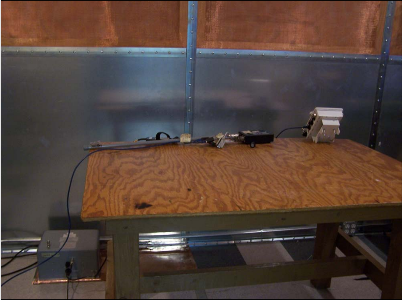
Photograph 3. Conducted Emissions, 15.207, Test Setup, ME3-09
