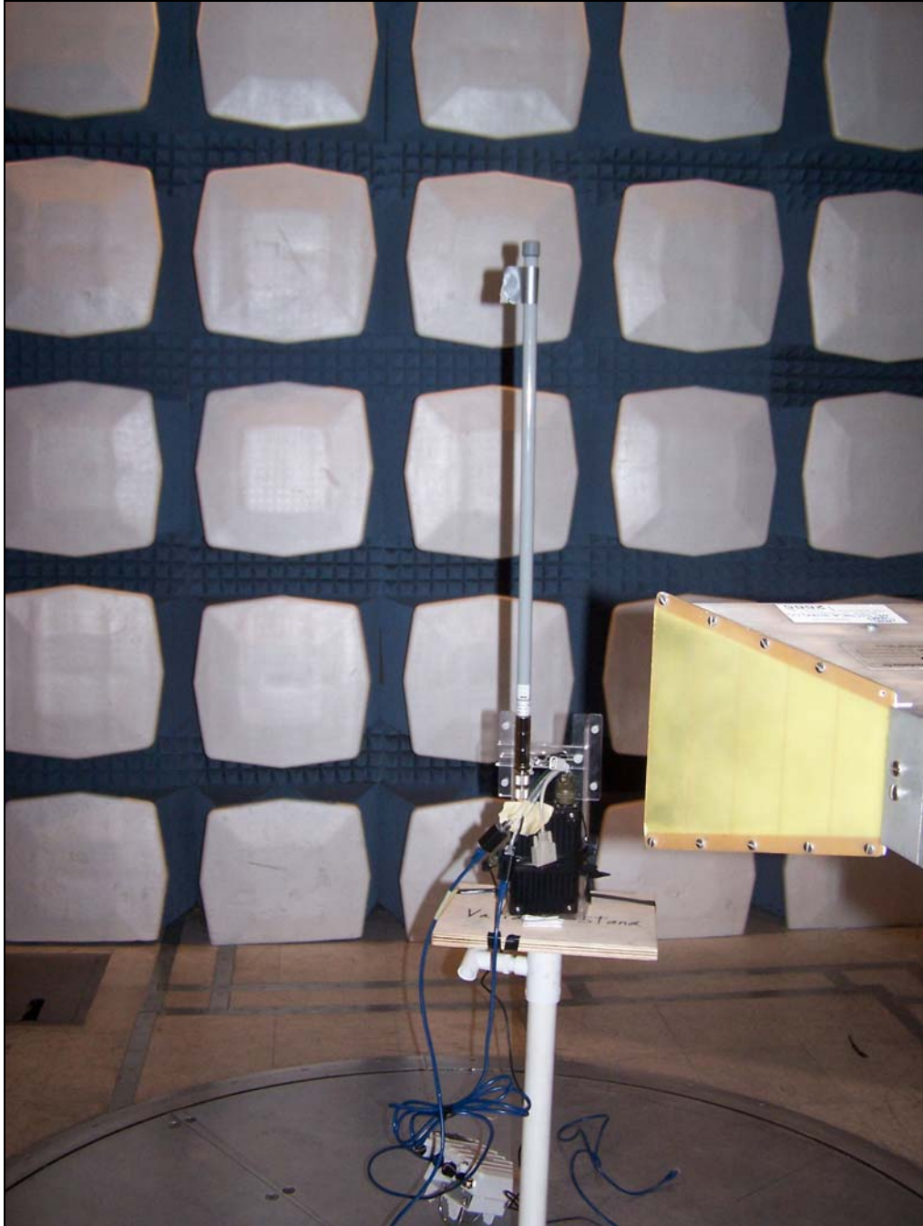
Photograph 4. Radiated Spurious Emissions, Test Setup, ME3-09
