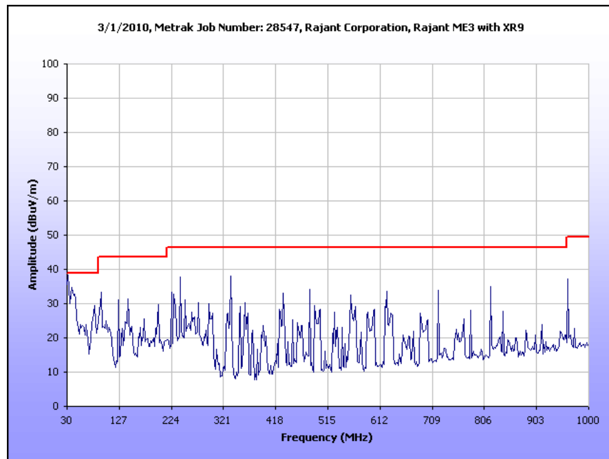
Plot 3. Radiated Emissions, 30 MHz - 1 GHz, FCC Limits, ME3-09
