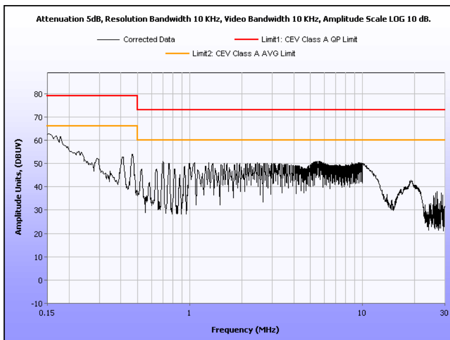
Plot 2. Conducted Emission, Neutral Line Plot, ME3-09
