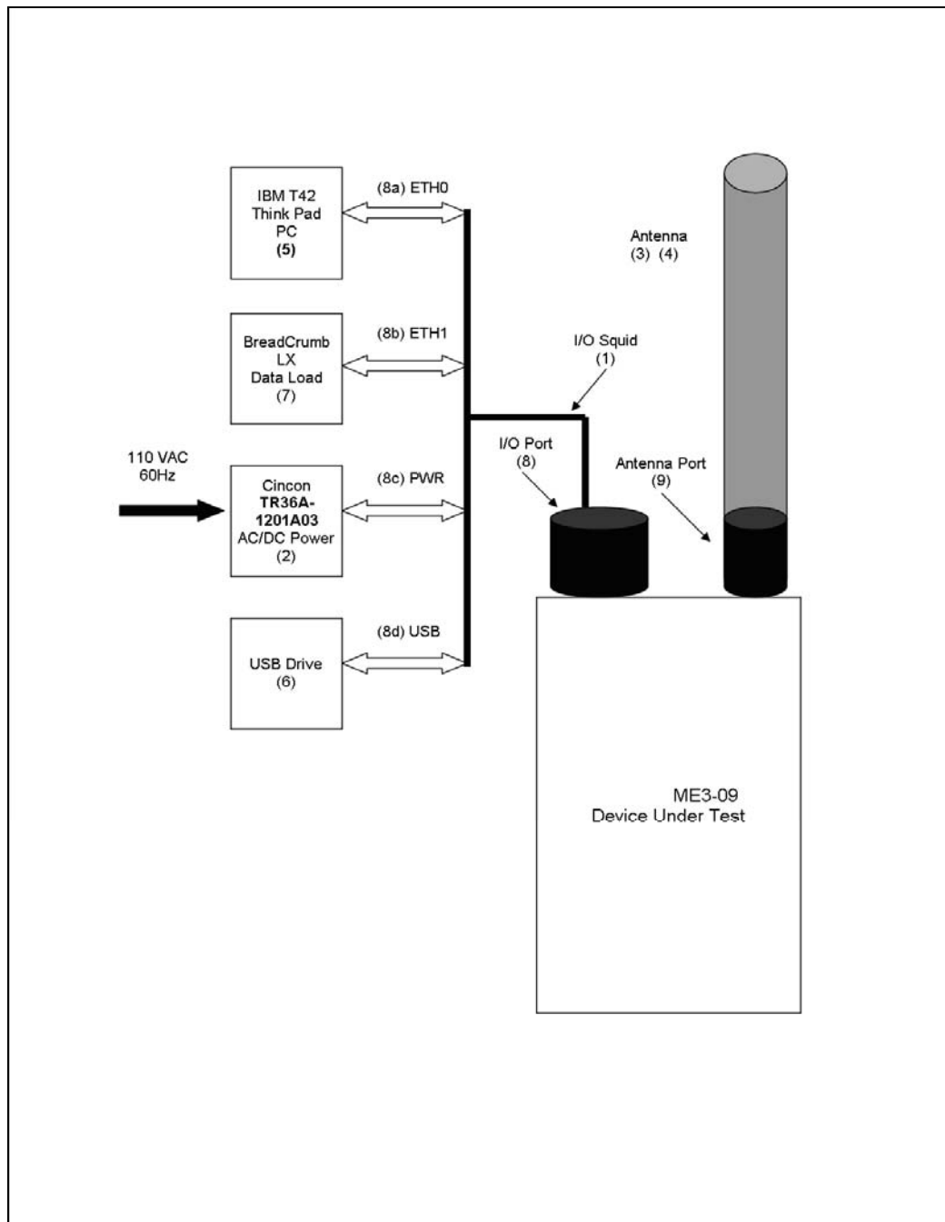
Figure 1. Block Diagram of Test Configuration
