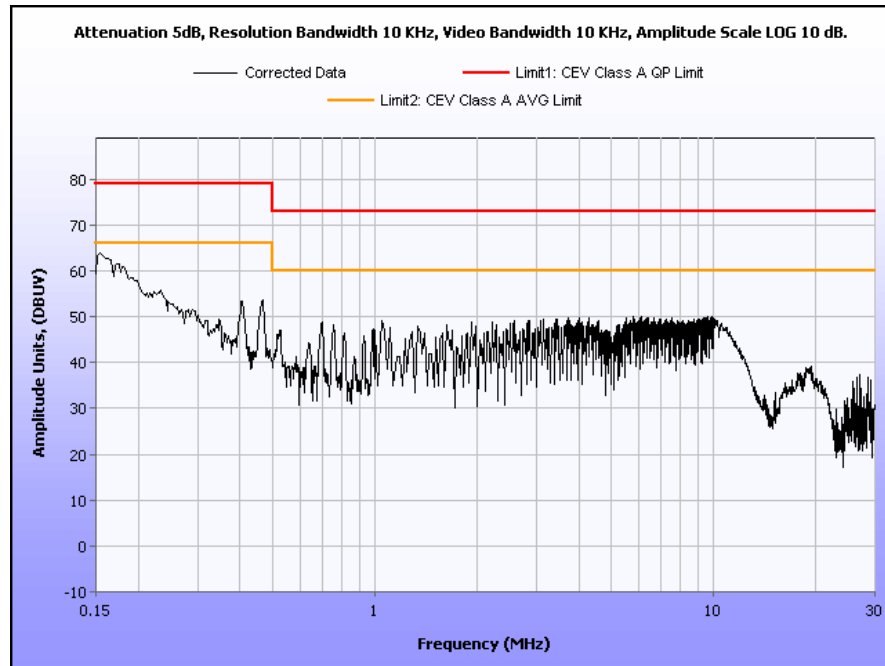
Plot 1. Conducted Emission, Phase Line Plot, ME3-09
