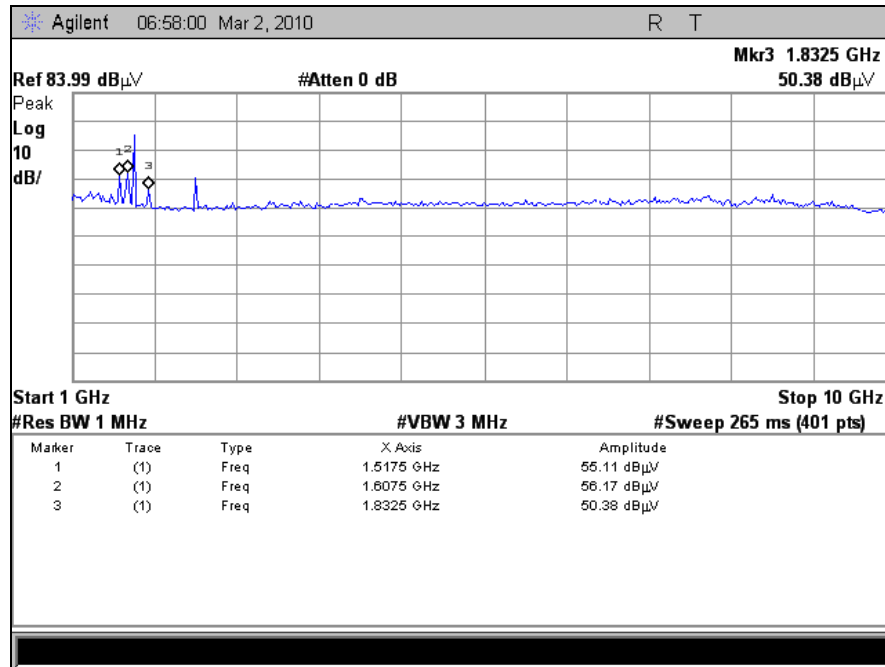
Plot 12. Radiated Spurious Emissions, 1 GHz – 10 GHz, Channel 6, b Mode, ME3-09
