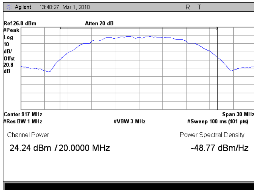
Plot 7. RF Output Power, b Mode, Channel 6, ME3-09
