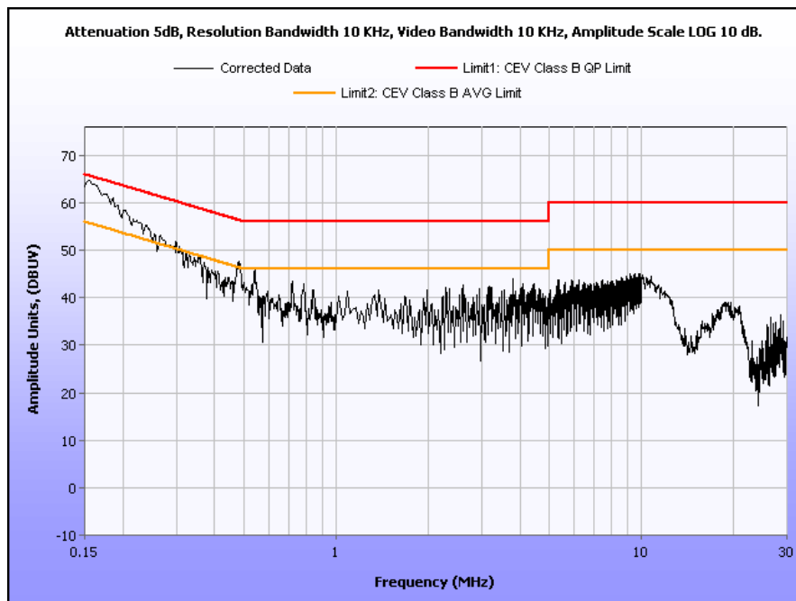
Plot 4. Conducted Emissions, Phase Line, Chanel 5, g Mode, ME3-09
