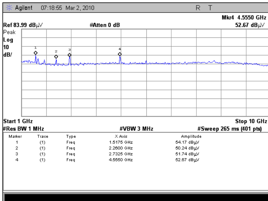
Plot 11. Radiated Spurious Emissions, 1 GHz – 10 GHz, Channel 5, g Mode, ME3-09
