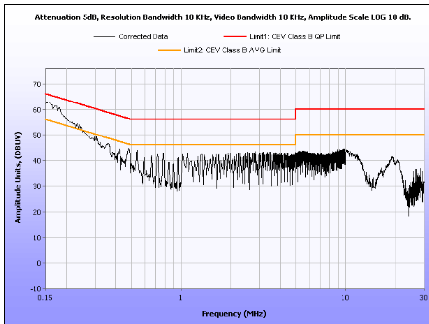
Plot 5. Conducted Emissions, Neutral Line, Chanel 5, g Mode, ME3-09
