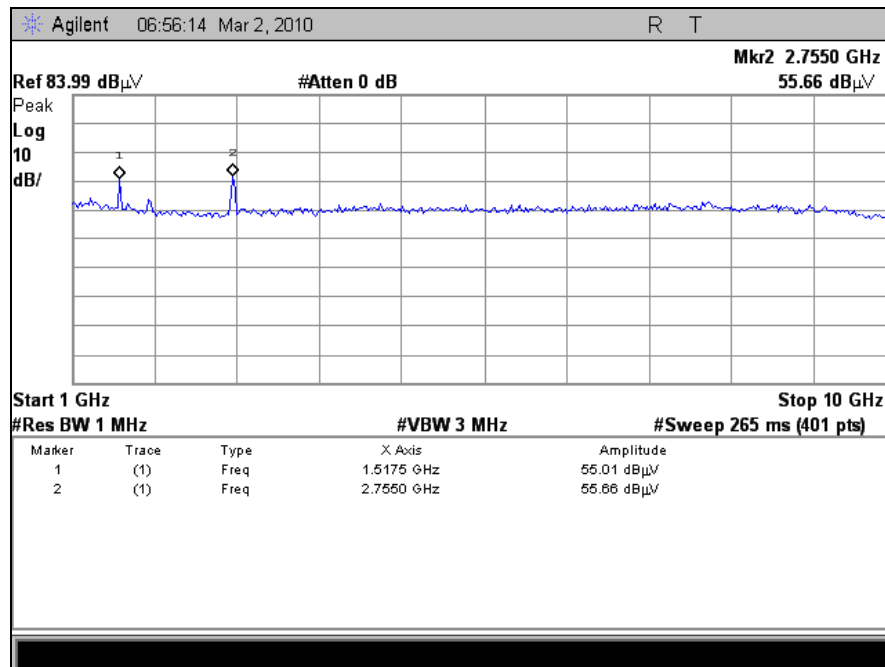
Plot 13. Radiated Spurious Emissions, 1 GHz – 10 GHz, Channel 6, g Mode, ME3-09
