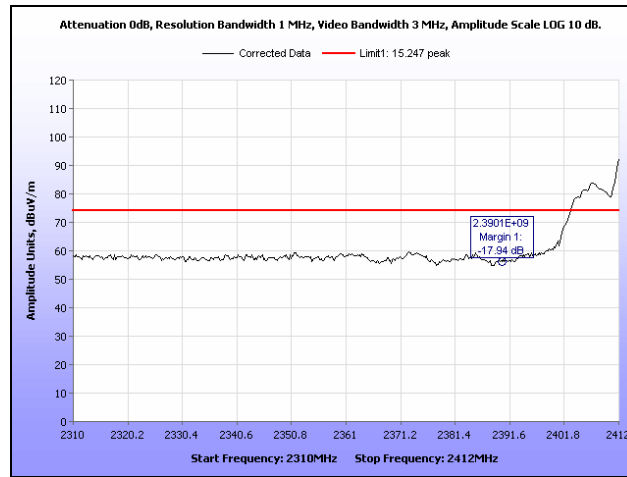
Plot 43. Radiated Restricted Band Edge, b Mode, Channel 3, Peak, 2.4 GHz
