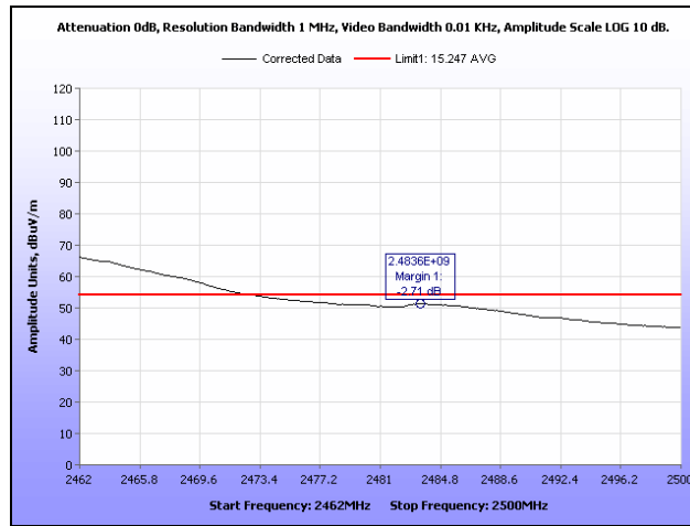
Plot 72. Radiated Restricted Band Edge, g Mode, Channel 8, Average, 2.4 GHz
