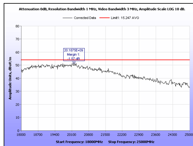
Plot 34. Radiated Spurious Emissions, High Channel, 18 GHz – 25 GHz, g Mode, 2.4 GHz
