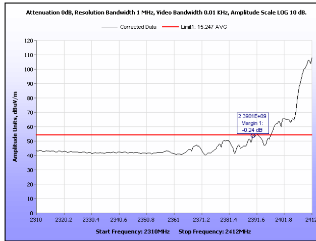
Plot 40. Radiated Restricted Band Edge, b Mode, Channel 2, Average, 2.4 GHz
