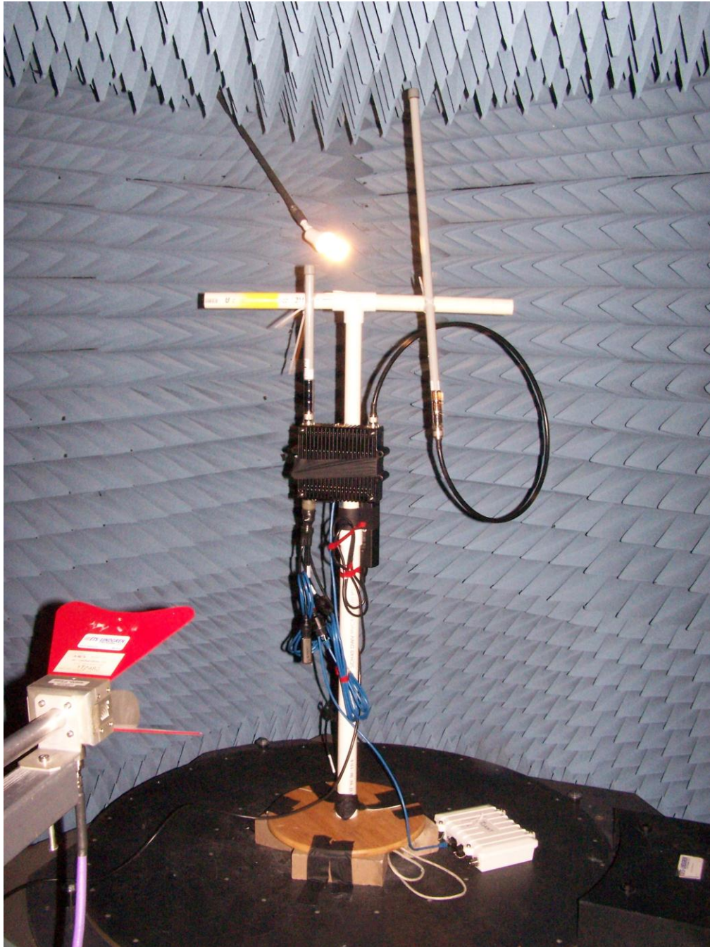
Radiated Emissions, 1 GHz – 7 GHz
