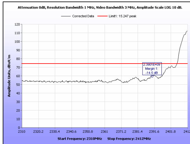
Plot 41. Radiated Restricted Band Edge, b Mode, Channel 2, Peak, 2.4 GHz
