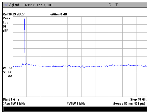
Plot 21. Radiated Spurious Emissions, Mid Channel, 1 GHz – 18 GHz, b Mode, 2.4 GHz
