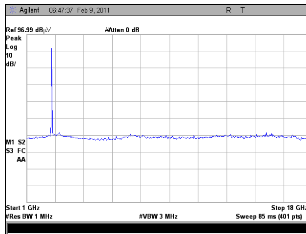
Plot 24. Radiated Spurious Emissions, High Channel, 1 GHz – 18 GHz, b Mode, 2.4 GHz
