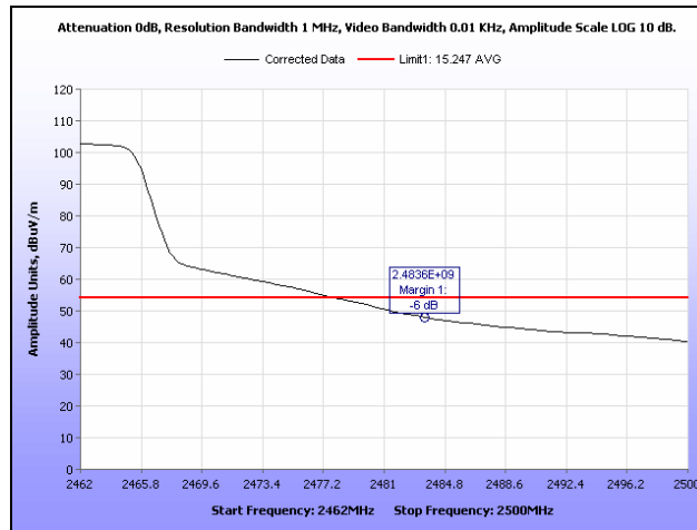
Plot 76. Radiated Restricted Band Edge, g Mode, Channel 10, Average, 2.4 GHz
