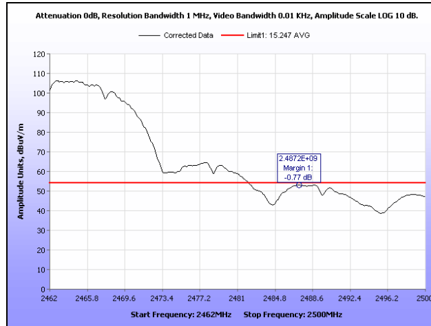
Plot 58. Radiated Restricted Band Edge, b Mode, Channel 11, Average, 2.4 GHz
