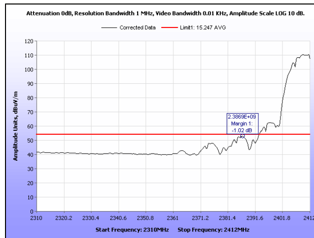
Plot 38. Radiated Restricted Band Edge, b Mode, Channel 1, Average, 2.4 GHz
