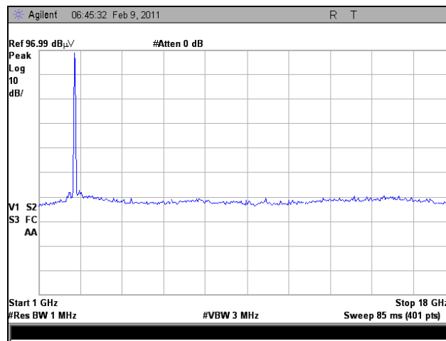
Plot 30. Radiated Spurious Emissions, Mid Channel, 1 GHz – 18 GHz, g Mode, 2.4 GHz
