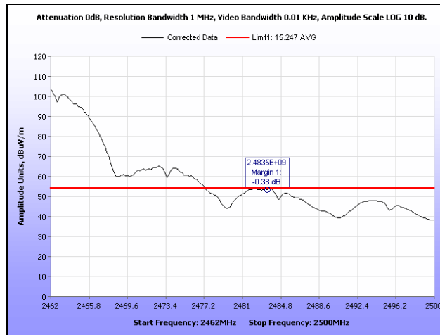
Plot 56. Radiated Restricted Band Edge, b Mode, Channel 10, Average, 2.4 GHz
