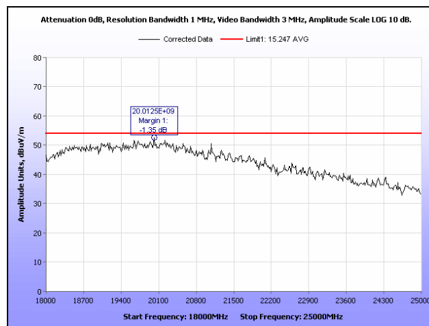
Plot 28. Radiated Spurious Emissions, Low Channel, 18 GHz – 25 GHz, g Mode, 2.4 GHz
