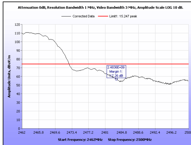
Plot 59. Radiated Restricted Band Edge, b Mode, Channel 11, Peak, 2.4 GHz
