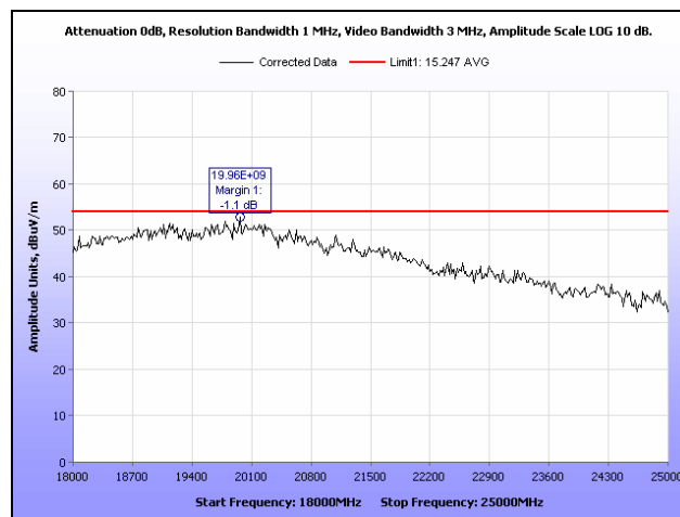
Plot 25. Radiated Spurious Emissions, High Channel, 18 GHz – 25 GHz, b Mode, 2.4 GHz
