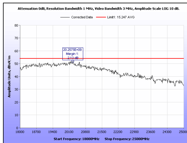
Plot 22. Radiated Spurious Emissions, Mid Channel, 18 GHz – 25 GHz, b Mode, 2.4 GHz
