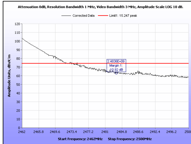
Plot 75. Radiated Restricted Band Edge, g Mode, Channel 9, Peak, 2.4 GHz
