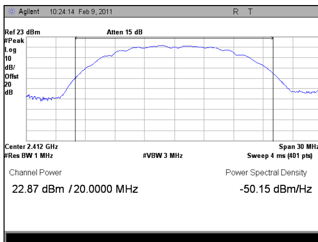
Plot 8. Peak Power Output, b Mode, Channel 1, 2.4 GHz
