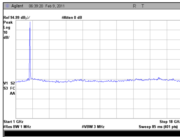
Plot 27. Radiated Spurious Emissions, Low Channel, 1 GHz – 18 GHz, g Mode, 2.4 GHz
