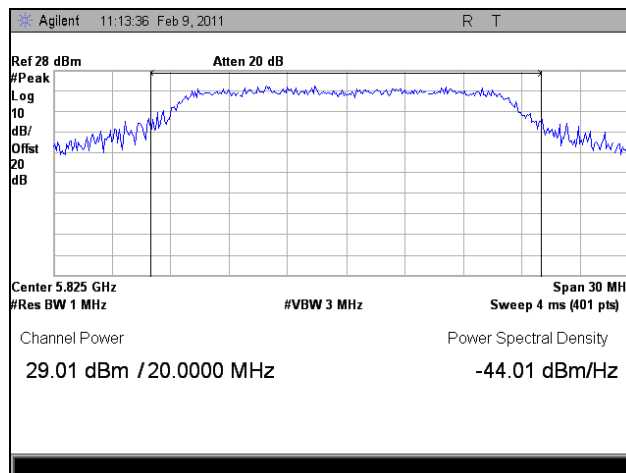
Plot 16. Peak Power Output, Channel 165, 5.8 GHz
