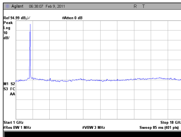
Plot 18. Radiated Spurious Emissions, Low Channel, 1 GHz – 18 GHz, b Mode, 2.4 GHz
