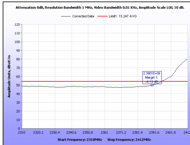
Plot 64. Radiated Restricted Band Edge, g Mode, Channel 3, Average, 2.4 GHz
