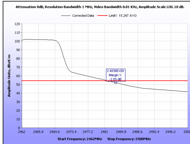
Plot 78. Radiated Restricted Band Edge, g Mode, Channel 11, Average, 2.4 GHz
