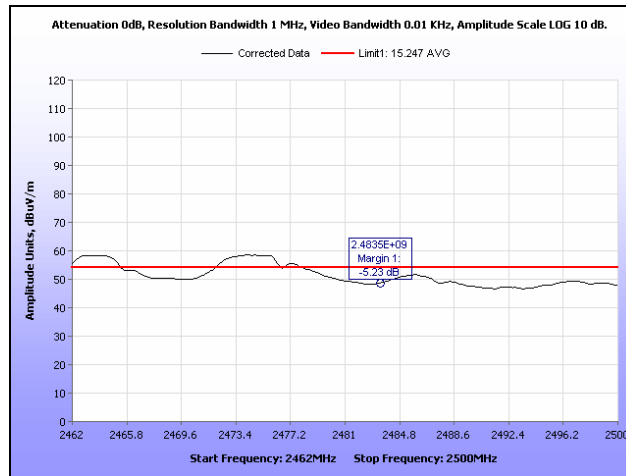
Plot 44. Radiated Restricted Band Edge, b Mode, Channel 4, Average, High End, 2.4 GHz
