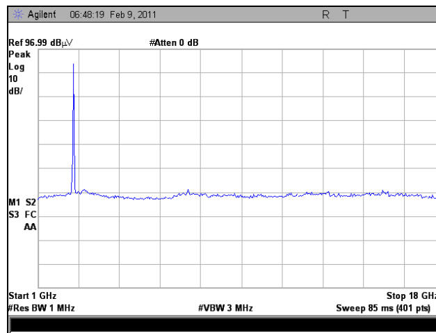
Plot 33. Radiated Spurious Emissions, High Channel, 1 GHz – 18 GHz, g Mode, 2.4 GHz
