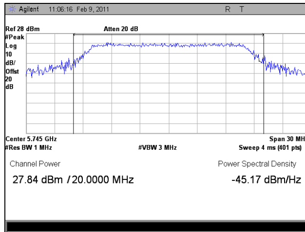
Plot 14. Peak Power Output, Channel 149, 5.8 GHz
