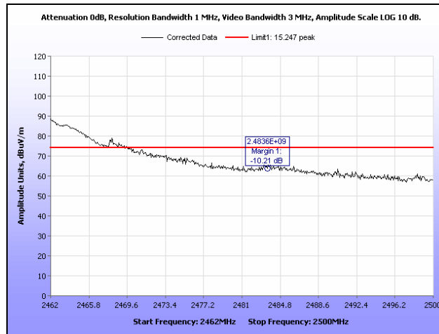
Plot 73. Radiated Restricted Band Edge, g Mode, Channel 8, Peak, 2.4 GHz
