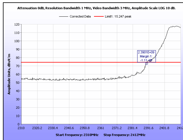
Plot 61. Radiated Restricted Band Edge, g Mode, Channel 1, Peak, 2.4 GHz
