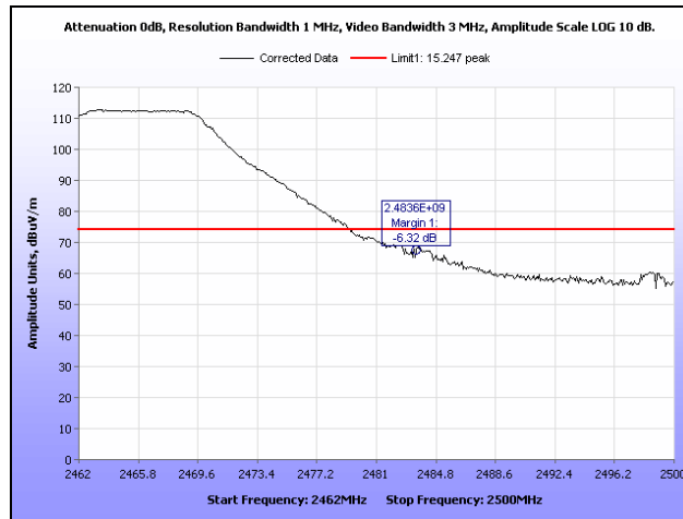
Plot 79. Radiated Restricted Band Edge, g Mode, Channel 11, Peak, 2.4 GHz
