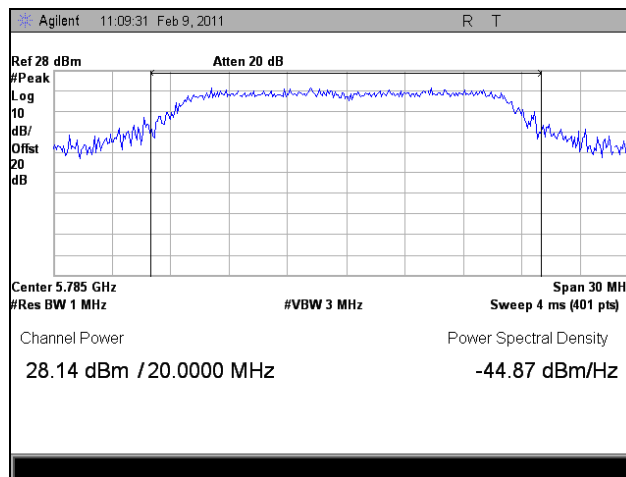
Plot 15. Peak Power Output, Channel 157, 5.8 GHz
