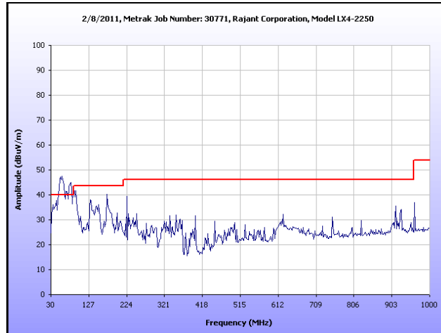
Plot 32. Radiated Spurious Emissions, High Channel, 30 MHz – 1 GHz, g Mode, 2.4 GHz
