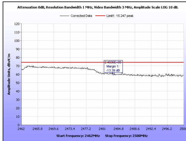
Plot 67. Radiated Restricted Band Edge, g Mode, Channel 4, Peak, High End, 2.4 GHz
