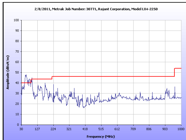
Plot 37. Radiated Spurious Emissions, High Channel, 30 MHz – 1 GHz, a Mode, 5.8 GHz
