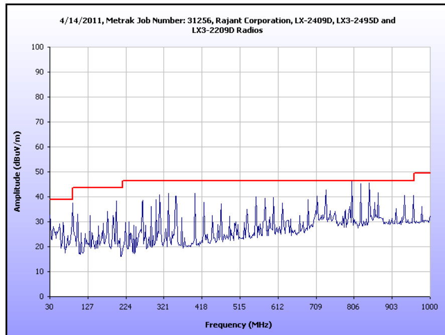
Plot 4. Radiated Emissions, 30 MHz - 1 GHz, FCC Limits, AC PoE
