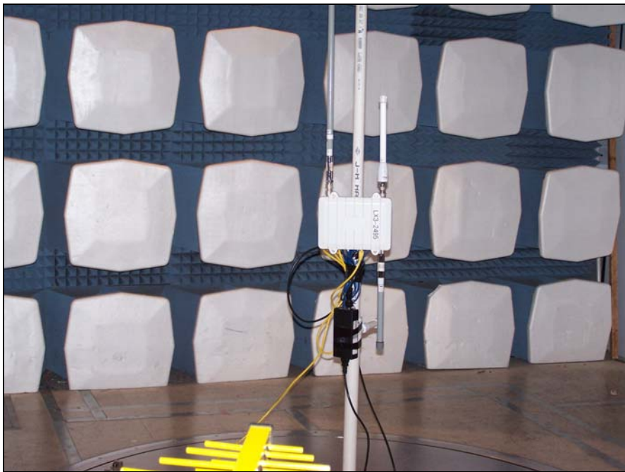
Photograph 4. Radiated Emission, Test Setup 30 MHz – 1 GHz (Models 2495 and 2209)
