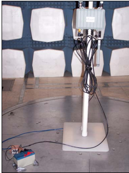
Photograph 5. Radiated Emission, Test Setup 30 MHz – 1 GHz, DC POE (Model LX3-2250)
