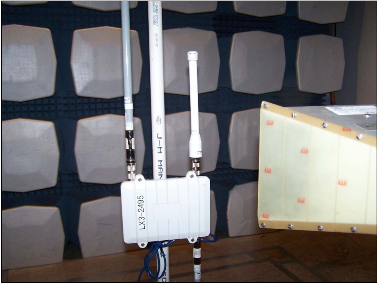
Photograph 9. Test Equipment and setup for various Radiated Measurements
